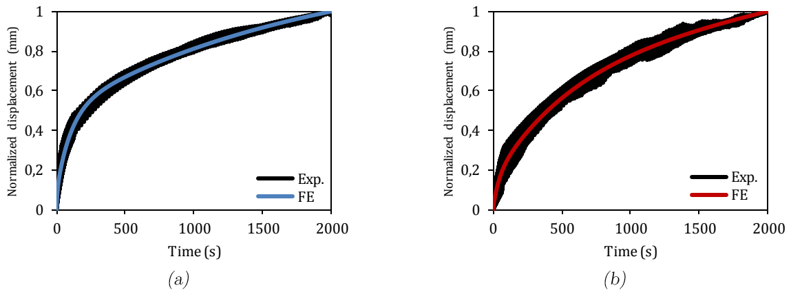
Figure VI.20: Validation of the selected viscous parameters ( n_0 ) and ( n_c ): normalized FE displacements versus normalized experimental displacements for the BM1822 (a) and for the SP498 (b) adhesives.
