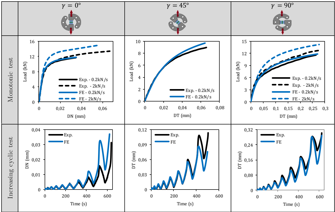
Figure VI.31: Comparison between FE predictions and experimental results for the Betamate-1822 adhesive.
