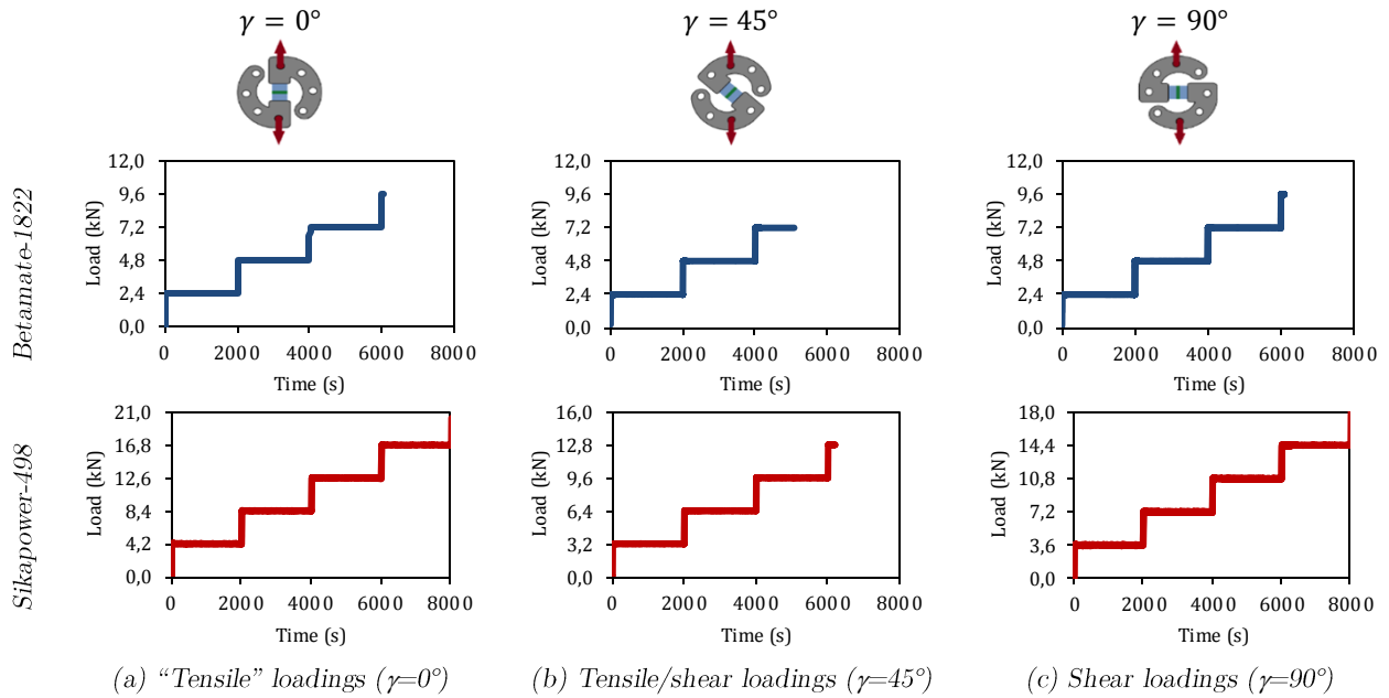
Figure V.12: Imposed load for the multilevel creep tests.
