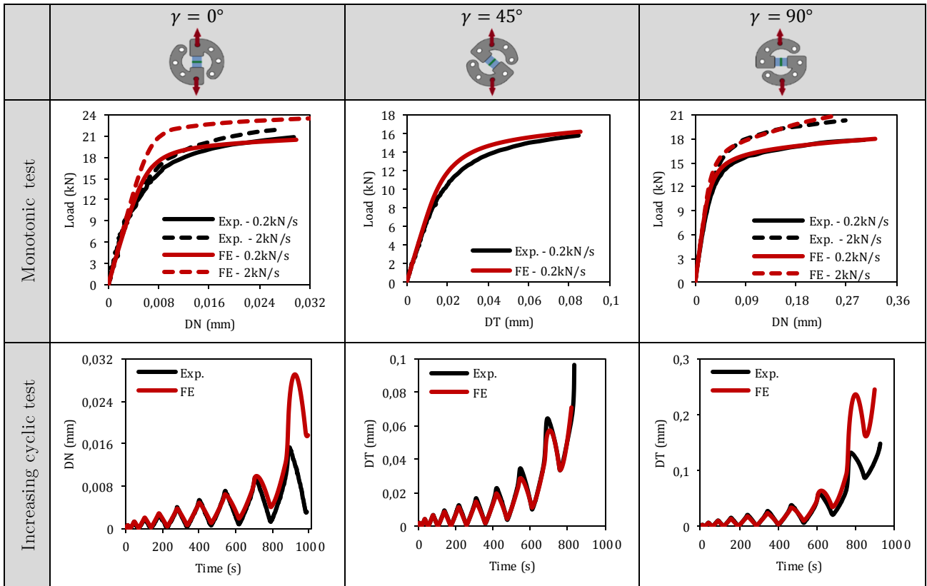
Figure VI.32: Comparison between FE predictions and experimental results for the Sikapower-498 adhesive.
