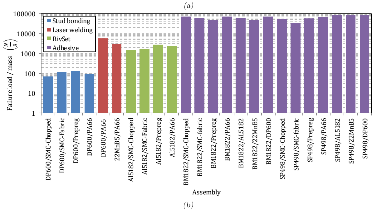
Figure IV.10: Comparison of the joining techniques as a function of the failure load and the additional mass in shear (a) and “tensile” loadings (b).
