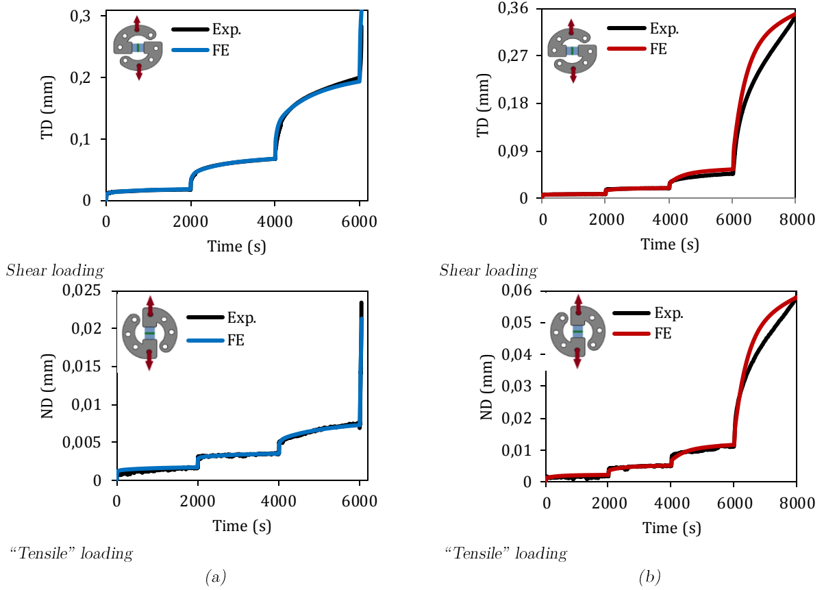
Figure VI.27: Numerical prediction versus experimental results of the multilevel creep tests for the Betamate-1822 (a) and Sikapower-498 (b) adhesives.
