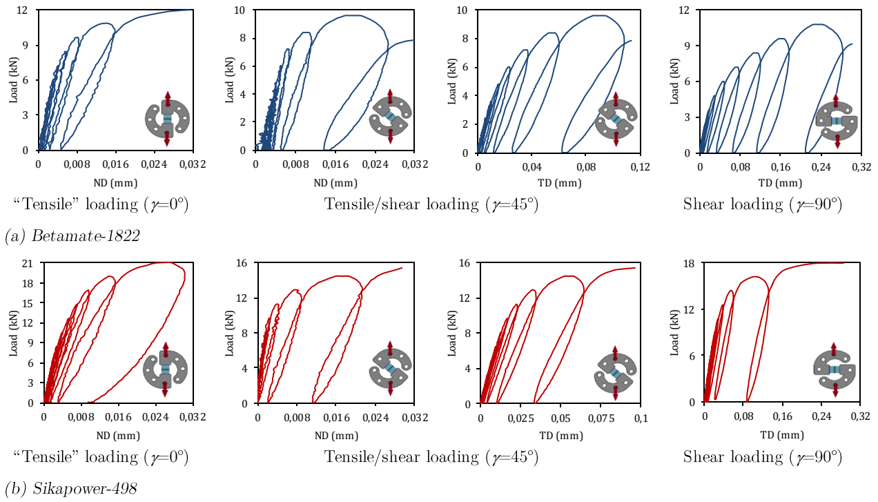
Figure V.21: Overview of the behavior of the adhesives in increasing cyclic tests. Only one single specimen has been plotted for each case.
