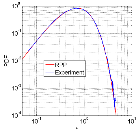
Figure 7.11: Probability density function of the Voronoï areas for the bubbles (blue line) and for a random Poisson process (red, obtained according to equation (7.9)).
