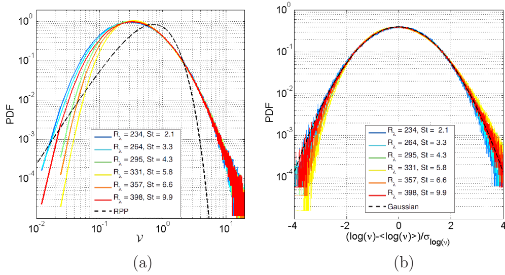
Figure 9.4: (a) Probability distribution of normalized Voronoï area \mathcal{V} for experiments at different Reynolds number and Stokes number. (b) Probability distribution function, centered and reduced, of \log(\mathcal{V}) .
