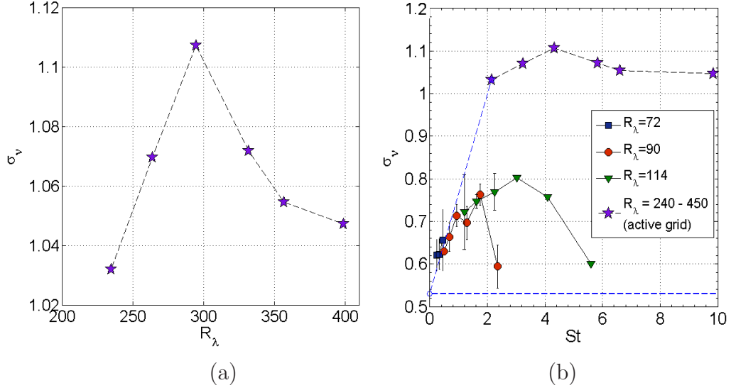
Figure 9.5: (a) Evolution of the standard deviation of the normalized Voronoï area with Reynolds number. (b) Evolution of the standard deviation of the normalized Voronoï area with Stokes number. We have also reported previous measurements at lower Reynolds number, with the passive grid, by Monchaux et al. [68]. We have also manually added the point (St = 0, \sigma_V = 0.53) .
