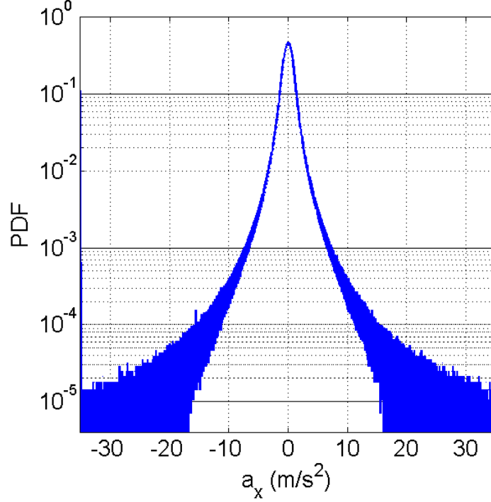
Figure 9.10: Histogram of the acceleration a_x of the flow obtained with DNS. The other components give similar result.
