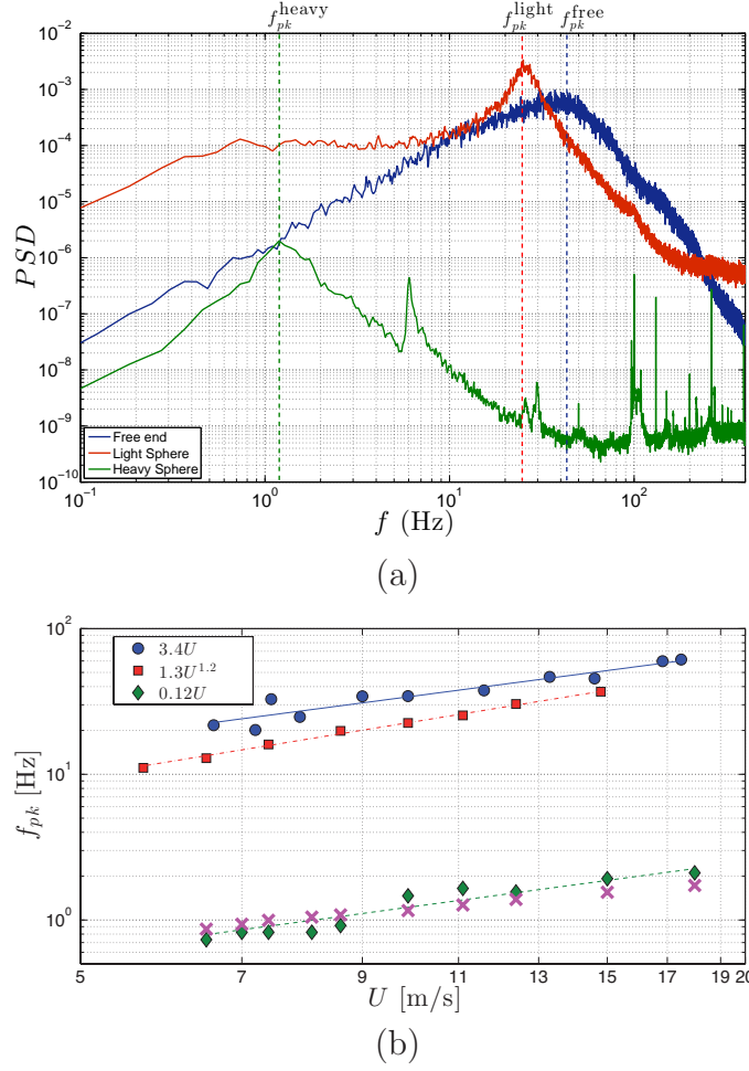
Figure 5.9: (a) Comparison of the spectral densities for the three towed configurations (free end, light particle and heavy particle) at a given towing velocity U \simeq 11 m/s. (b) Dependency of the peak frequency on mean towing velocity U for the three configurations : free end (blue circles), polystyrene sphere (red squares) and lead sphere (green diamond). The lines indicate the best power law fit, whose parameters are given in the legend (note that linear fit indeed correspond to a power law fit for which the best fitting exponent was found to be almost 1). Magenta crosses indicate the estimation of the peak frequency for the heavy lead particle based on a simple pendular model discussed in section 5.3.4.
