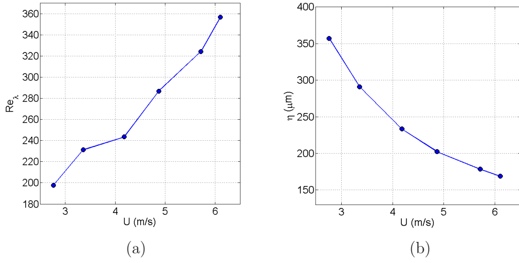
Figure 2.8: Reynolds number based on the Taylor microscale (a) and Kolmogorov length scale (b) obtained for the active grid for different streamwise velocities at x = 3.0 m.
