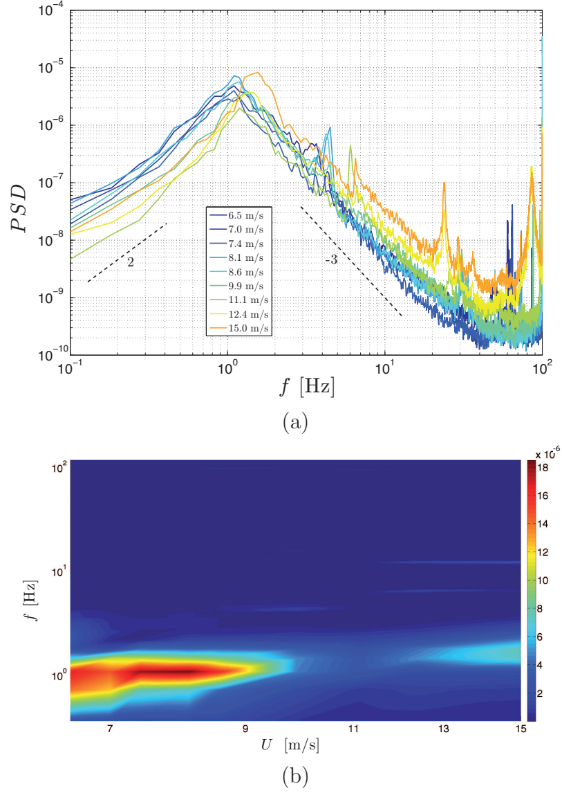
Figure 5.8: (a) Power Spectral Density of the velocity fluctuations for the heavy sphere at different towing speeds (only the horizontal component is showed). (b) Interpolated representation of the previous PSDs in the velocity - frequency ( U - f ) plane. The color codes the amplitude of the spectra.
