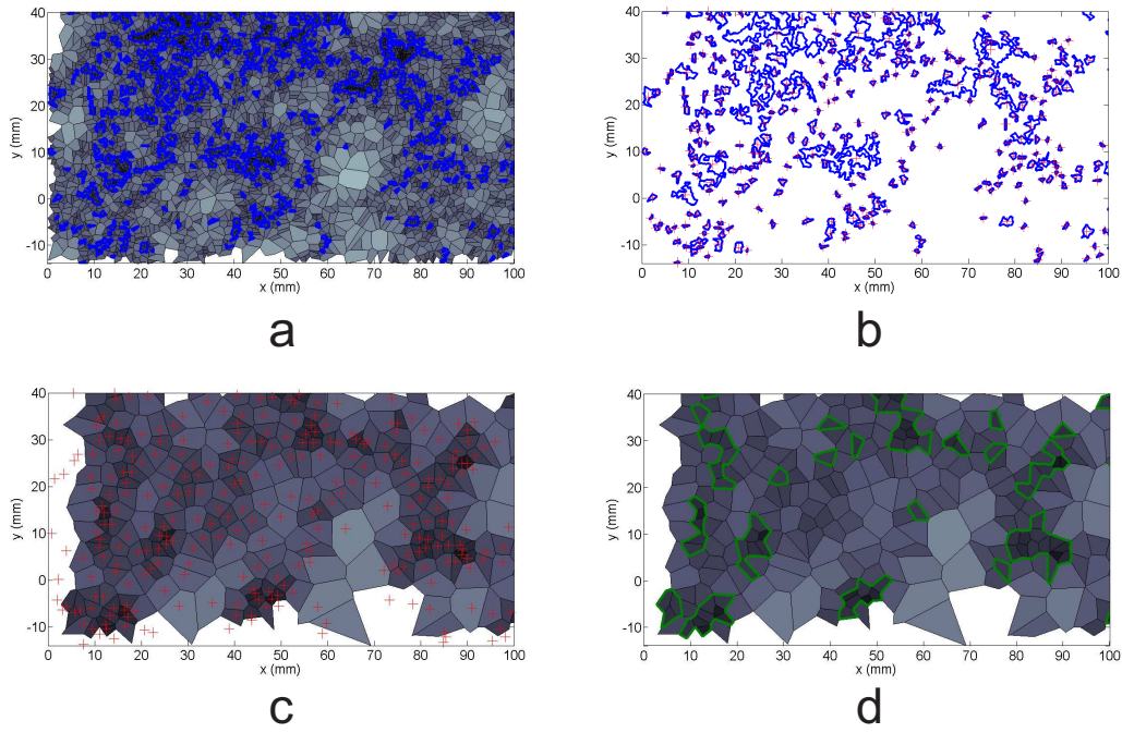
Figure 9.17: Procedure for obtaining superclusters. (a) Clusters are identified from the Voronoï cells obtained from raw images. (b) The centers of clusters are identified as the average of local densities (i.e. the inverse of Voronoï cells area). (c) Voronoï tessellations of clusters centers are computed. (d) Clusters of clusters are identified. Only a section with 5 \text{ cm}^2 of images is represented for properly identifying Voronoï diagrams.
