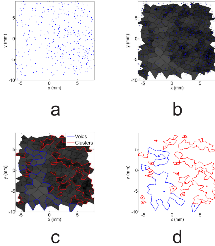
Figure 8.6: Schema of clusters and voids detection. Starting from particle's centers in real space (a), the Voronoï diagrams are obtained (b). With the method explained above, clusters and voids are identified (c). In a final step, centers of mass of clusters and voids are calculated (d).
