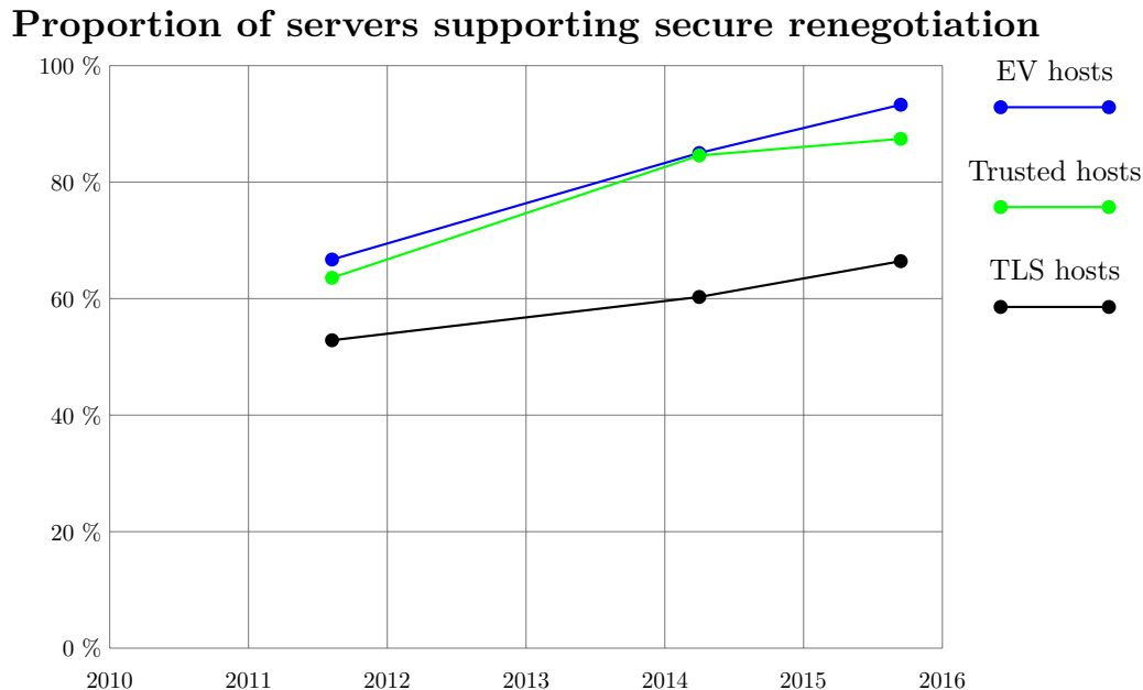
Figure 5.6: Proportion of servers supporting secure renegotiation between 2010 and 2015.
