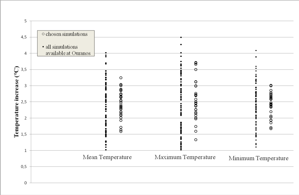
Figure S3: Differences between the mean of the future (2046-2065) and of the historical simulated temperature distributions (1971-2000) (deltas of the mean of the three temperature variables, i.e. daily mean, minimum and maximum temperatures) for the simulations chosen and for all available simulations at the Ouranos consortium on climate change (n=127 simulations for mean temperatures, n=111 for maximum and minimum temperatures).
