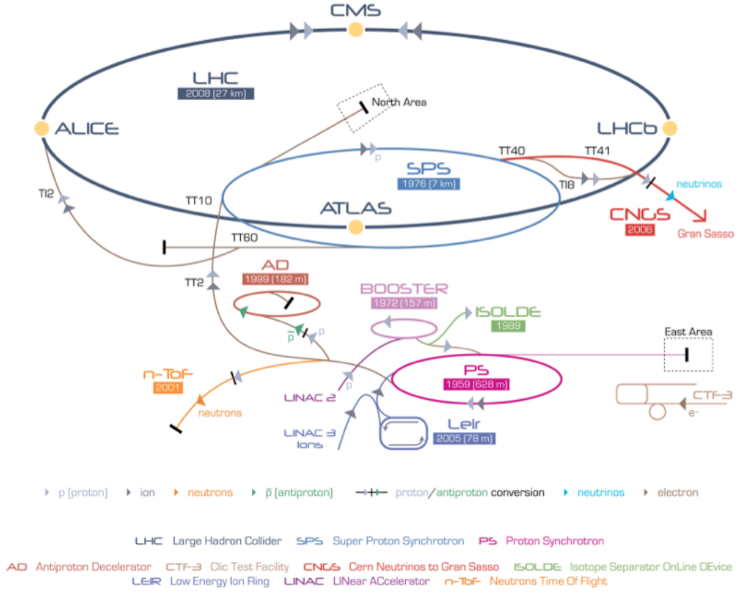
Figure 3.2: Overview of the CERN accelerator complex including the LHC.
