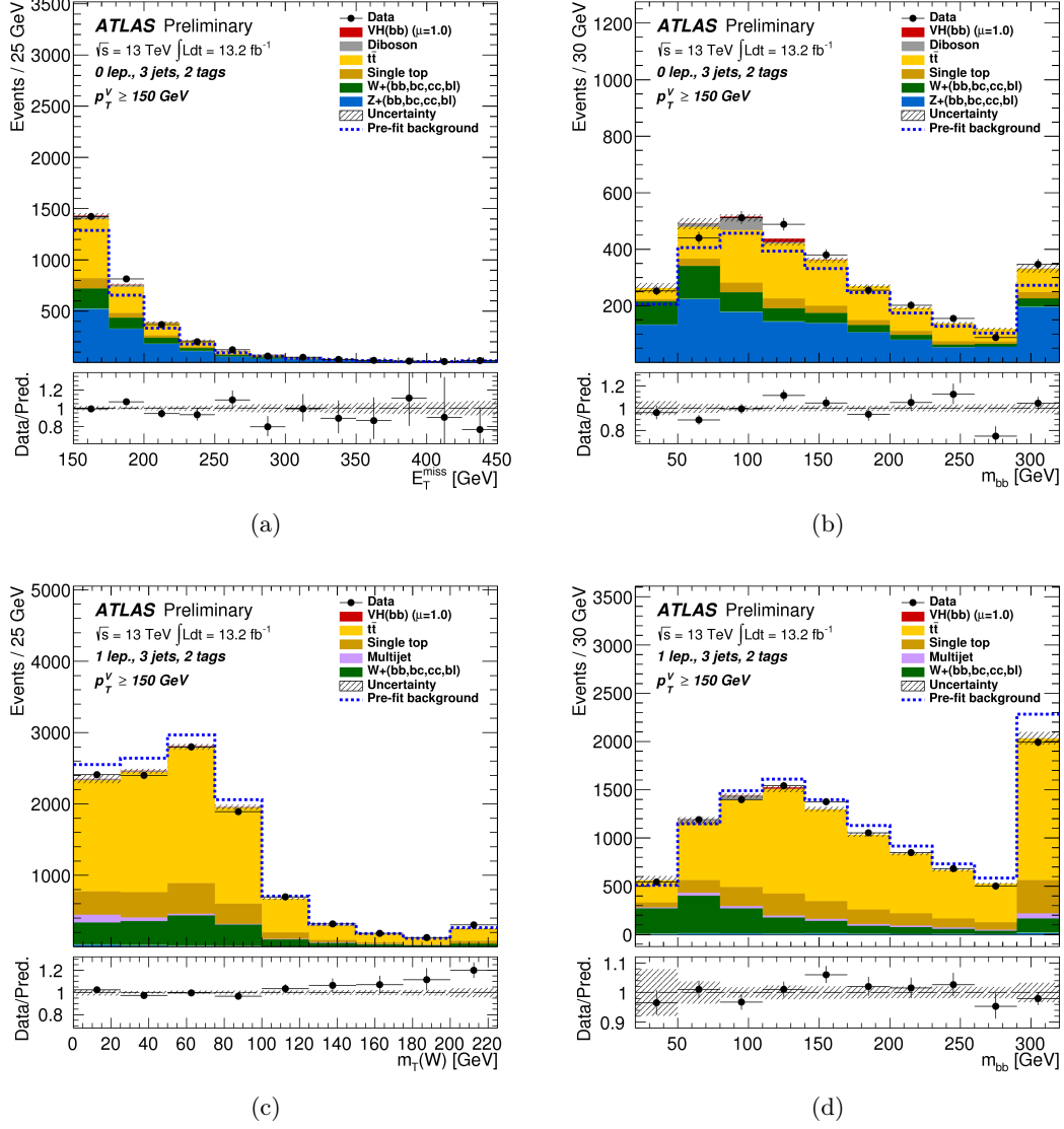
Figure 8.6: The E_T^{miss} (left) and m_{bb} (right) post-fit distributions in the 0-lepton channel for 2-tag events, in the 3-jet high p_T^V region (top). The m_W^W (left) and m_{bb} (right) post-fit distributions in the 1-lepton channel for 2-tag events, in the 3-jet high p_T^V region (bottom). The background contributions after the global likelihood fit are shown as filled histograms. The Higgs boson signal ( m_H = 125 GeV) is shown as a filled histogram on top of the fitted backgrounds as expected from the SM (indicated as \mu = 1.0 ). The dashed histogram shows the total background as expected from the pre-fit MC simulation. The size of the combined statistical and systematic uncertainty on the sum of the signal and fitted background is indicated by the hatched band. The ratio of the data to the sum of the signal and fitted background is shown in the lower panel.
