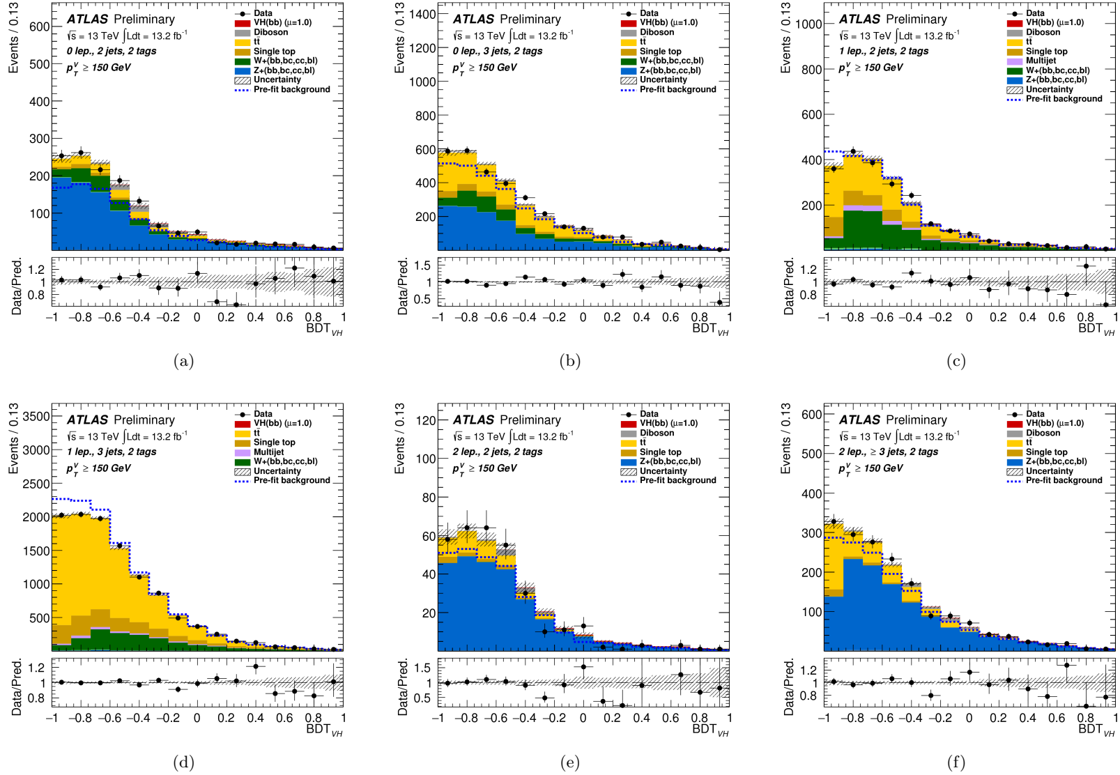
Figure 8.10: The BDT_{VH} post-fit distributions in the 0-lepton (top) 1-lepton (middle) and 2-lepton (bottom) channel for 2-tag events, in the 2-jet (left) and exactly 3 or \geq 3 -jets for the 2-lepton case (right) categories in the high p_T^V region. The background contributions after the global likelihood fit are shown as filled histograms. The Higgs boson signal ( m_H = 125 GeV) is shown as a filled histogram on top of the fitted backgrounds as expected from the SM (indicated as \mu = 1.0 ). The dashed histogram shows the total background as expected from the pre-fit MC simulation. The size of the combined statistical and systematic uncertainty on the sum of the signal and fitted background is indicated by the hatched band. The ratio of the data to the sum of the signal and fitted background is shown in the lower panel.
