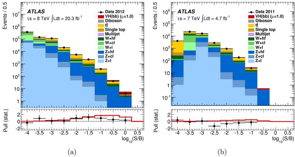
Figure 6.33: Event yields as a function of \log(S/B) for data, background and Higgs boson signal with m_H = 125 \text{ GeV} for the (a) 8 TeV data and (b) 7 TeV data. Final-discriminant bins in all signal regions are combined into bins of \log(S/B) . The signal S and background B yields are expected and fitted, respectively. The Higgs boson signal contribution is shown as expected for the SM cross section (indicated as \mu=1.0 ). The pull of the data with respect to the background-only prediction is also shown with statistical uncertainties only. The full line indicates the pull of the prediction for signal ( \mu=1.0 ) and background with respect to the background-only prediction.
