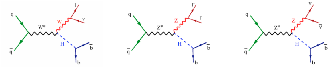
Figure 2.14: Feynman diagrams for the three leptonic decay channels of VH(b\bar{b}) .
