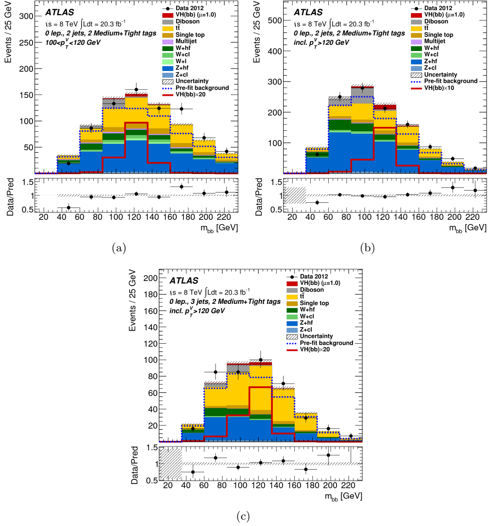
Figure 6.15: The dijet-mass distribution observed in data (points with error bars) and expected (histograms) in the 0-lepton channel with the Medium and Tight b-tagging categories (also referred to as MM and TT in the text) combined for (a) the 2-jet signal region in the 100 < p_T^V < 120 GeV interval, (b) the 2-jet signal regions in the three intervals with p_T^V > 120 GeV combined, and (c) the 3-jet signal regions in the three intervals with p_T^V > 120 GeV combined. The background contributions after the global fit of the dijet-mass analysis are shown as filled histograms. The Higgs boson signal ( m_H = 125 GeV) is shown as a filled histogram on top of the fitted backgrounds, as expected from the SM (indicated as \mu = 1.0 ), and, unstacked as an unfilled histogram, scaled by the factor indicated in the legend. The dashed histogram shows the total background as expected from the pre-fit MC simulation. The entries in overflow are included in the last bin. The size of the combined statistical and systematic uncertainty on the sum of the signal and fitted background is indicated by the hatched band. The ratio of the data to the sum of the signal and fitted background is shown in the lower panel.
