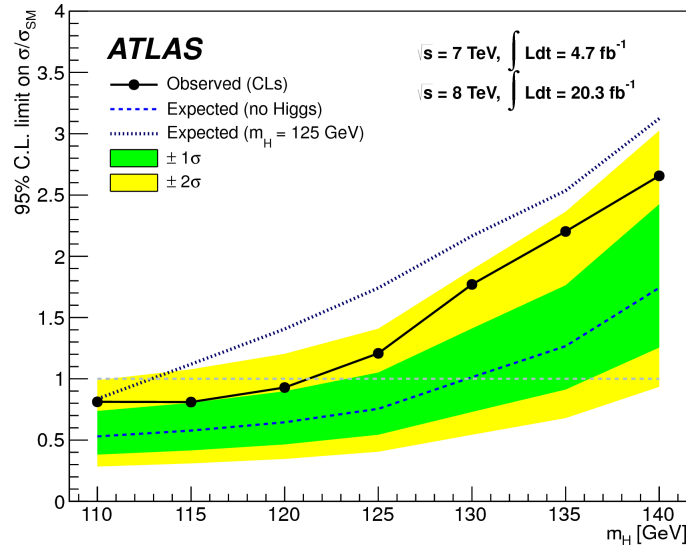
Figure 6.28: Observed (solid) and expected 95% CL cross-section upper limits, normalised to the SM Higgs boson production cross section, as a function of m_H for all channels and data-taking periods combined, as obtained using the dijet-mass analysis for the 7 TeV dataset and BDTs trained at each individual mass for the 8 TeV dataset. The expected upper limit is given for the background-only hypothesis (dashed) and with the injection of a SM Higgs boson signal at a mass of 125 GeV (dotted). The dark and light shaded bands represent the 1\sigma and 2\sigma ranges of the expectation in the absence of a signal. For all curves shown, the results obtained at the tested masses are linearly interpolated.
