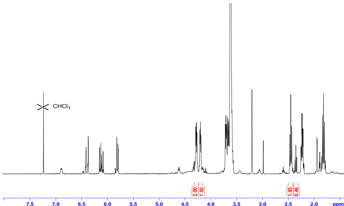
Figure II.5: ^1\text{H-NMR} spectrum ( \text{CDCl}_3 , 400 MHz) of PEG-acryloyl-5-hexynoate. The signal of -\text{CH}_2- of 5-hexynoic acid in the \alpha -position to the carbonyl is shifted from 2.38 to 2.47 ppm once it's coupled to PEG. The signal at 2.38 ppm on the spectrum corresponds to the excess of 5-hexynoic acid.
