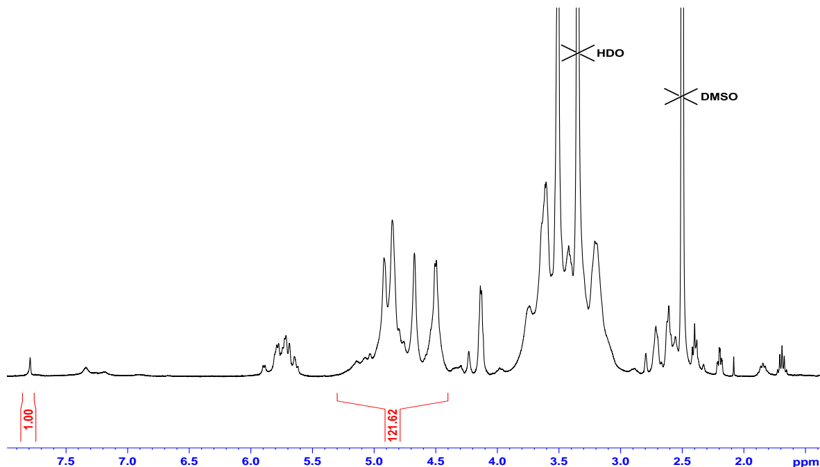
Figure II.9: ^1\text{H-NMR} spectrum ( \text{DMSO-d}_6 , 400 MHz) of DT40-g-PEG- \beta\text{CD} ( \text{DS}_{\text{CD}} = 3.7\text{mol.}\% ) prepared by CuAAC in pure water without TBTA ( P0 ). Redoubling of \beta\text{-CH}_2\text{-} protons of 5-hexynoate at 1.6-1.9 ppm is clearly observed.
