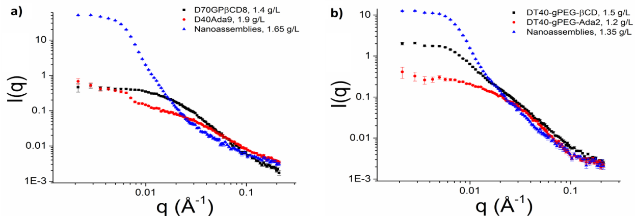
Figure II.34: SAXS scattering patterns representing the formation of HG-nanoassemblies between the polymers without (a) and with (b) hydrophilic PEG spacer ( C_{CD/Ada} = 5 \cdot 10^{-4} M).
