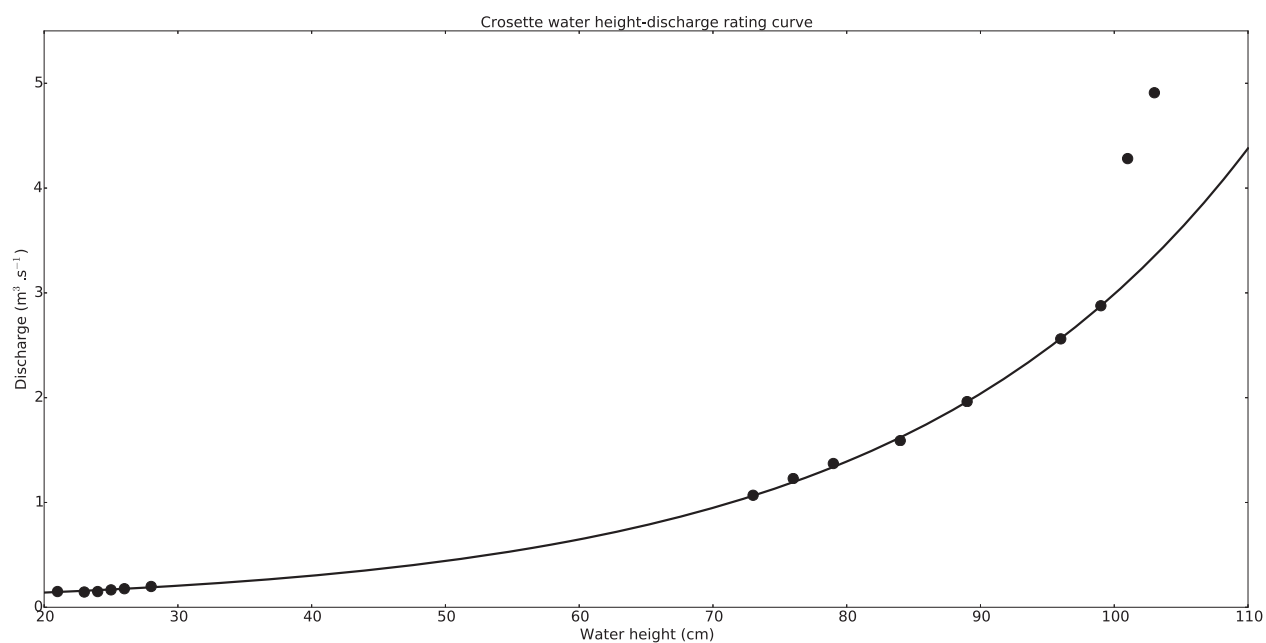
FIGURE B.3 – Crosette water height-discharge rating curve.
