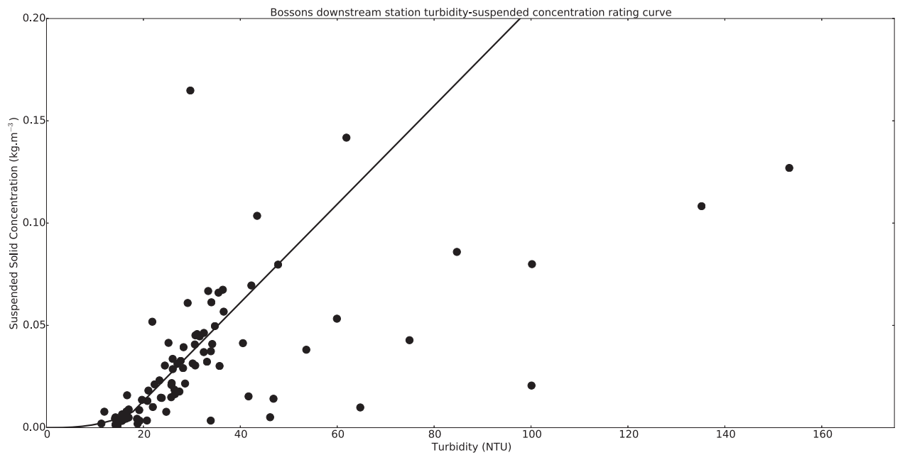
FIGURE B.1 – Bossons downstream station turbidity-suspended concentration rating curve.
