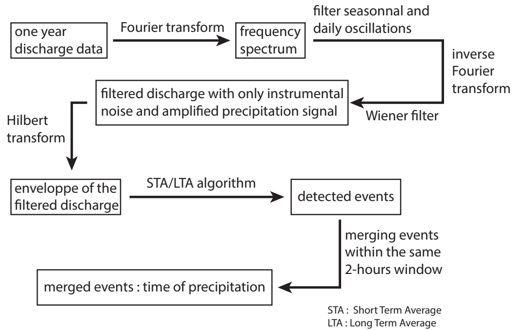
FIGURE C.23 – Signal processing of the discharge to identify rain periods.
