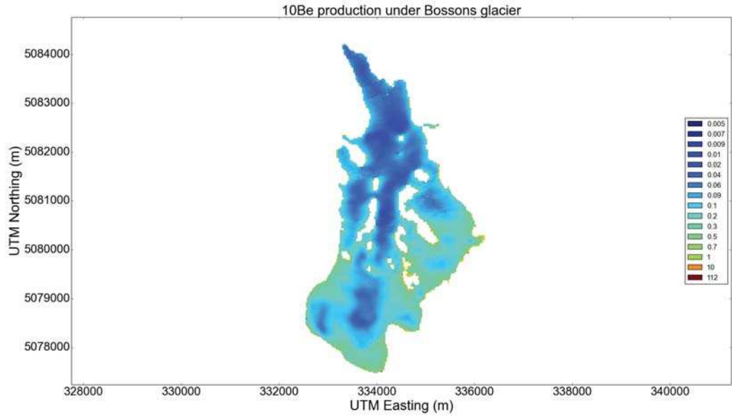
FIGURE A.4 – ^{10}\text{Be} production under Bossons glacier calculated using thickness from the Huss and Farinotti (2012) model and relations (A.1-A.13). Production rates are given in \text{at.g}^{-1}.\text{yr}^{-1} .
