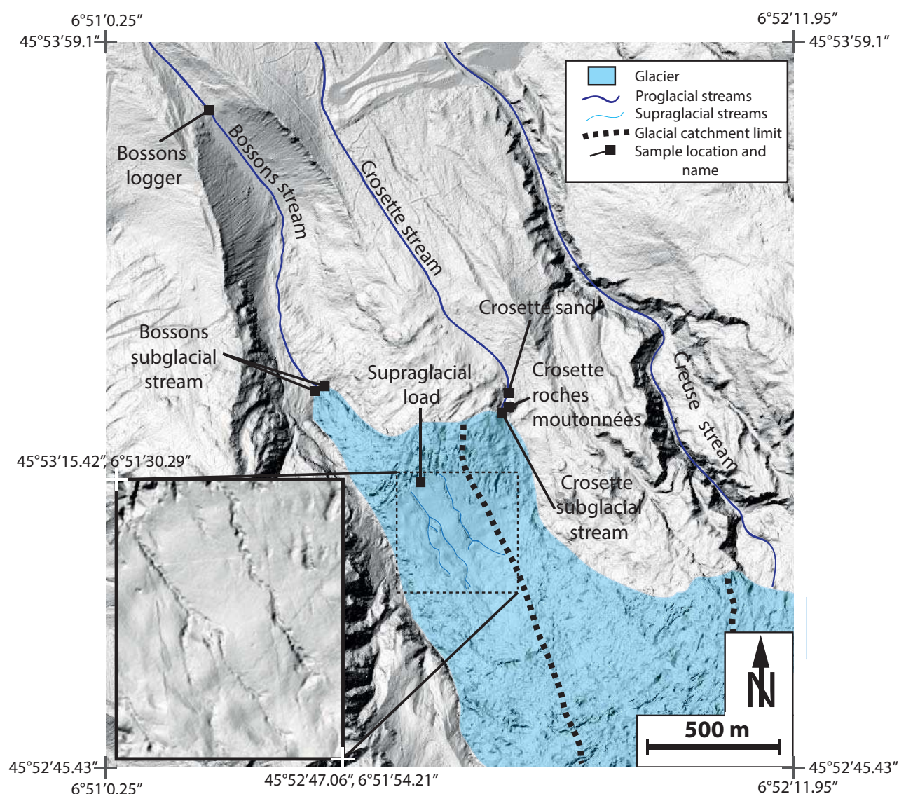
Figure 1.4 – Shaded relief map of the lower part of the Bossons glacier, based on 1-m resolution airborne Lidar data collected in 2008 (IRSTEA, unpublished). Thick dashed lines show subglacial watershed limits as in Figure 1.1. Supraglacial channels and sinkholes are only present above the subglacial watershed of the Bossons stream. Sampling locations for TCN samples are indicated by black squares. Detailed information including TCN concentration for each sample can be found in Table 1.1.
