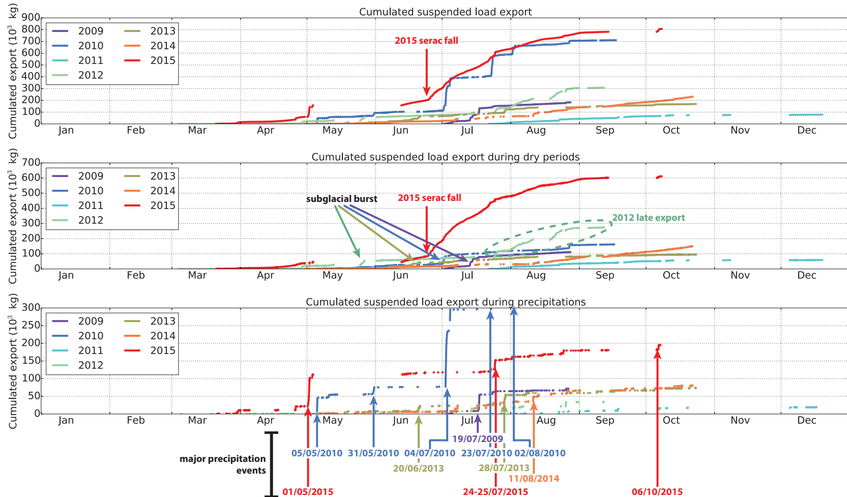
FIGURE 5.9 – Cumulated export of suspended load for Bossons stream between 2009 and 2015. a) Cumulated export regardless of meteorological conditions ; b) Cumulated export during dry periods. Notice that most of the export occurs during dry periods. The 2015 serac fall event is reported as well as major increases linked to subglacial events in 2009, 2012 and 2013. ; c) Cumulated export during precipitations. Major rain events associated with intense export are identified.
