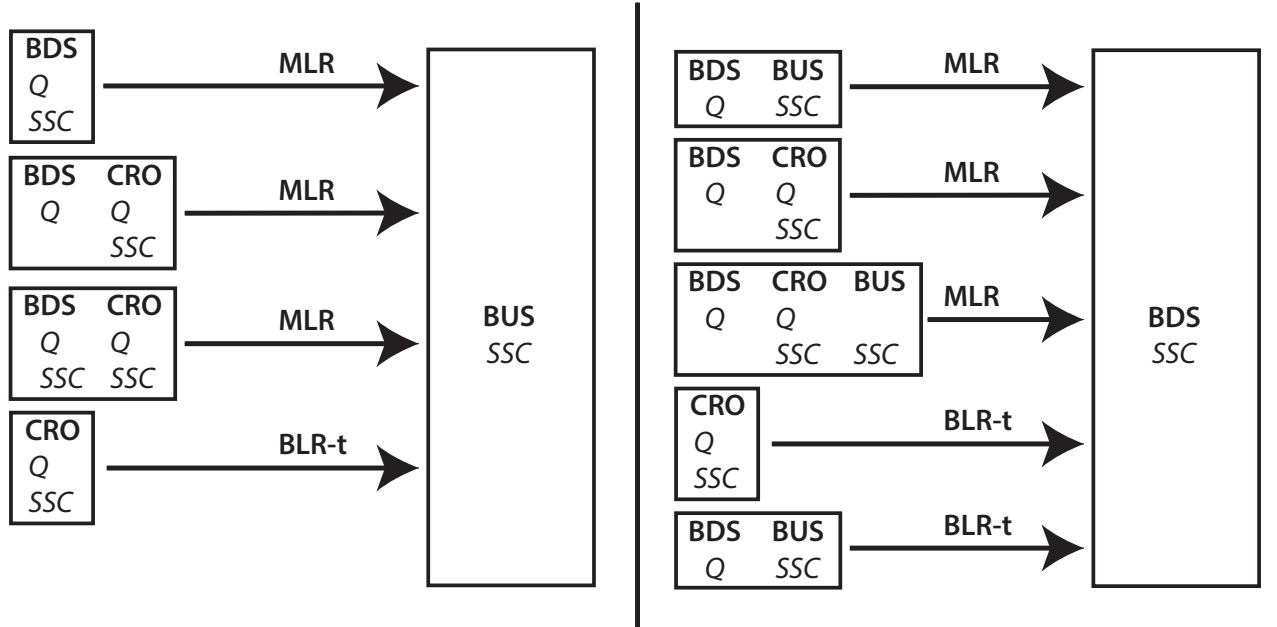
FIGURE C.10 – Data extrapolation with different methodologies at BUS station.
