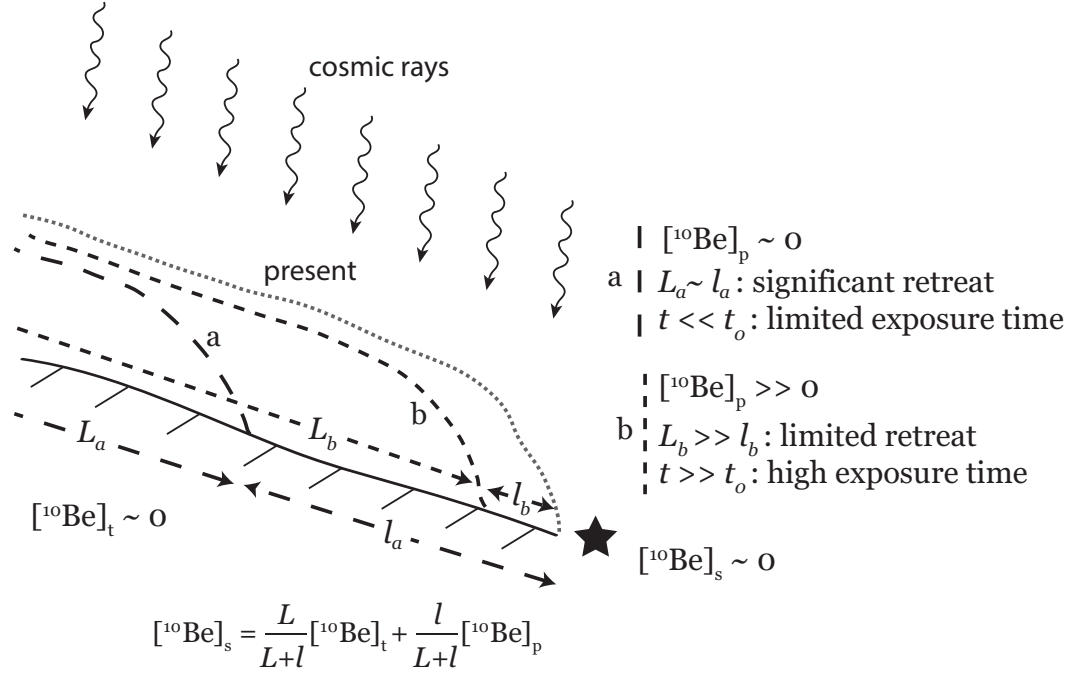
Figure 1.6 – Negligible ^{10}\text{Be} concentration in stream load related to glacial retreat scenarios. Ice-covered bedrock ^{10}\text{Be} concentration ( [^{10}\text{Be}]_t ) is negligible whereas the concentration in proglacial bedrock ( [^{10}\text{Be}]_p ) may not be. Black star represents a measurement location within a stream. L is the stream length beneath the glacier whereas l is the one within the proglacial area. (a) Short exposure time preventing significant ^{10}\text{Be} enrichment. (b) Limited glacial retreat so that ^{10}\text{Be} enriched proglacial area is negligible with respect to subglacial catchment area.
