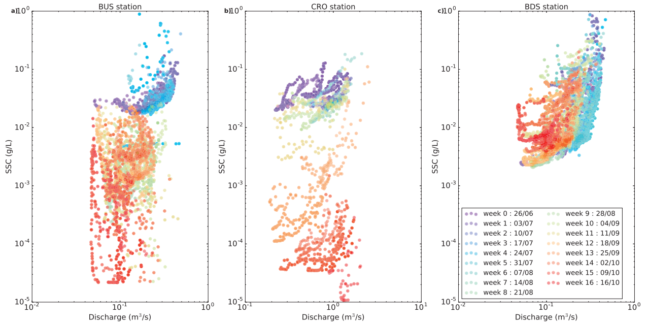
Figure 2.11 – Relation between discharge and SSC at BUS, CRO and BDS stations. Each point on the following log-log graphs represents a one hour average of our data. Colors represent the evolution by week throughout the respective dataset from violet to red for the early and late season, respectively. Oblique points clusters represent strong linear relationship, vertical clusters indicate lack of dependency on discharge from SSC where as horizontal clusters are linked to a stream already exporting as much as possible from the sediment supply. a) BUS station; b) CRO station; c) BDS station.
