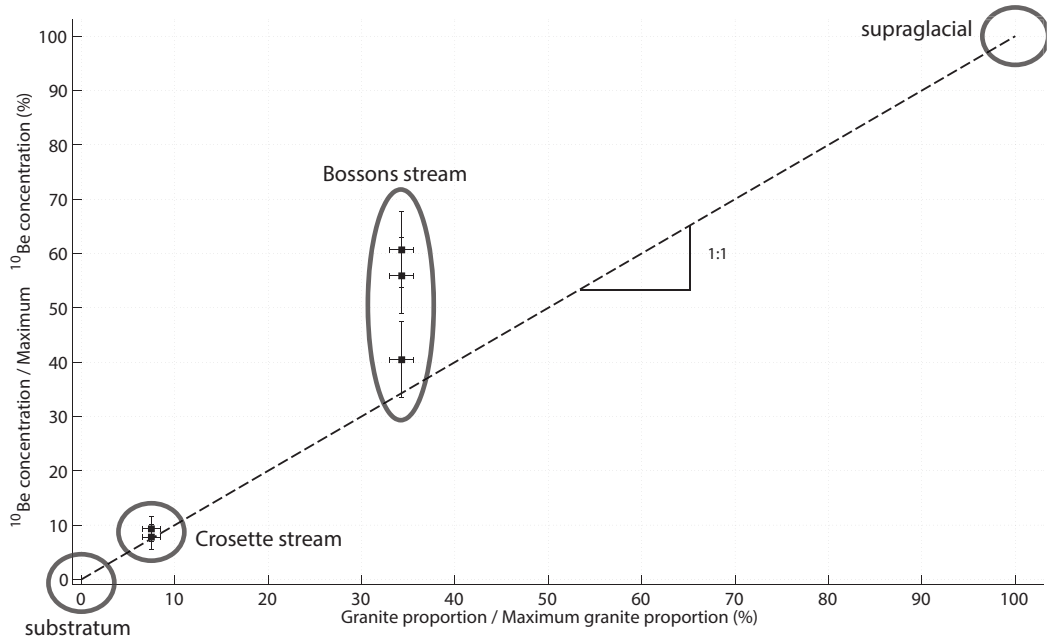
Figure 1.7 – Comparison between granite proportion (from Godon et al., 2013 ) and normalized ^{10}\text{Be} concentration for glacial substratum, subglacial stream sediments and supraglacial load.
