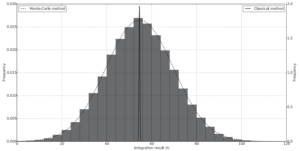
FIGURE C.5 – Histogram of the result of a Monte-Carlo simulation integrations on flux with 100000 trials. The dashed black line is the normal distribution fitted to the Monte-Carlo result. The solid black line is the normal distribution representing the classical method result.
