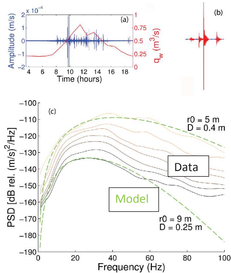
Fig. 1: Grain size estimates inverted using the model of Tsai et al. (2012) by considering the seismic signal acquired along the “Les Bossons” River during an extreme flood event. (a) Ground velocity (blue) recorded at 1 of the 4 deployed seismic stations, superimposed with water discharge (red). (b) Zoom on the seismic signal plotted in (a), showing large impulses associated with single grain impacts. (c) Recorded PSDs associated with automatically picked impulses (contiguous lines) and inverted PSDs using the model of Tsai et al. (2012) (dashed lines). The inversion is performed by tuning two parameters: the distance r_0 between the grain impact and the seismic station, and the grain size D .
