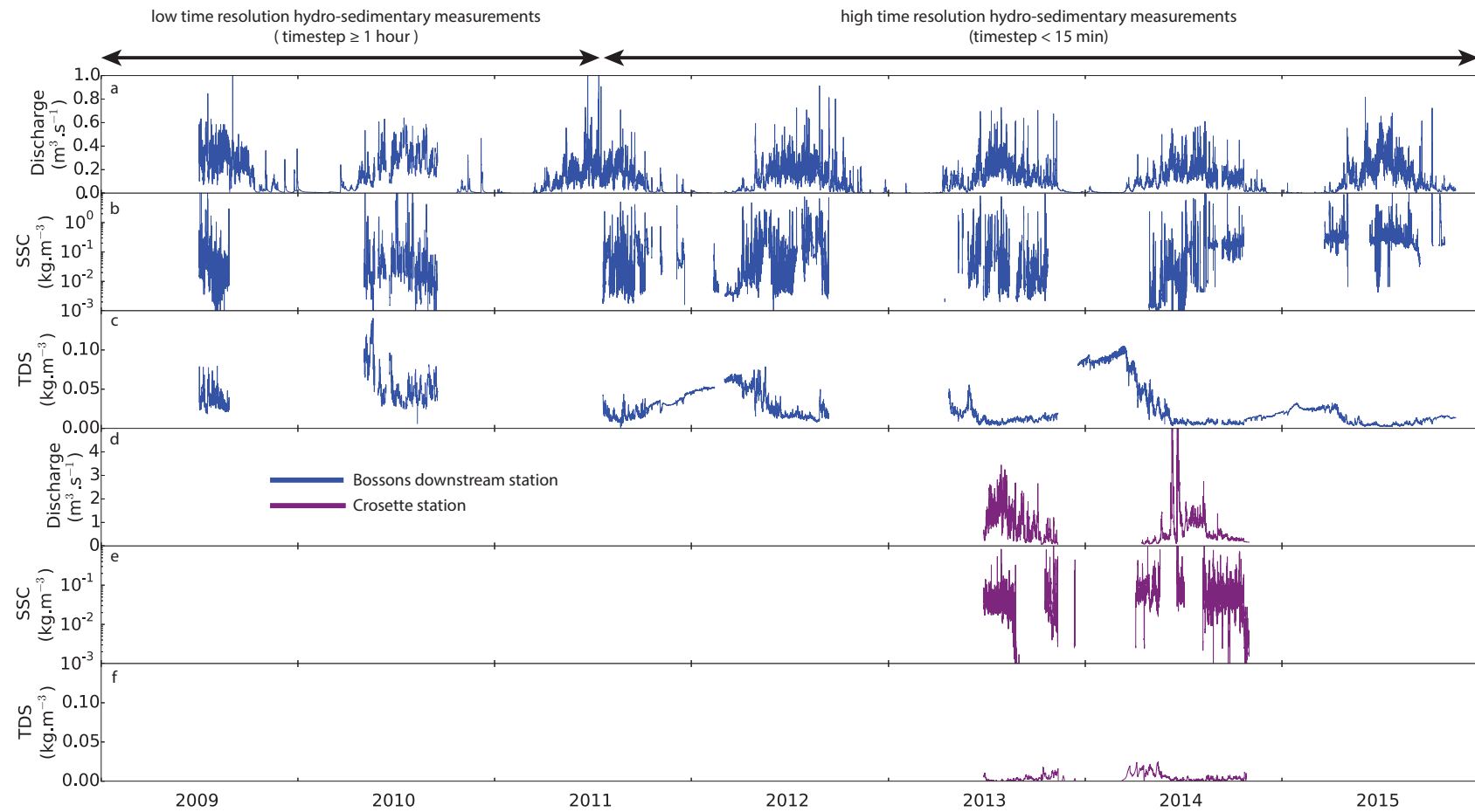
FIGURE 5.8 – Hydro-sedimentary data measured at the Bossons downstream station (a-c, blue) and at the Crosette station (d-f, violet). a,d) Water discharge; b,e) Suspended Sediment Concentration (SSC); c,f) Total Dissolved Solids (TDS). Periods of low and high time resolution are reported.
