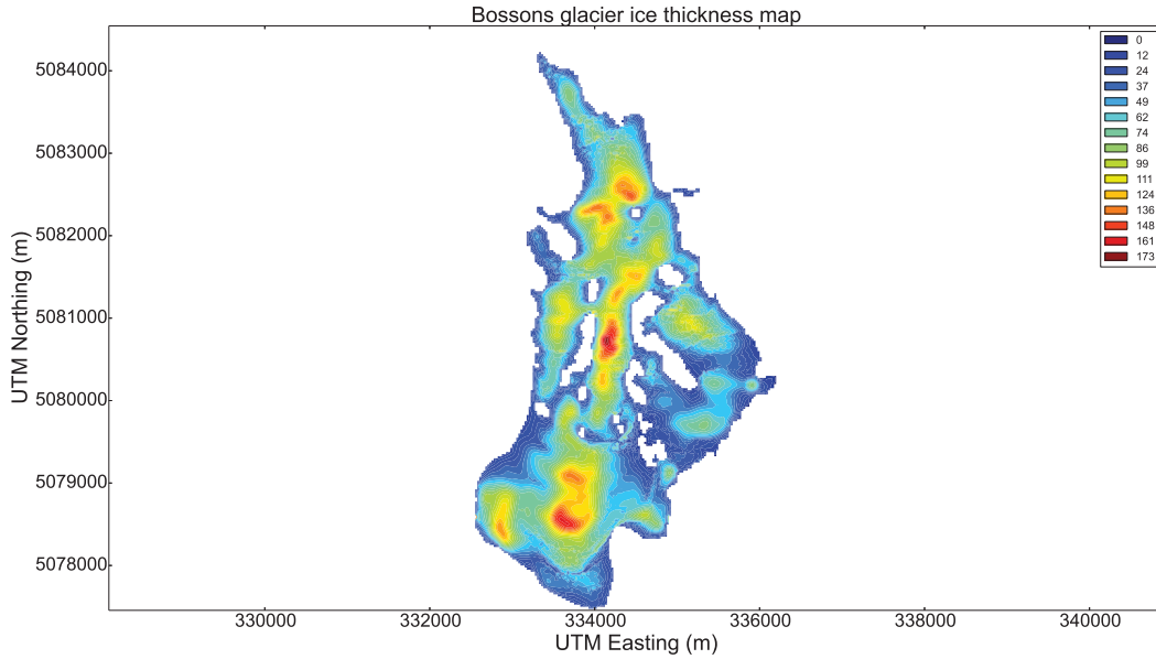
FIGURE A.2 – Bossons glacier ice thickness calculated using output of Huss and Farinotti (2012) model. Ice thickness in m.
