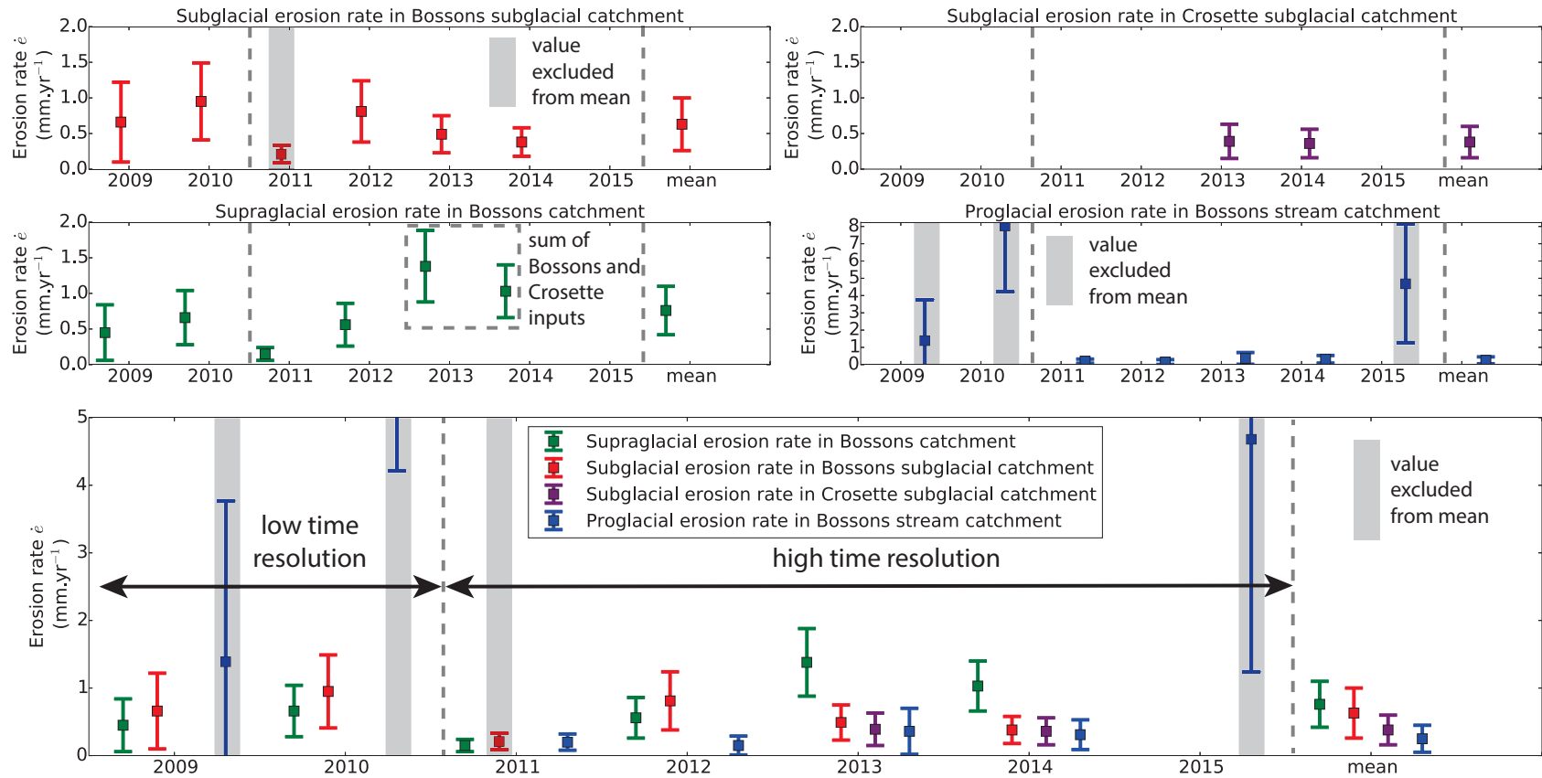
FIGURE 5.15 – Erosion rates estimated during a standard melt season lasting 187 days for the supraglacial (green), subglacial (red) and proglacial (blue) domains of the Bossons glacier from 2009 to 2015. Subglacial erosion rate for Crosette (violet) is displayed when data are available. Mean for each geomorphologic domain are displayed at the right. The 2009 and 2010 proglacial values have been excluded from the mean due to high uncertainties and extreme values during rain events, respectively. The 2011 subglacial erosion rate does not fully represent the subglacial erosion as it only corresponds to the late melt season. The 2015 supra and subglacial values have been estimated from 2009, 2011, 2013 and 2014 values and are not taken into account into the mean calculation (see text).
