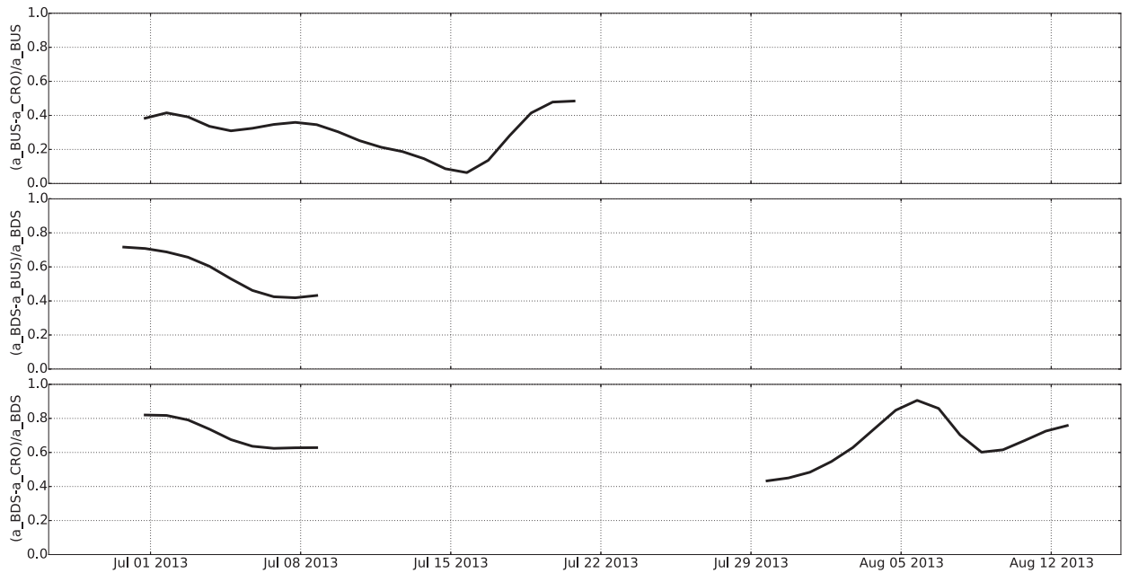
FIGURE C.11 – Temporal evolution of the ratio between slopes of the log Q - log SSC relationships at each stations.
