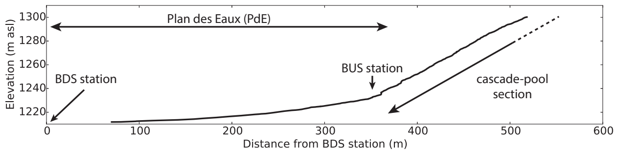
Figure 2.4 – Altitudinal profile of Bossons stream.
