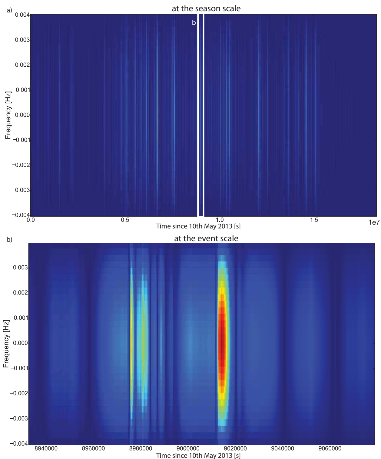
FIGURE C.21 – Spectrogram of the 2013 discharge. a) At the season scale; b) at the event scale.
