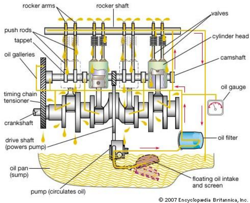
Figure 7. Engine lubrication system (source: Encyclopædia Britannica, Inc.).
