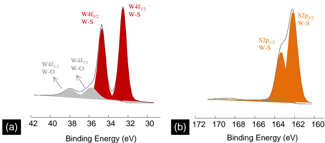
Figure 42. XPS spectra of WS 2 nanoparticles: (a) W4f region, (b) S2p region
