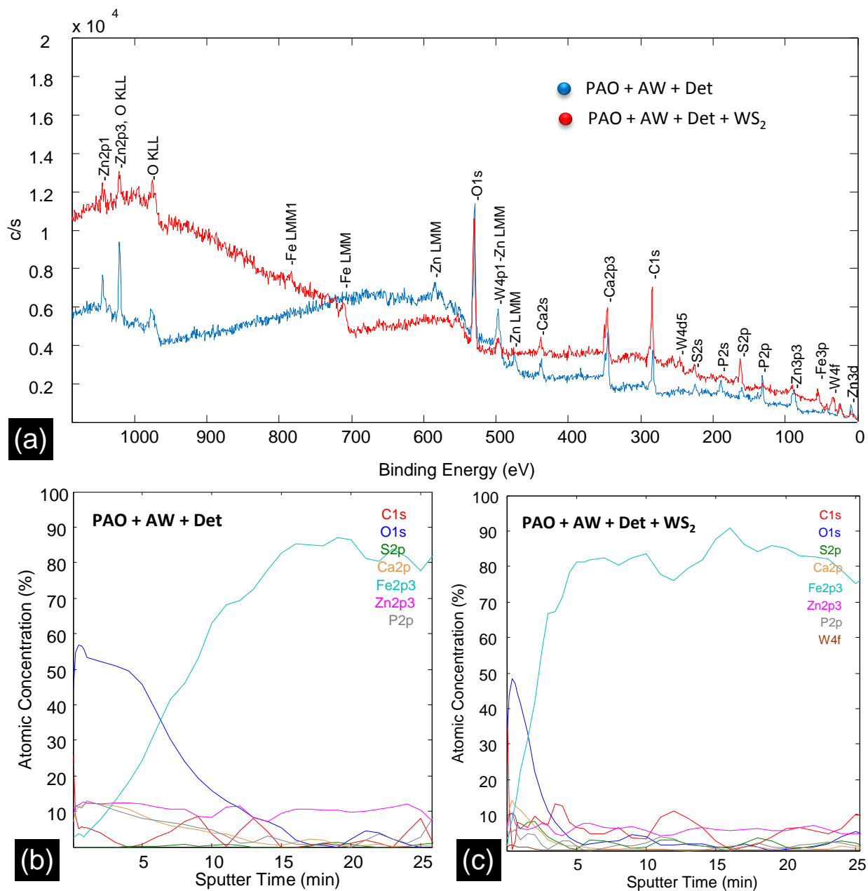
Figure 92. XPS spectra of the tribofilm formed by both samples at the end of the test a) survey scan b) elementary depth profile of the tribofilm formed by the reference sample and c) elementary depth profile of the tribofilm formed by the sample that contained the nanoparticles
