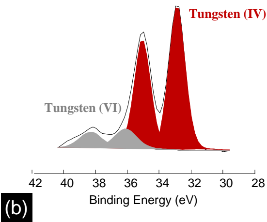
Figure 83. XPS spectra of the tribofilm formed by the nanoparticles in the presence of ZDDP additive on the rough steel flat; a) survey scan; b) W4f energy region and c) S2p energy region
