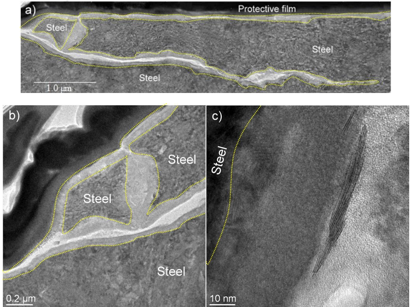
Figure 109. a) TEM image of the FIB preparation (Sample B), b) zoom-in at the beginning of the crack, and c) zoom-in on a zone containing sheets of WS_2
