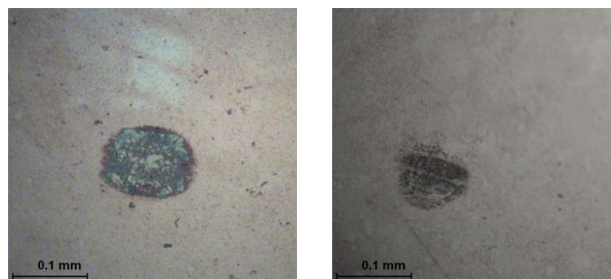
Figure 86. Wear scars for the sample containing ZDDP and detergent without (left) and with (right) the nanoparticles
