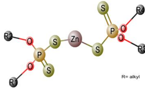
Figure 15. Molecular structure of ZDDP molecule.
