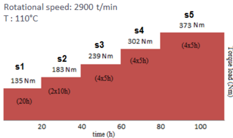
Figure 95. FZG testing program (rotational speed and temperature were constant across the load stages)
