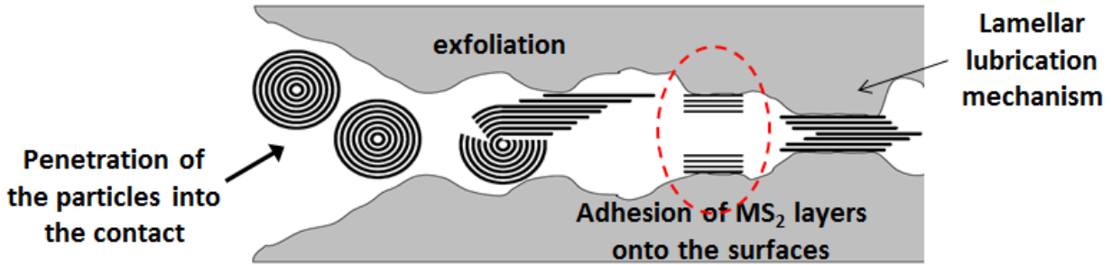
Figure 20. Lubrication mechanism of the MS_2 fullerene like nanoparticles in a steel/steel contact.
