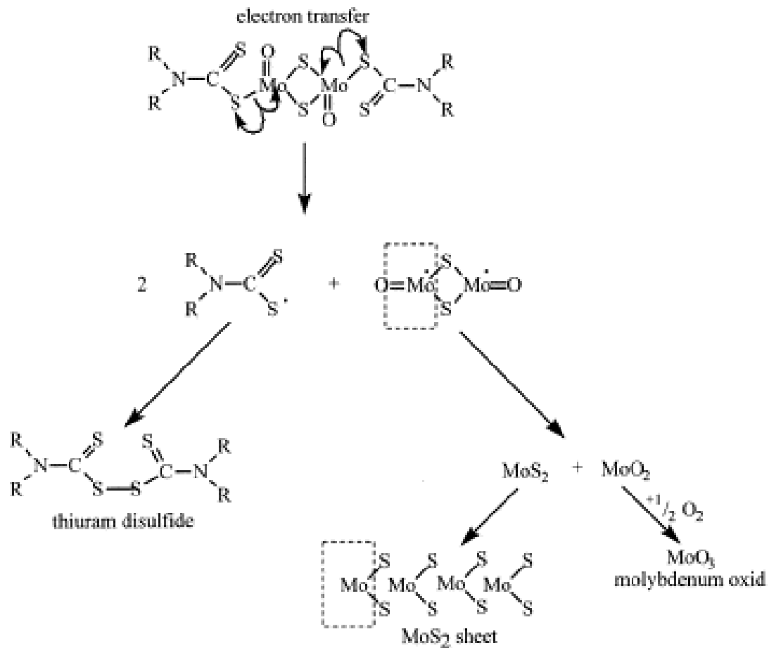
Figure 17. \text{MoS}_2 chemical process formation from MoDTC (62).
