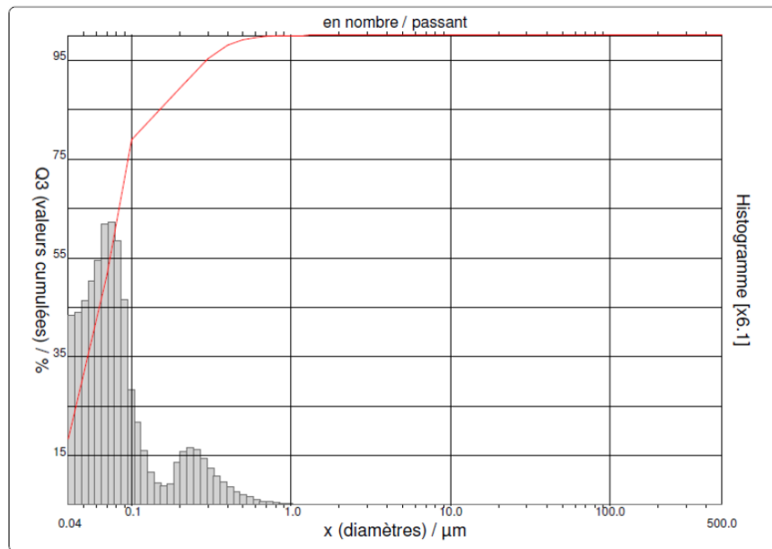
Figure 41. Particle size distribution of the nanoparticles
