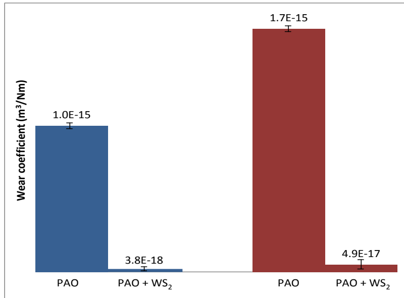
Figure 48. Wear coefficient calculated for PAO and PAO + WS_2 nanoparticles at room temperature (blue) and 100^\circ C (red)
