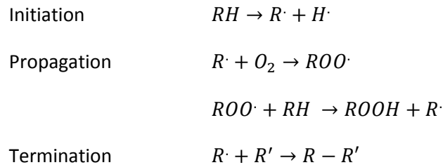
Figure 69. Lubricants oxidation schema
