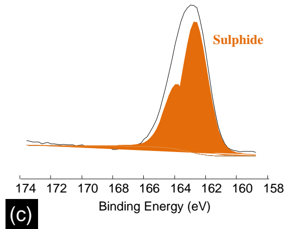
Figure 83. XPS spectra of the tribofilm formed by the nanoparticles in the presence of ZDDP additive on the rough steel flat; a) survey scan; b) W4f energy region and c) S2p energy region
