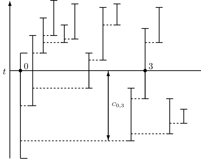
FIGURE 3.8 – Coalescence time between individuals 0 and 3 represented as an arrow.
