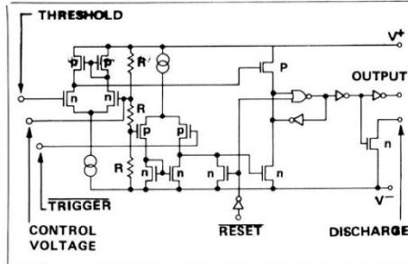
Figure 5. Equivalent circuit.
