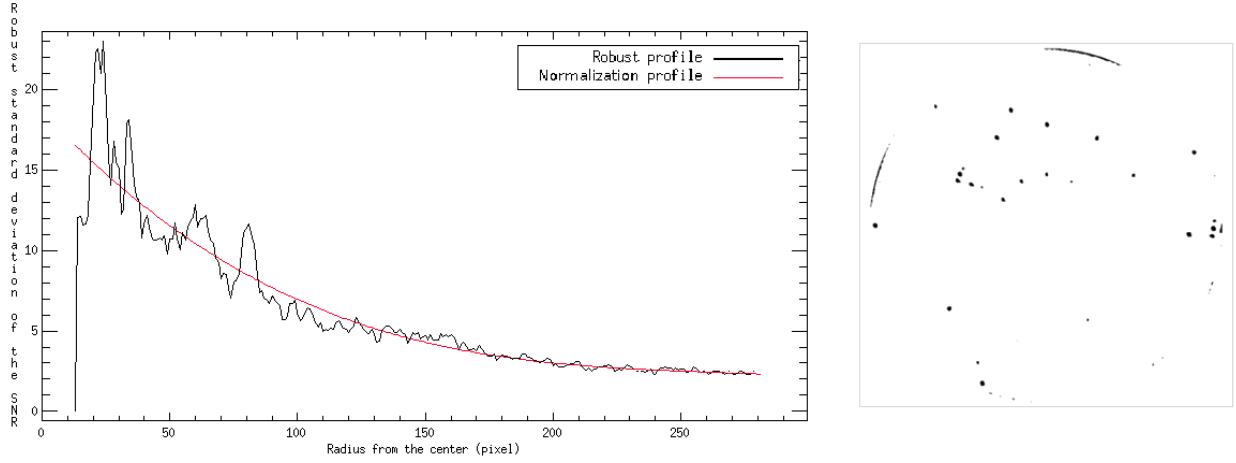
Figure 3.11 – Smoothing the normalization profile. Left: Normalization profile (red solid line) obtained by a 4th order fit of the radial robust standard deviation of the SNR map (black solid line). Right: SNR map normalized by this profile, thresholded to 5\sigma . The close companions are missing though visible on the non-thresholded SNR map.
