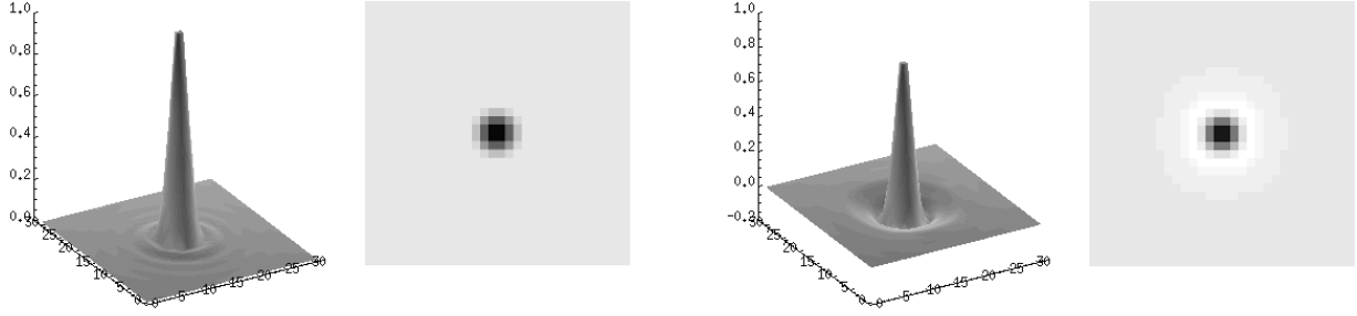
(a) : Reference PSF (here a noiseless Airy pattern defined on a 64 \times 64 pixels frame, with an oversampling of 1.66) - Without filtering.
