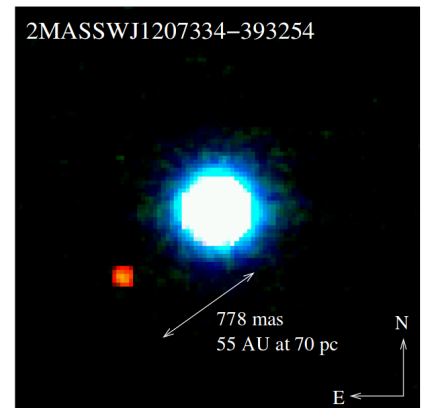
Figure 1.4 – First exoplanet detected around a brown dwarf, using the VLT/NaCo instrument (Figure from Chauvin et al., 2004).
