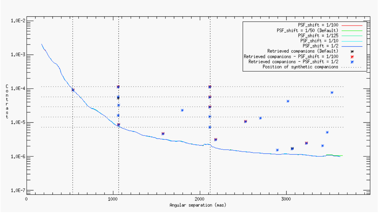
Figure 4.17 – Detection limits retrieved as a function of the size of the reference PSF subpixel shift, PSF_{shift} , used to build the model of the planet signature in the post-ADI images.
