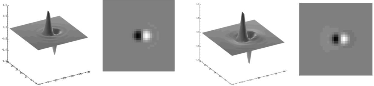
(c) : Resulting planet signature after the ADI (using \delta_{min} = 1\lambda/D ) - Without filtering.
