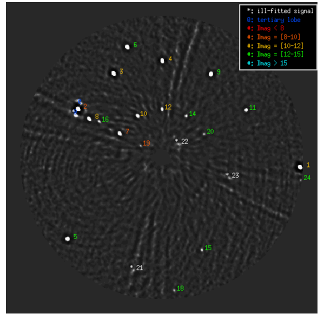
(b) : SNR map displaying the detections and their properties (position, SNR rank, flux range and if it is an artifact)
