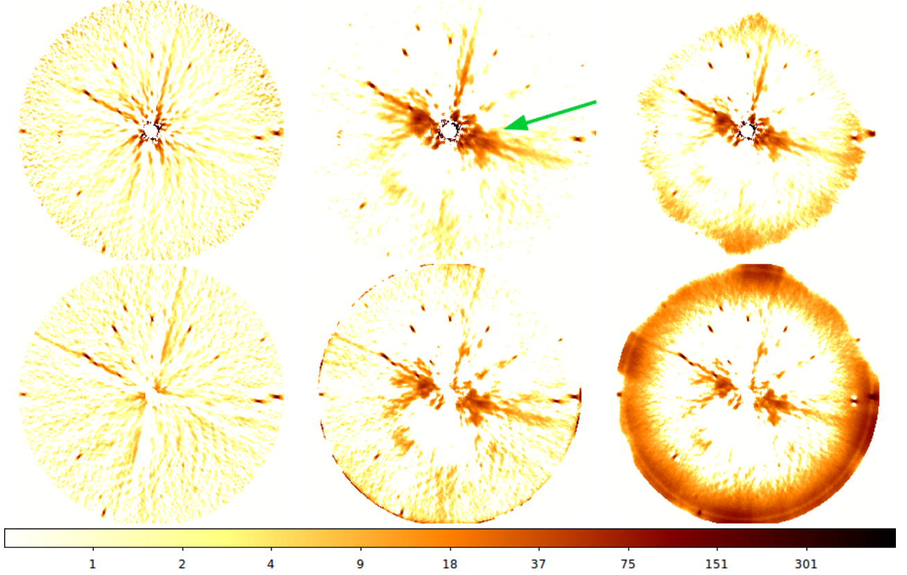
Figure 2.10 – SNR maps provided by ANDROMEDA using the parameters gathered in Tab. 2.4. From left to right: Without ADI optimization, with the total ration (TR) optimization, with the least-square (LS) optimization. Top: using the 3D-variance map. Bottom: using the 2D-variance map. The scale is logarithmic (in sigma units).
