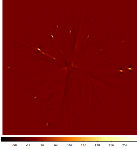
(a) : SNR map obtained by using no ADI optimization - Without filtering.
