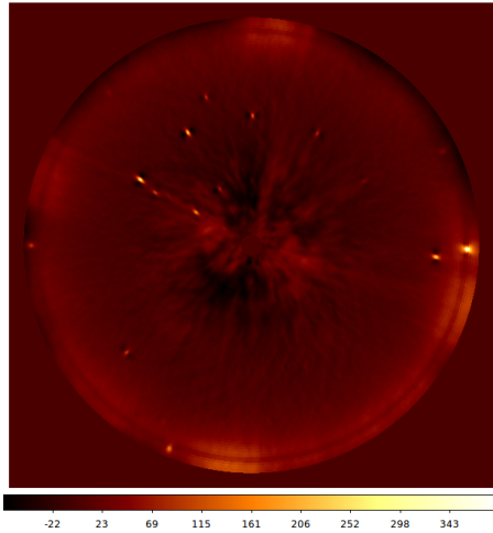
(e) : SNR map obtained by using a least-square ADI optimization - Without filtering.
