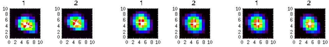
Figure 4.15 – Subimages of the first two detections according to the size of the reference PSF window set. From left to right: N_{PSF} = 8 \times 8 pixels, N_{PSF} = 16 \times 16 pixels and N_{PSF} = 64 \times 64 pixels
