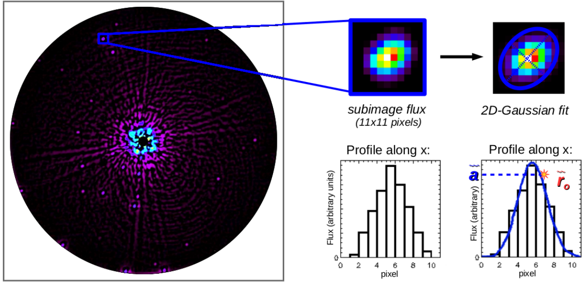
Figure 3.37 – Sketch of the determining of the point source signal flux by a 2D-Gaussian fit, at the estimated position \hat{r}_0 .
