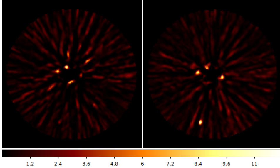
Figure 6.16 – Maps obtained by combining the 39 SNR maps obtained by running ANDROMEDA in ADI (channel per channel) on the SPHERE-IFS data of 51Eri, as in Thiebaut et al. (2016) . Left: YJ-bands ( \text{SNR}_{51\text{Eri}b} = 3\sigma ). Right: YH band ( \text{SNR}_{51\text{Eri}b} = 11.5\sigma ). In both maps, the SNR of the highest residuals, located at \sim 75 mas from the star, are of about 10\sigma : Eri51 b is the highest signal in the YH map but not in the YJ map.
