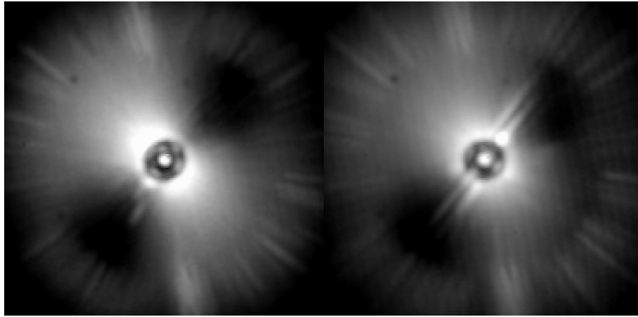
Figure 6.14 – Reduced images from SPHERE-IFS data of the star 51Eri, collapsed on all wavelength in YJ bands (left) and YH bands (right).
