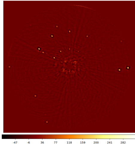
(f) : SNR map obtained by using a least-square ADI optimization - With filtering.
