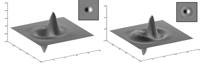
Fig. 2. Illustration of the planet signatures obtained when performing the ADI, setting \delta_{\min} = 0.5\lambda/D . These have been obtained by simulating two identical noiseless planetary PSF, separated by \delta_{\min} and then subtracted one from the other. Left : Planet signature obtained without high-pass filtering of the raw data. Right : Planet signature obtained when the raw data have been filtered of their low frequencies ( F = 1/4 ). This time secondary opposite lobes surround the main lobe.
