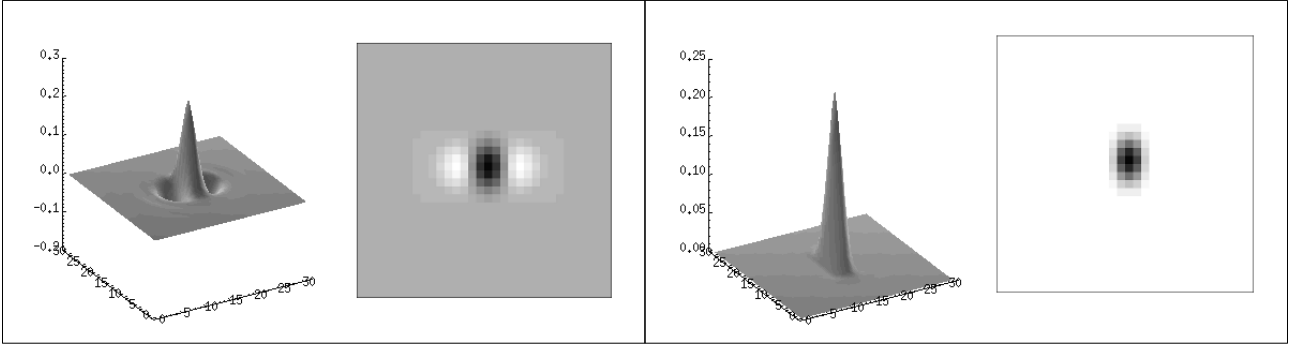
Figure 2.5 – Typical planetary pattern expected either in the flux map and in the SNR map, without (left) or with (right) the positivity constraint. These figures have been obtained by cross-correlating the planetary signature at Fig. 2.4 where \delta_{\min} is set to 1\lambda/D along the x-axis. Colors have been inverted: Black is high values and white is low values. The resulting planetary pattern is indeed oval, having its major axis perpendicular to the PSF shift axis (here the x-axis).
