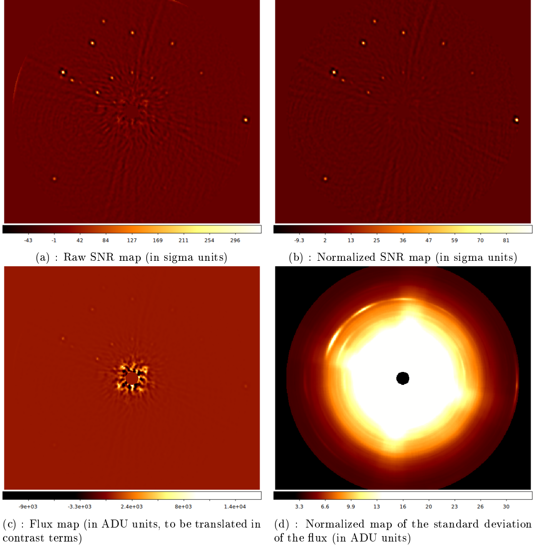
Figure 4: Maps output by the ANDROMEDA function and from which are made the detection, the astrometry, the photometry and the detection limit estimation.
