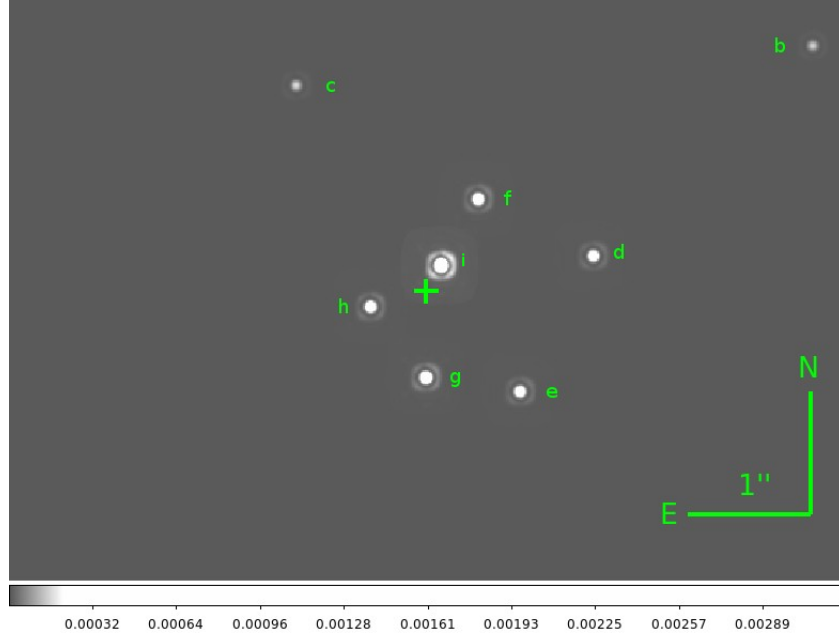
Figure 5.1 – Image showing the location and the contrast of the eight injected synthetic companions inside the SPHERE-IRDIS data. The green cross shows the location of the target star, centered on the central pixel of the frame .
