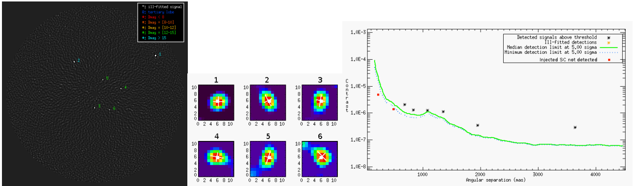
Figure 5.5 – Images output by the detection module of ANDROMEDA (see Sect. 3.3.5). From left to right: Detection map, subimages of each detection and corresponding detection limit at 5\sigma . For information, I a posteriori added the two non-detected synthetic companions (red squares).
