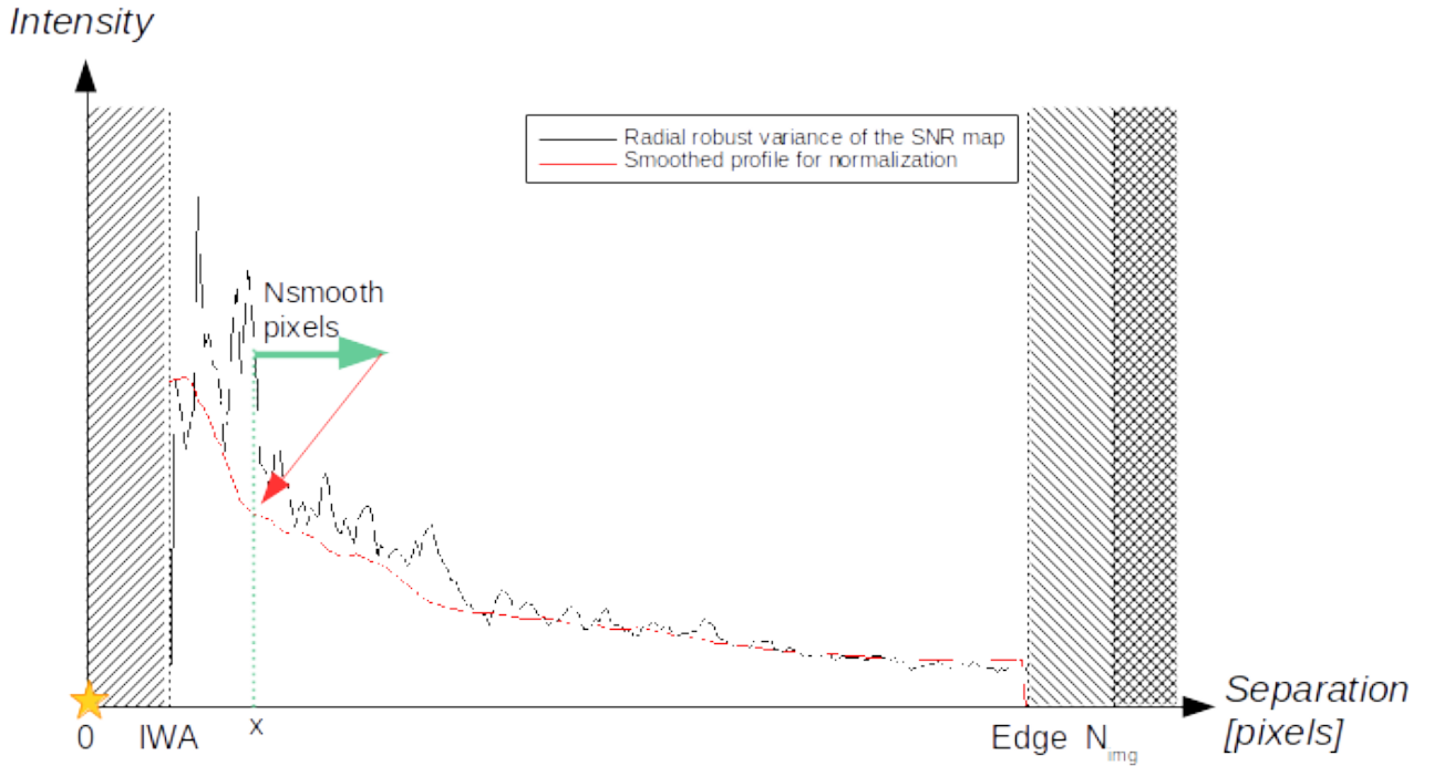
Figure 3: Schematic drawing of the smoothing made to build the normalization profile (red curve).
