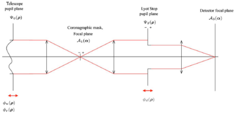
Figure C.1 – Schematic representation of a coronagraphic set up (From Sauvage et al., 2010).
