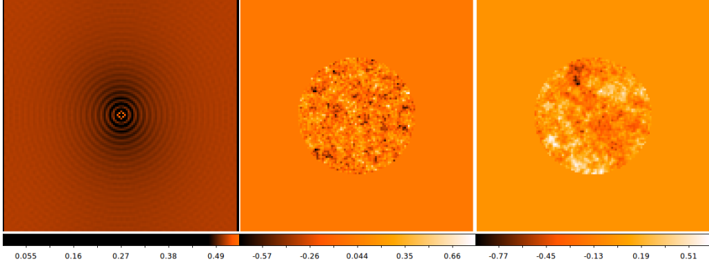
Figure 8.1 – Phase maps used to build the multispectral data cube for the inverse crime. Left: Turbulence residuals phase structure function, D_{\phi_{res}} . Middle: Static upstream phase, \phi_{up} (radians). Right: Static downstream phase, \phi_{down} (radians). To produce the multispectral cube, these three arrays are zero-padded into bigger arrays whose size are proportional to the wavelength ratio \lambda_i/\lambda_{Shannon} .
