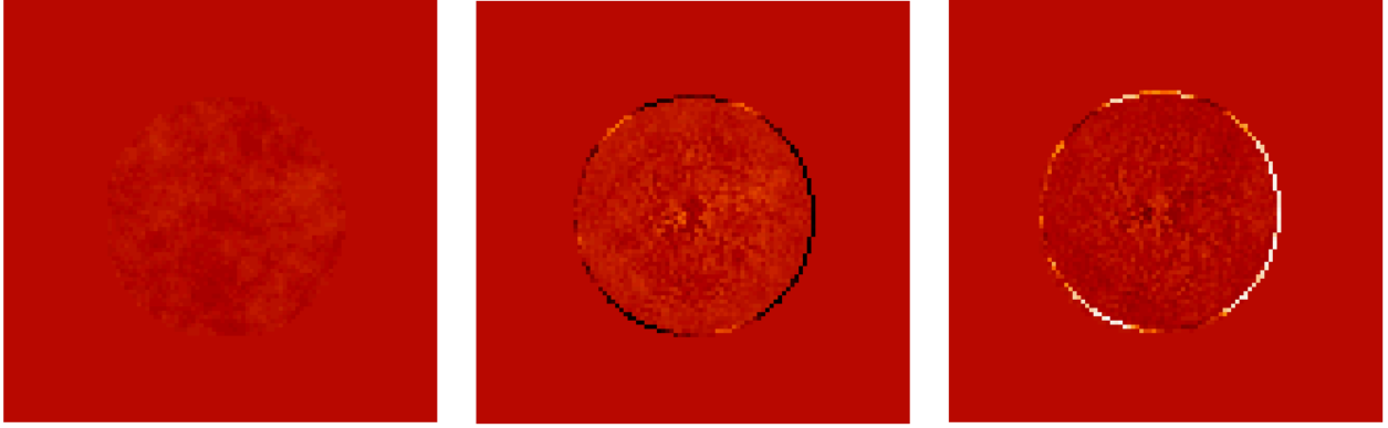
Figure 9.15 – Results from the whole MEDUSAE process. From left to right: Input upstream phase, estimated upstream phase and residuals (same scale).
