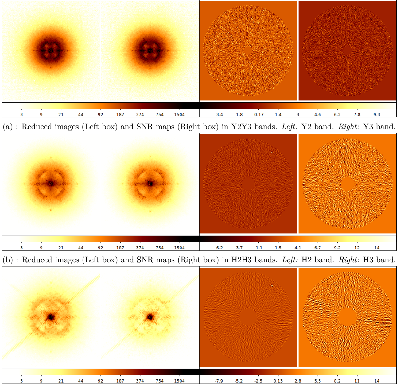
Figure 6.2 – One reduced image from the cube of the star GJ504 observed under the conditions gathered at Tab. 6.1 (left boxes, logarithmic scale, inverted colors). SNR maps provided by ANDROMEDA when using the user-parameters at Tab. 6.2 (right boxes).
