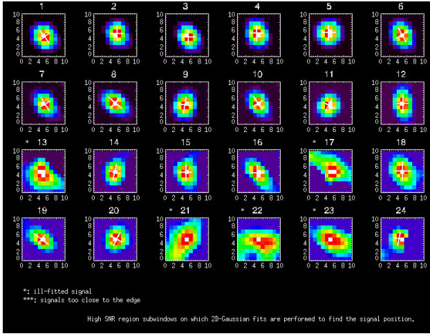
(a) : SNR subimages enclosing all the detected signals above the threshold set in which the analysis is made. When the 2D Gaussian fit could converge, its parameters are in-printed on the subwindow (maximum, semi major axis and semi minor axis).
