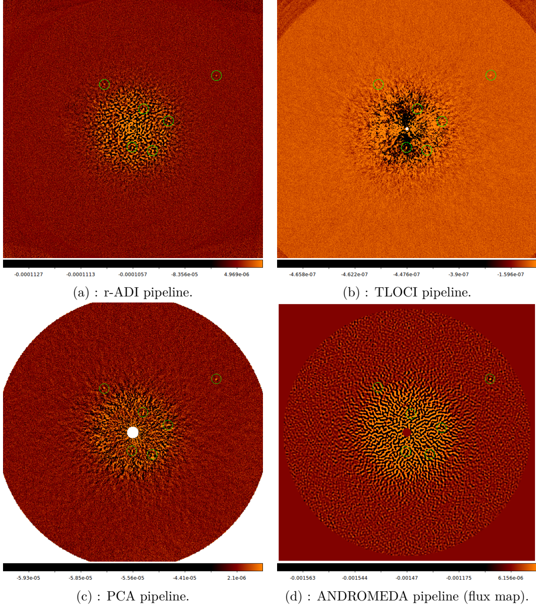
Figure 5.8 – Final images obtained for each pipeline. The images are given in logarithmic colors. For T-LOCI and PCA, these maps are used to perform the detection by visual inspection. For r-ADI and ANDROMEDA, the detection is made via the SNR map, respectively by visual inspection and by thresholding.
