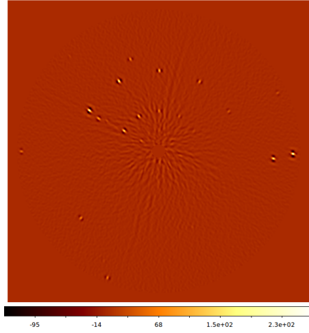
(b) : SNR map obtained by using no ADI optimization - With filtering.
