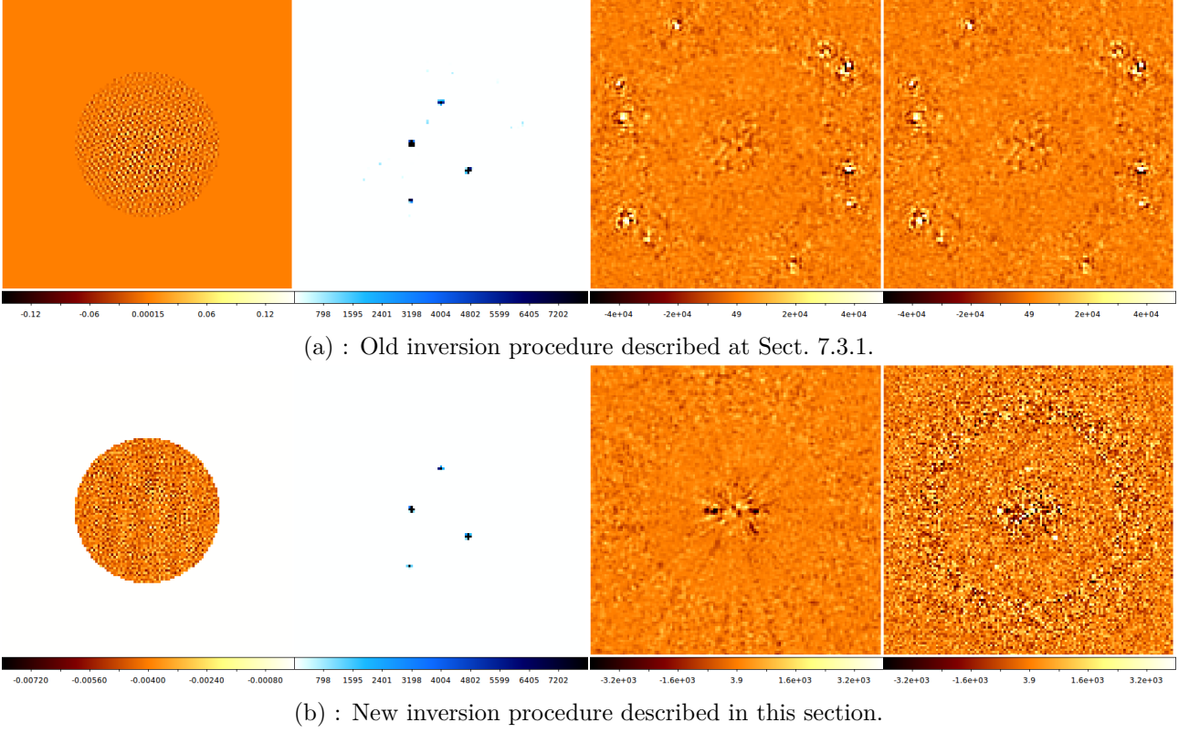
Figure 8.7 – Results obtained by running MEDUSAE on the inverse crime data, for the two different inversion procedure. From left to right: residual aberration map, estimated object map (inverted colors), residual speckle field and residual image. The scale is linear but the bounds different for every image.
