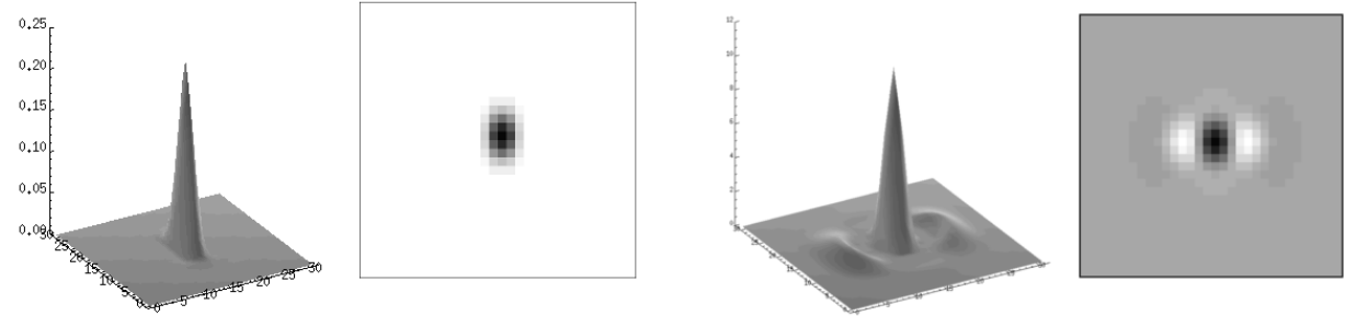
(e) : Resulting pattern after the MLE (using the positivity constraint) - Without filtering.
