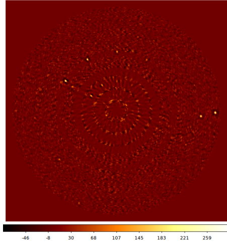
(d) : SNR map obtained by using a total-ratio ADI optimization - With filtering.
