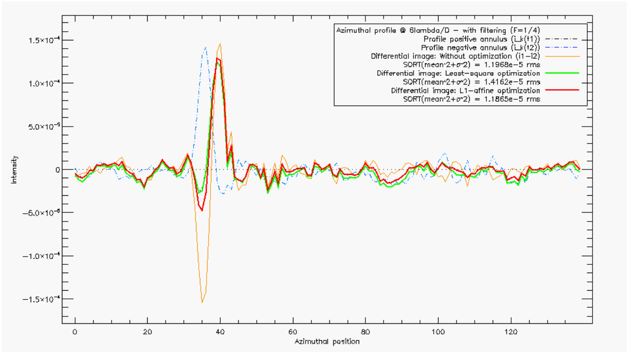
Figure 3.26 – Azimuthal profile (over a one pixel's wide annulus) of the differential images obtained by subtracting the annuli used at Fig. 3.25, according to the optimization method used. In order to compare the three methods, the rms value of the profile deprived of the planetary signal is indicated in the legend. The profile of i_k(t_1, \mathbf{r}_{\text{sub}}) and i_k(t_2, \mathbf{r}_{\text{sub}}) are over-plotted in dashed-line (respectively black and blue lines).
