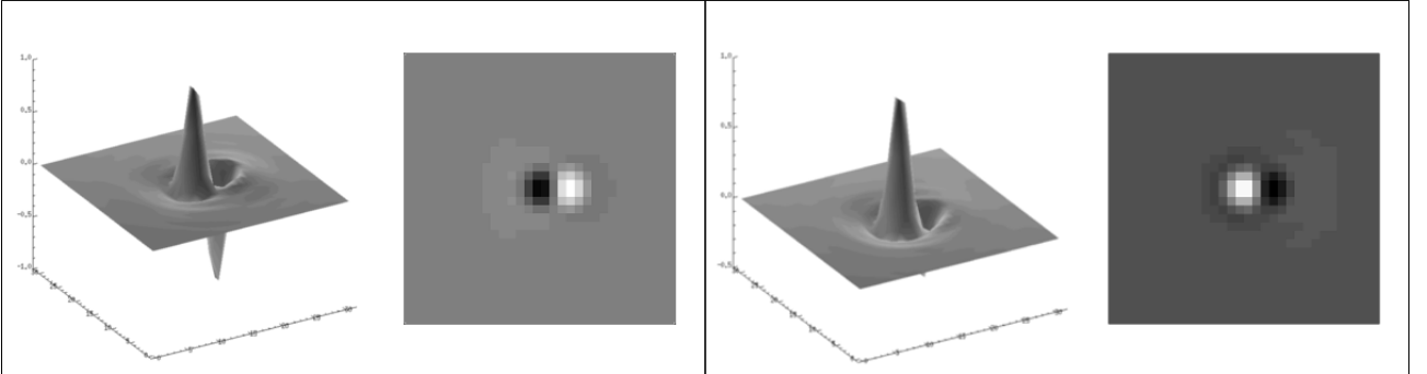
Figure 3.32 – Model of the planet signature (with pre-filtering, F = 1/4 ), without (left) or with (right) the scaling factor taken into account ( \gamma_{LS} = 0.4 in this example). As in Fig. 2.4, this planet signature is obtained by shifting the reference PSF of \delta_{min} (here only the distance \delta_{min} is not angular but along the x-axis; \delta_{min} = 1\lambda/D ). This illustration is made thanks to an Airy pattern sampled with an oversampling rate of 1.6 and normalized to its maximum.
