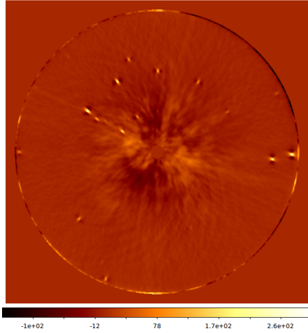
(c) : SNR map obtained by using a total-ratio ADI optimization - Without filtering.
