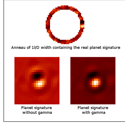
(b) : One differential annulus of width d_r = 1\lambda/D containing the signal of \beta Pictoris b and corresponding planet signature.
