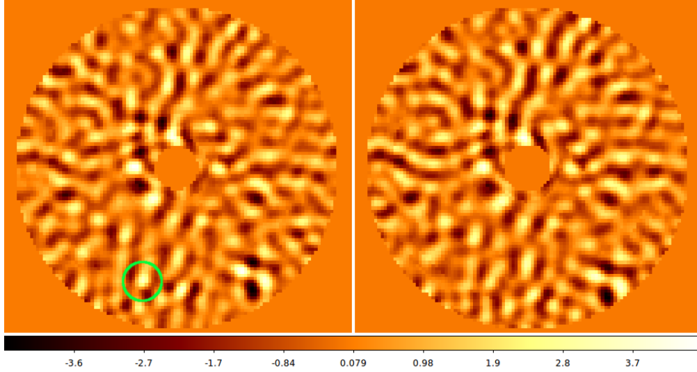
Figure 6.7 – SNR maps obtained by running ANDROMEDA on the 51Eri data, described at Tab. 6.6, using the parameter set at Tab. 6.7, in H2-band (left) and H3-band (right). The companion 51Eri b is visible on the left panel inside the green circle.
