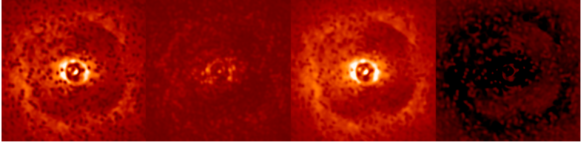
(a) : Test #1 (after initialization at only one wavelength).
