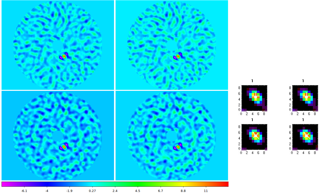
Figure 3.34 – SNR maps (left) and corresponding subimages (right) obtained by running ANDROMEDA on the data set presented in Sect. 3.2.1, using the parameters gathered in Tab. 3.2. From left to right: SNR map obtained with a least-square optimization and SNR map obtained with a L1-affine optimization. From top to bottom: SNR map obtained by using a model without the scaling factor and SNR map obtained by using a model with the scaling factor. In each of these maps, the companion \beta Pictoris b is the only signal found above the 5\sigma threshold, with a SNR of (from left to right, top to bottom): 14.80\sigma , 14.08\sigma , 14.47\sigma and 14.03\sigma .
