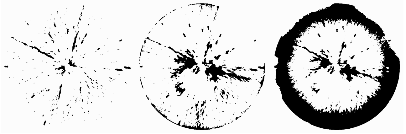
Figure 2.12 – SNR maps thresholded at 5\sigma , provided by ANDROMEDA using the parameters gathered in Tab. 2.4, using an empirical 2D-variance map. From left to right: without ADI optimization, with a total ratio optimization of the ADI and with a least-square optimization. Colors are inverted: white corresponds to zero and black to one.
