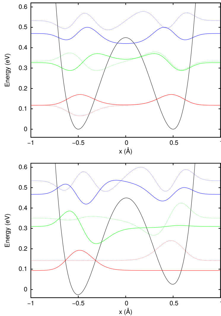
Figure 4.1.1: Symmetric ( E = 0 - top panel) and asymmetric ( E = 0.014 \text{ V.}\text{\AA}^{-1} - lower panel) double well potential (see equation (4.1.1)) and corresponding proton wave functions, calculated numerically. The baselines of the wave functions have been shifted to represent the energy levels. In both cases, P = 10 \text{ GPa} i.e. we are considering the situation of a high barrier.
