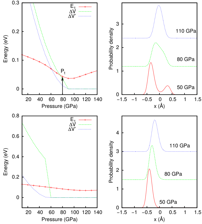
Figure 4.1.4: Left panels: Evolution of zero-point energy E_1 and barrier heights \Delta V and \Delta V' as functions of pressure for two different values of E (top panel: E = 0.014 \text{ V.Å}^{-1} , lower panel: E = 0.14 \text{ V.Å}^{-1} ). P_t indicates the quantum transition pressure (i.e. \Delta V = E_1 ). Right panels: Probability density \rho(x, T) at room temperature and different pressures for E = 0.014 \text{ V.Å}^{-1} (top panel) and E = 0.14 \text{ V.Å}^{-1} (lower panel).
