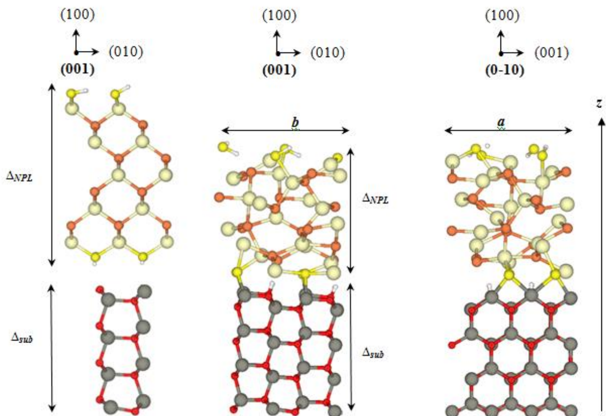
Figure AI.1. a) Structure of the isolated subsystems: 9 layers thick (9L) CdSe.SH and 8 layers thick (8L) ZnO slabs. b) Optimized geometry of the CdSe.SH (9L) – ZnO (8L) heterostructure, viewed along the (001) and (0-10) directions.
