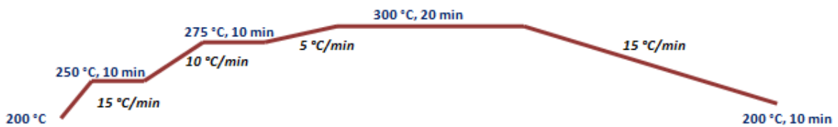
Figure II.5. Ramping program for the thermal treatment of seeded FTO glasses prepared with the spin-coating of Zn(Ac) 2 solution with method 1).
