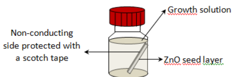
Figure II.6. Experimental setup for the ZnO NR growth.
