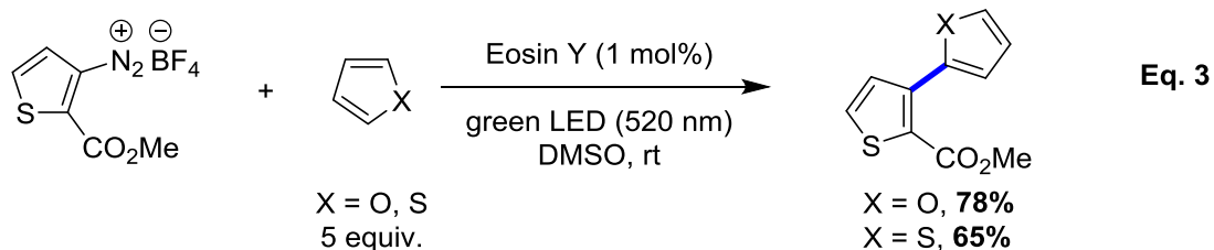
Scheme 6. Formation of aryl radical by photoreduction of diazonium salts
