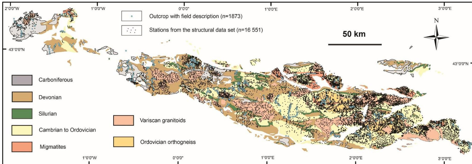
Figure S1. Location of i) structural data retrieved from works in the literature and existing geological maps and ii) field stations of the present study, shown on a simplified geological map of the Pyrenees.
