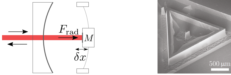
Figure 1.1: Left: The generic optomechanical system, a Fabry-Perot cavity with one movable mirror. The displacement \delta x modifies the phase of the reflected laser beam, and the radiation-pressure force F_{\text{rad}} exerted by the laser modifies the position of the mirror by an amount that is inversely proportional to the effective mirror mass M . Right: Scanning electron microscope (SEM) image of the mechanical resonator studied in this thesis.
