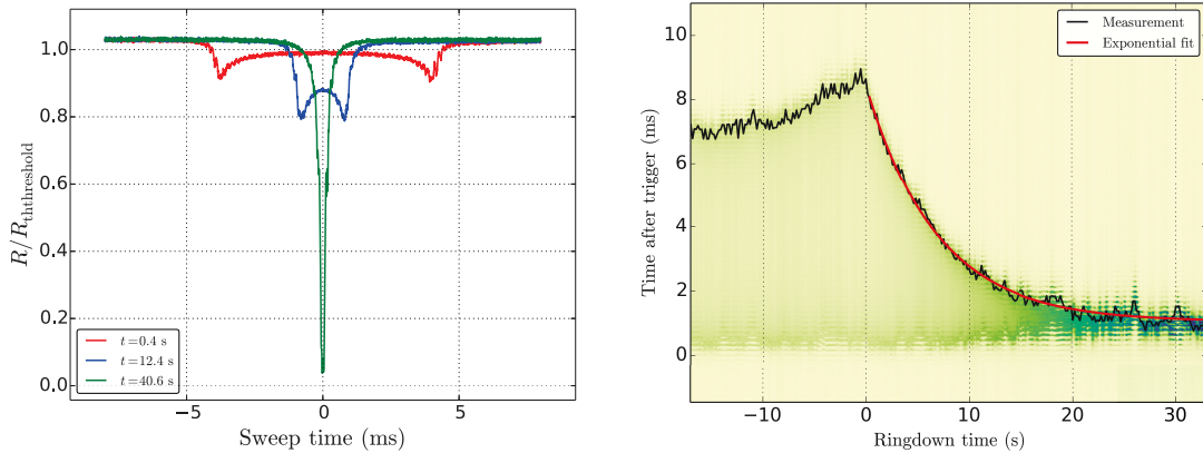
Figure 7.8: Left and right: Cavity length sweep ringdown measurement. The compression mode of the micropillar is driven to displacement amplitudes of the order of 10 cavity linewidths. At t = 0 , the drive is turned off and the displacement amplitude decays at the intrinsic damping rate. Left: Reflection from the measurement cavity at different times after the RF drive was turned off while slowly sweeping the cavity length with a sinusoidal voltage at 20 Hz. The cavity resonance dip is strongly broadened due to the mechanical oscillation of the compression mode. The maximum distance of the acquired reflection values below a threshold (the ordinate axis is scaled in units of this threshold) is a good estimate of the displacement amplitude. Right: The black line shows the estimated displacement amplitude with the procedure described for the left plot during the mechanical ringdown. The red exponential fit visibly yields a good representation of the tendency in the noisier data trace. The data was recorded by setting the oscilloscope trigger slightly below the off-resonant reflection voltage such that two resonance dips were acquired per sweep period. The color-plot in the background shows the measured cavity reflection. The vertical axis encodes the time relative to the last oscilloscope trigger event. The horizontal axis indicates the absolute time during the ringdown measurement. The fit yields a quality factor Q = 7.7 \times 10^7 . The vibration-enlarged optical linewidth can be read off from the black trace once the ringdown is complete, and is estimated to be about 1.1 ms. This indicates that the maximum displacement amplitude of the mechanical oscillator is of the order of 8 optical linewidths (about 40 pm). The slow rise of the displacement amplitude before the drive is turned on is likely caused by a slow drift of the relative frequency between the mechanical oscillator and the RF source, since the mechanical linewidth of 44 mHz still corresponds to a fraction of only 4 \times 10^{-10} of the 125 MHz-clock of the RF source.
