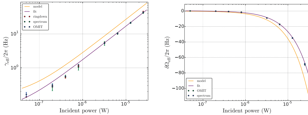
Figure 7.4: Left: Damping rates \gamma_{\text{eff}} obtained by ringdown, spectrum and OMIT measurements for injected powers from 50 nW to 25 \mu W with a red-detuned laser. Error bars indicate the variance of the available 2 – 25 individual measurements with each method at each power. The power dependence from an independent characterization of the system (model) is plotted with a fit of the data. The parameters of the model and fit are shown in Table 7.2. The deviation at low powers can be explained by an incorrect detuning estimation. Right: Effective mechanical resonance frequency shift \delta\Omega_{\text{eff}} = \Omega_{\text{eff}} - \Omega_0 versus injected power for the same measurements and models as in the left plot in linear-logarithmic scale. The unperturbed resonance frequency is \Omega_0/(2\pi) = 3.578313 MHz. Both plots are indistinguishable from a straight line if plotted in linear scale.
