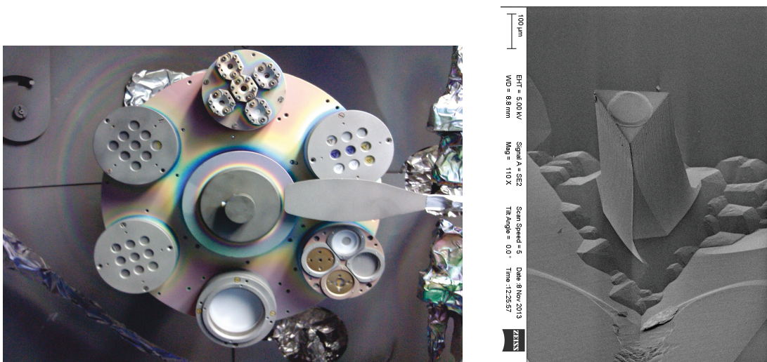
Figure 3.7: Left: Samples mounted inside the SPECTOR machine just before coating the dielectric mirrors. Out of the six circumferentially arranged satellites, the upper right one contains seven micropillar samples with different attempts of mask design. The two left satellites contain nine concave micromirror substrates each. Right: Scanning electron microscope image of a micropillar with a successfully coated mirror. Clearly, no mirror coating is seen on the side faces of the pillar.
