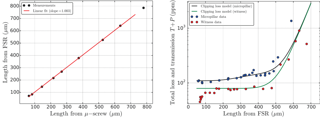
Figure 3.19: Left: Length estimated by the program "finesse.py" versus length estimated by turning a micropositioner screw. The abscissa has an arbitrary offset. Right: Estimated T + P versus cavity length for two cavities, constructed with the same concave coupling mirror (S6-9, T = 35 ppm) and either the quartz witness sample QT2 (large, homogeneous flat mirror, baked out after mirror coating) or the micropillar sample 20121009C4 (without bakeout). The clipping loss model consists in the sum of a loss offset and the clipping loss from a circular aperture at each mirror surface. Both curves assume an equal aperture at the coupler ( 82 \mu\text{m} ) and the independently measured radius of curvature R_c = 900 \mu\text{m} .
