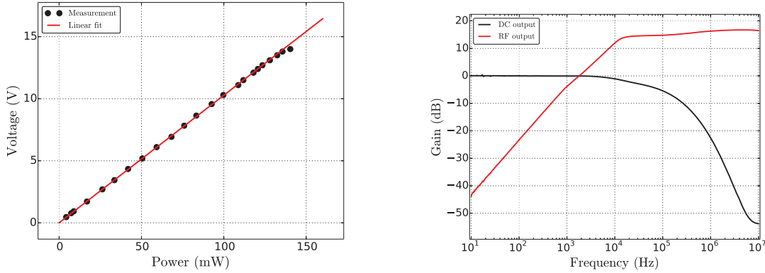
Figure 5.20: Left: Measured DC voltage from a photodiode constructed with a Epitaxx-500 photodiode for different incident powers. The detector voltage is linear up to incident powers of 120 mW, above which it saturates near 14 V, in agreement with the maximum output voltage specification of the amplifier OP27 for a supply voltage of 15 V. Power was further increased up to 330 mW without damaging the photodiode. From the slope of the linear fit, we can deduce a photodiode quantum efficiency \eta_{PD} = 0.77 \pm 0.04 . Right: Measured frequency-dependent gain of the DC and RF photodiode outputs. All gains are normalized to the DC gain at low frequency. The gain was measured by recording the photodiode response to an amplitude-modulation created with an acousto-optic modulator. The RF-output is flat to within 0.5 dB from 1 to 10 MHz. Since the transfer function of the modulator is not necessarily flat, these gain curves can only give an approximate idea of the real transfer functions.
