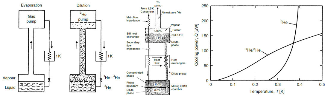
Figure 4.1: Left: Simplified schematics of a ^3\text{He} and a dilution refrigerator. In reality, the concentrated ^3\text{He} phase is lighter and therefore on top of the dilute phase. Middle: More detailed illustration of a dilution refrigerator, showing how a still solves the challenge of pumping on the heavier diluted phase and how good heat exchanger design can lead to reinjection of ^3\text{He} into the mixture chamber at nearly the mixing chamber temperature. Right: Cooling powers of a ^3\text{He} and dilution refrigerator if the same helium pump is used. Figures are taken from [Pob07] (left and middle) and [Lou74] (right).
