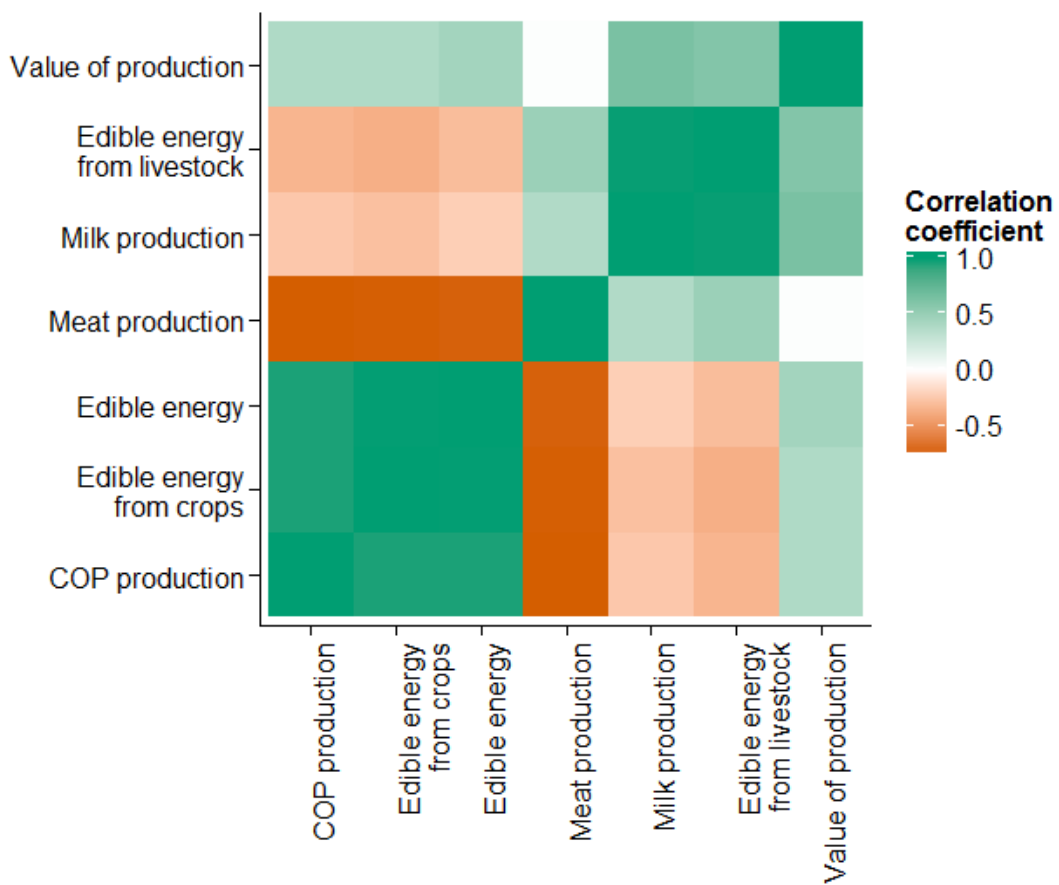
Figure IV-B-2 Pearson correlation coefficients among computed production metrics
