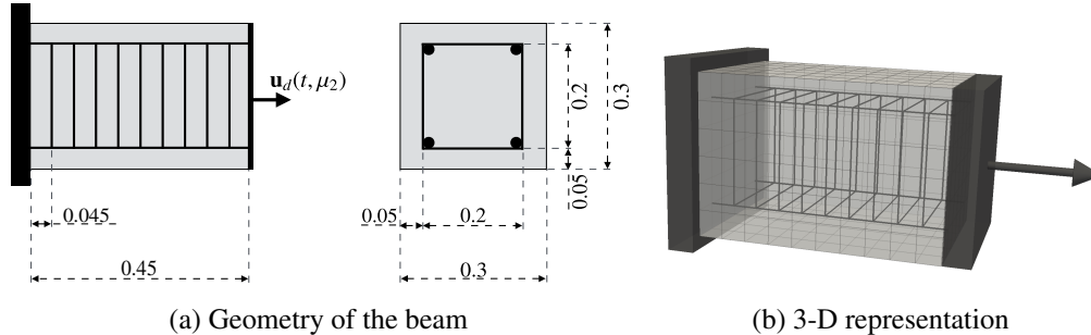
Figure 4.1: Tensile test – geometry (left) and 3-D representation (right) of the beam
