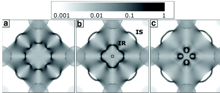
Figure 2.2: Fe (001) k_{\parallel} -resolved minority DOS: Minority DOS of the topmost Fe layer in a Fe/MgO/Fe (001) trilayer for three energies: (a) 0.02eV below E_F (b) at E_F and (c) 0.02eV above E_F . Regular surface states and resonance states are marked IS and IR respectively. Figure reproduced from Belashchenko et al. 72 .
