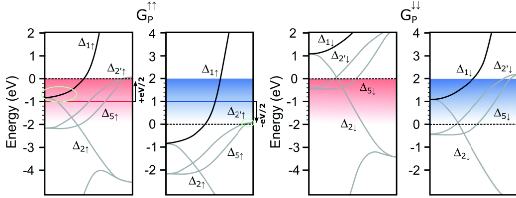
Figure 2.10: Impact of bias voltage related to the band structure of the ferromagnetic leads: Bias window induced by a bias U = 2\text{ V} on the spin- and symmetry-resolved band structure of bcc Fe for the parallel magnetic state and for both spin channels. As the bias is swept, tunneling electrons at E_F in the emitting electrodes probe the density of states of the collecting electrode. Sharp features in the density of state, emphasized by green circles, are expected to have a strong impact on G_P and G_{AP} . See text for a detailed discussion.
