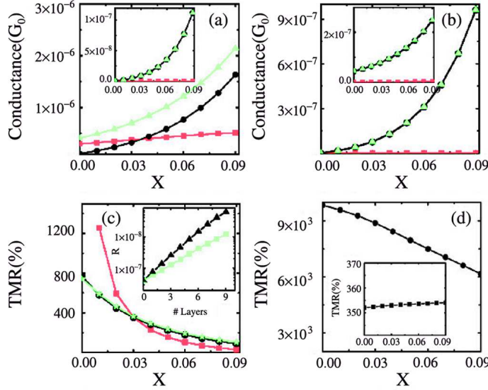
Figure 2.24: Electrical properties of Fe/MgO/Fe MTJs as a function of O vacancy concentration: Panels (a) and (b) plot the conductance for G_P^\uparrow and G_{AP}^\uparrow as a function of oxygen vacancy concentration x , located at the interface layer. 3 % of oxygen vacancies are introduced at the bottom MgO layer and the concentration x is varied in the topmost MgO layers. The coherent (red), vertex correction (black) and total conductance (green) are plotted. Insets represent similar data for G_P^\downarrow and G_{AP}^\downarrow . Panel (c) plots the TMR related to data of panel (a) and (c) for various samples. Panel (d) shows the effect of substituting OV by nitrogen atoms (the large TMR is recovered). The inset of panel (d) shows that TMR is almost independent of oxygen vacancies introduced in the middle of the MgO layer. Reproduced from Ke et al. 159 .
