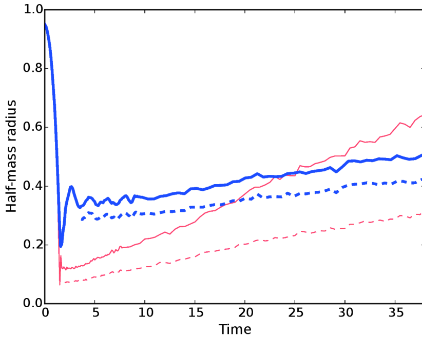
Figure 4.3: Half-mass radius as function of time for two systems undergoing collapse : a uniform-density sphere, Ru20, as the thin red solid curve, and a clumpy Hubble model, Rh20, as the thick blue solid curve. Half-mass radii are in H.u, as well as the time axis, where t_{Henon} = 1\text{unit} = 0.13\text{Myr} . Dashed lines are the half-mass radii of the same systems for the same systems but including only the bound stars.
