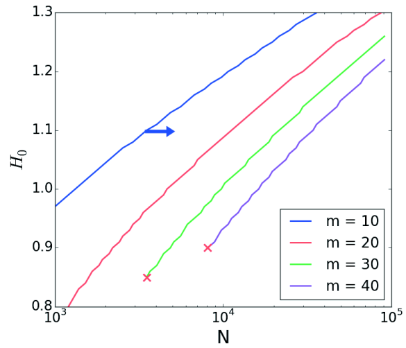
(b) Segregation domains
