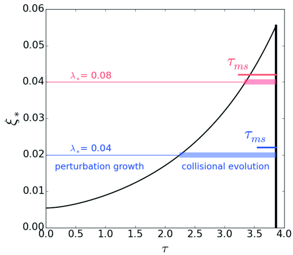
(a) Regimes of overdensity evolution
