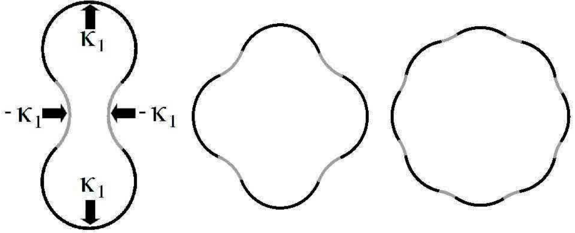
Figure 2.3: Crunching of a circularly closed non-linearly elastic filament for \kappa_0/\kappa_1 = 0.5 . A ground state consists of a sequence of positive and negative curvature regions. All depicted states are ground states and have the same elastic energy
