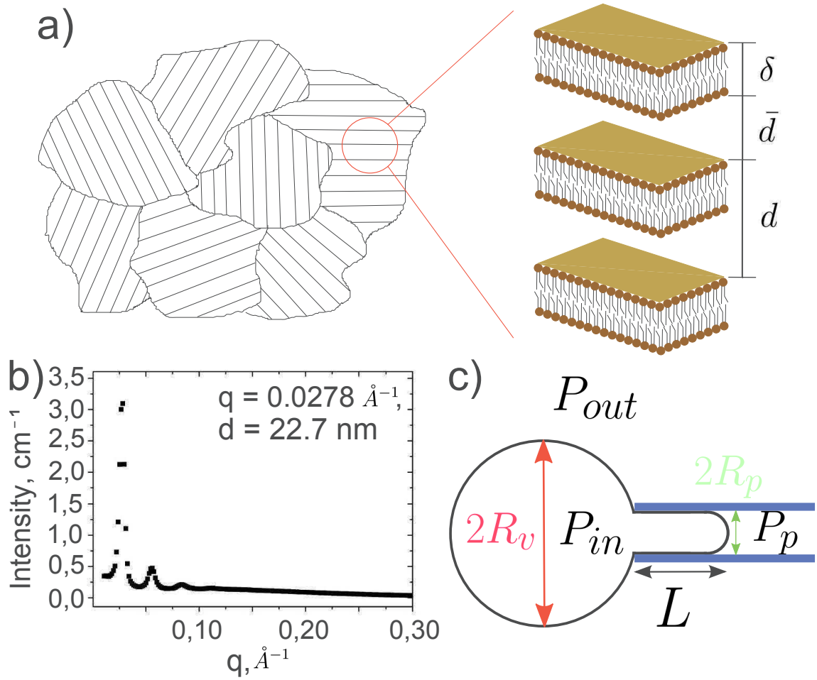
Figure 1.4: Schematic representations of X-Ray (panels (a) and (b)) and micropipette (panel (c)) experiments. (a) Typical X-Ray sample, showing multi-domains lamellar phases (left) and a zoomed view of a lamellar phase (right). (b) Example of plot of intensity scattered by the lamellar phases sample as a function of the wavevector q . Three Bragg peaks are visible, allowing to infer the periodicity of the sample: d = 22,7 \pm 0,4 \text{ nm} [29].
