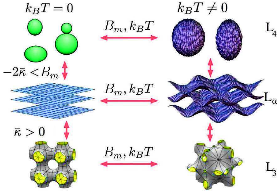
Figure 1.6: Schematic representation of the stability of a lamellar phase at 0 K (left), and at temperature T (right). L_4 , L_\alpha and L_3 respectively correspond to the vesicular, lamellar and sponge phases [41].
