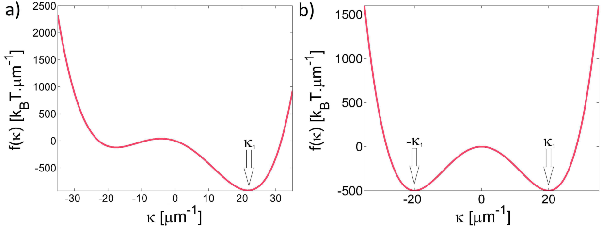
Figure 2.2: Profile of the monomer's energy with respect to the curvature \kappa . For a), the parameters are A = -20k_B T , B = 5k_B T \cdot \mu m and C = 1/160k_B T \cdot \mu m^3 and \kappa_1 \approx 21.76 \mu m^{-1} . For b), the parameters are A = 0k_B T , B = 5k_B T \cdot \mu m and C = 1/160k_B T \cdot \mu m^3 and \kappa_1 = 20 \mu m^{-1} . For a monomer of size a = 10 nm, the barrier is equal to 5k_B T .
