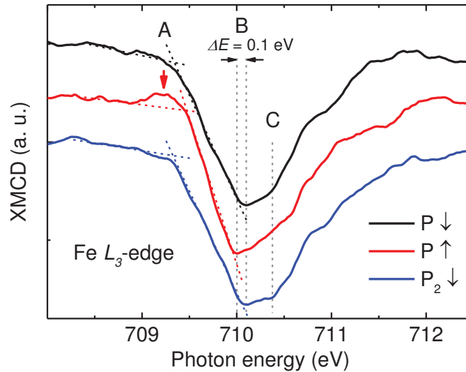
Figure 6.10: Modification of Fe L_3 -edge XMCD upon ferroelectric switching of the device. XMCD at the Fe L_3 -edge of FePc acquired for the consecutive PZT polarization P \downarrow , P \uparrow , and P_2 \downarrow states. Note the features A, B, and C revealing the FE polarization driven changes and identical P \downarrow and P_2 \downarrow spectra. The spectra were acquired in total electron yield mode at both directions of the magnetic field |H| = 0.1 T.
