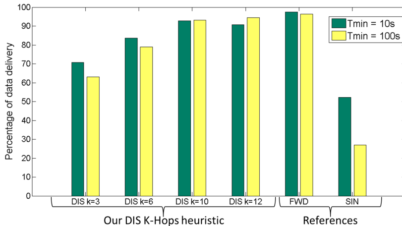
Fig. 3.6 Delivery ratio in a 300-nodes network for different solutions.
