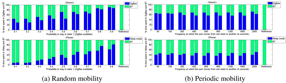
Fig. 6.7 The percentage of time spent by the sensor in Bluetooth and ZigBee, and by the phone in Bluetooth and sleep mode, in function of the user mobility.
