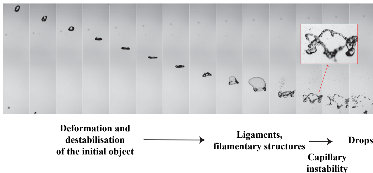
Figure 7.1: Typical sequence of steps involved in a fluid fragmentation process. Water drop falling in an ascending stream of air (modified from Villermaux & Bossa, 2009). The sequence includes deformation of the initial drop which flattens into a pancake shape, formation of liquid ligaments (a toroidal rim collects much of the initial drop mass), destabilization of the rim (highlighted in the inset), leading to disjointed drops distributed in size. Time interval of 4.7 ms, We \approx 600 .
