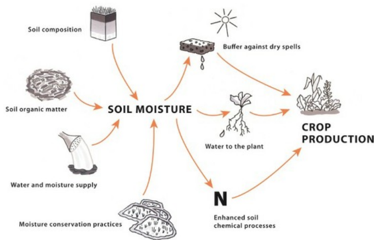
Figure 12: Soil moisture as a system
