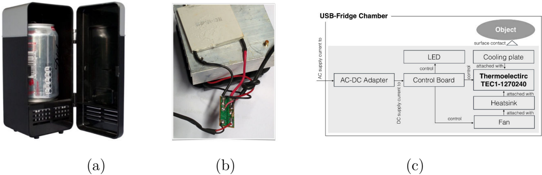
Fig. 6-5 Mini USB-Fridge (a) current product, (b) a simple control board, and (c) a simplified system architecture model
