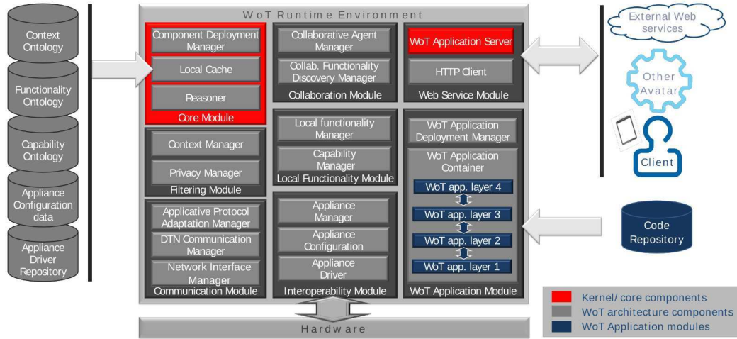
Figure 2.6: Web architecture of avatar agents([ Mrissa et al. 2015 ])
