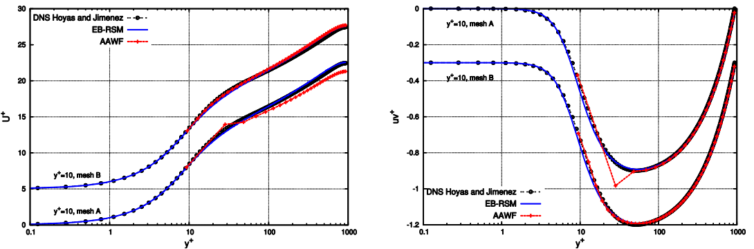
Figure 6 : Illustration of the discretization error introduced in the computation when the mesh is very coarse: when the refined mesh B is used, the kink in the variables vanishes.
