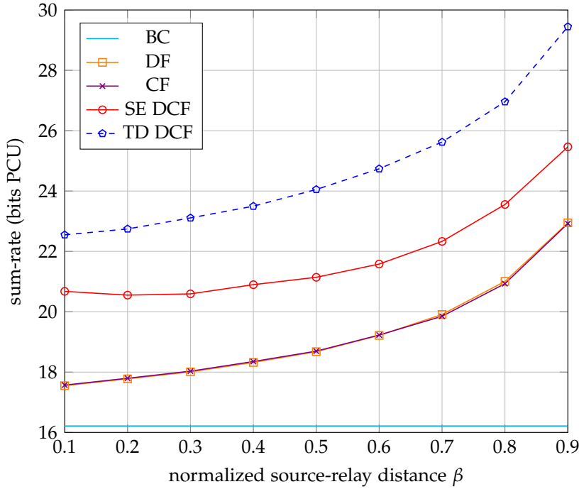
Figure 23: Sum-rate performance of the SE/TD DCF and the baseline schemes (BC/DF/CF) when SNR = 47dB.
