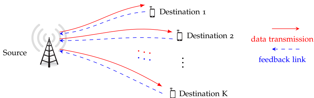
Figure 1: An example of homogeneous feedback
