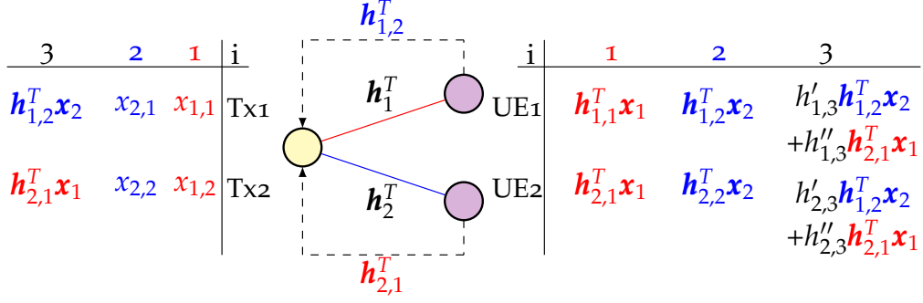
Figure 5: Example of MAT scheme.
