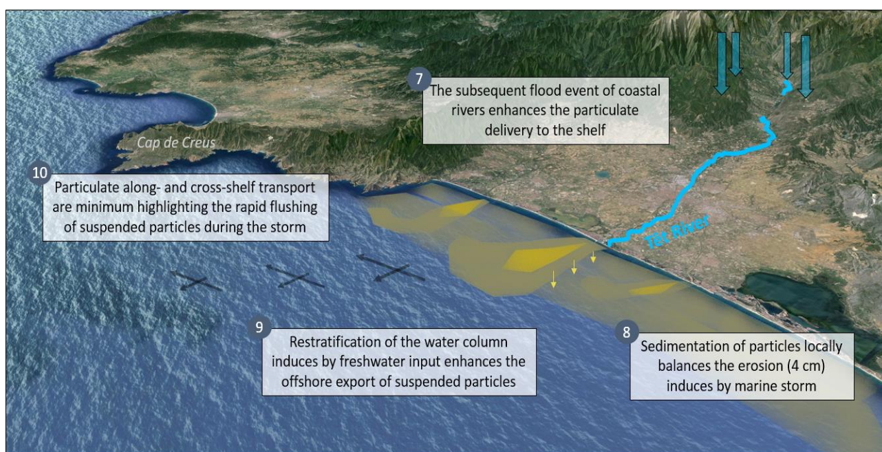
Figure 7.3 : Graphical abstract of the impact of a "back-to-back" storm and flood event on SPM dynamics over the SW part of the shelf of the GoL. View is from the NE.
