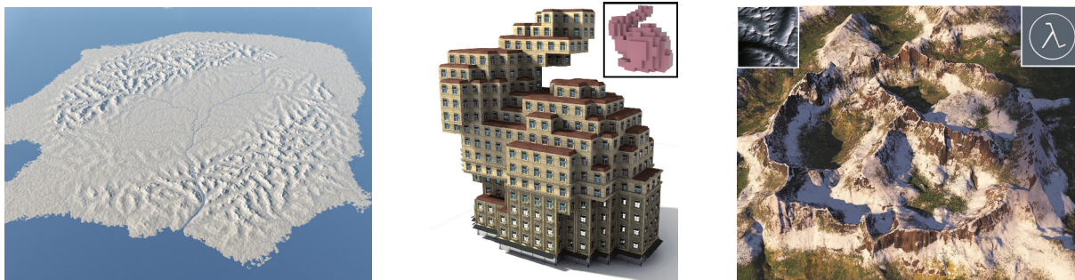
(a) Terrain procedurally generated by Génevaux et al. (2013) using hydrological principles.
