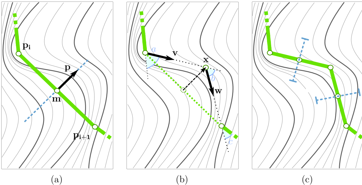
Figure 4.6 – Recursive subdivision process for waterfall network segments: (a) The segment [p_i, p_{i+1}] is subdivided at its middle m , which is moved along perpendicular direction p . (b) The final position x is the point that minimizes our cost function C(x) . (c) The process is iterated until segments are smaller than the threshold l .
