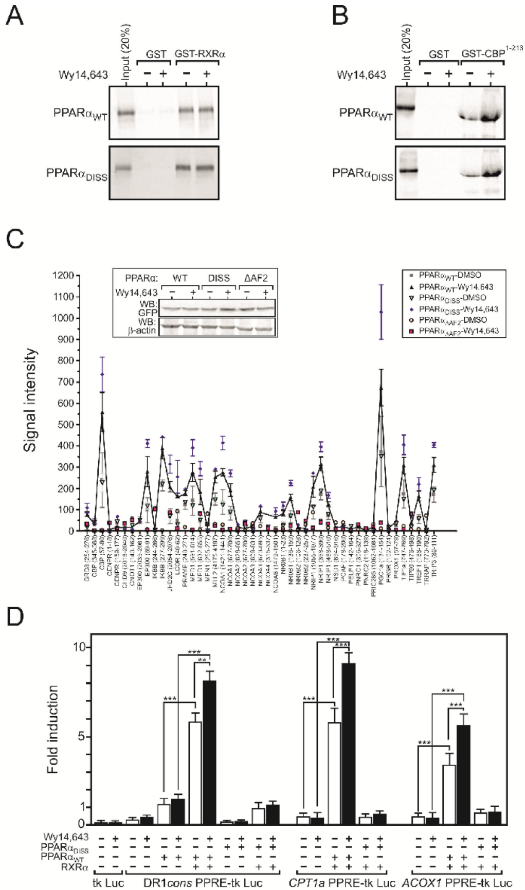
Figure 2. Structural integrity of the PPAR \alpha DISS mutant.
