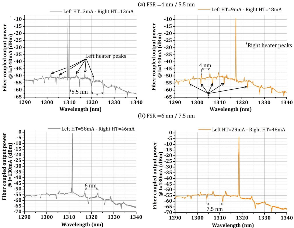
Figure C-37: Spectra for two SGDBR lasers with their mirrors having different FSR: (a) FSR_{left}=4 \text{ nm} / FSR_{right}=5.5 \text{ nm} , (b) FSR_{left}=6 \text{ nm} / FSR_{right}=7.5 \text{ nm} .
