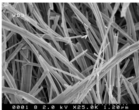
(A) Palygorskite
