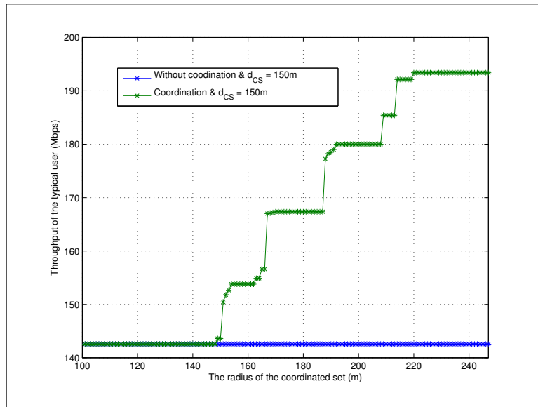
Figure 5.4: Throughput vs d_{CS} , for d = 150\text{m} , radius of the coordinated set.
