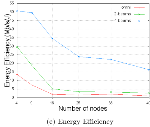
Figure 9.7: N-Sources/1-Destination - Grid topology (vs Number of nodes).
