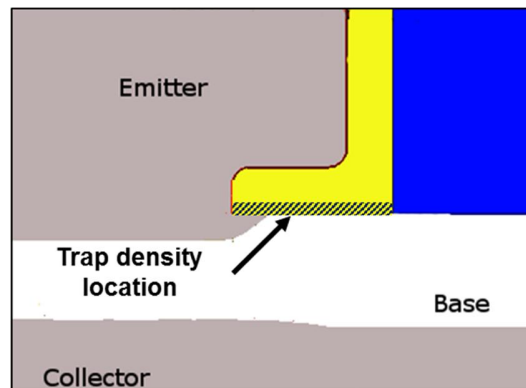
Figure 67 Trap location impacting the forward Gummel plot
