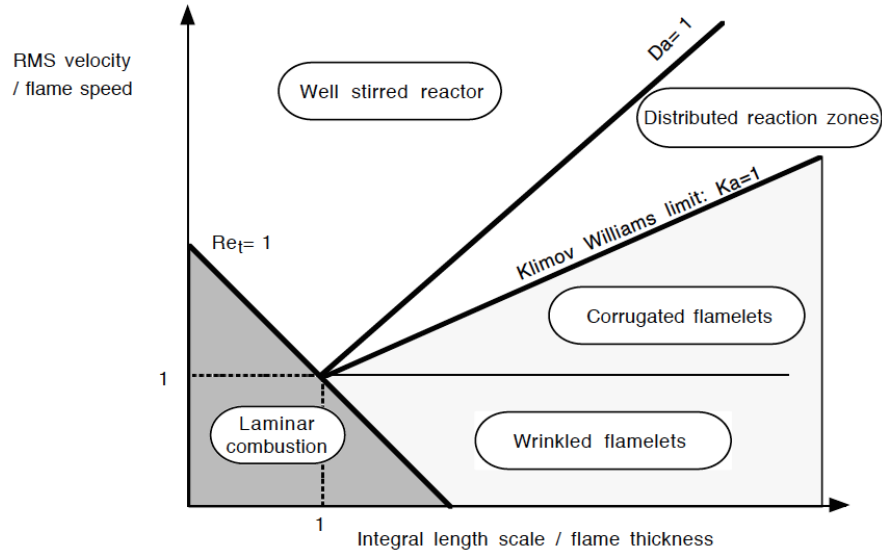
Figure 2.2: Turbulent premixed combustion diagram: combustion regimes are identified in terms of length ( \ell_t/\delta_L^0 ) and velocity ( u'/S_L ) ratios using a log-log scale (Poinso and Veynante 2011).
