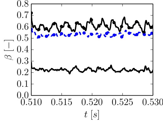
Figure 6.8: Temporal evolution of the global parameter \beta(t) ( \text{--}\bullet\text{--} ), local average model parameter \bar{\beta}(t) , Eq. 6.18 ( \text{--}\bullet\text{--} ) and its fluctuation \beta'(t) , Eq. 6.19 ( \text{—} ).
