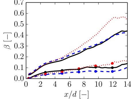
Figure 5.12: Spatial evolution of \beta_{avg}^s(x) (no symbols) and \beta_{rms}^s(x) (symbols) for simulations varying test and averaging filter widths. (—) L_{3.0\Delta}^{1.5\Delta} ; (---) L_{6.0\Delta}^{1.5\Delta} ; (···) L_{3.0\Delta}^{3.0\Delta} .
