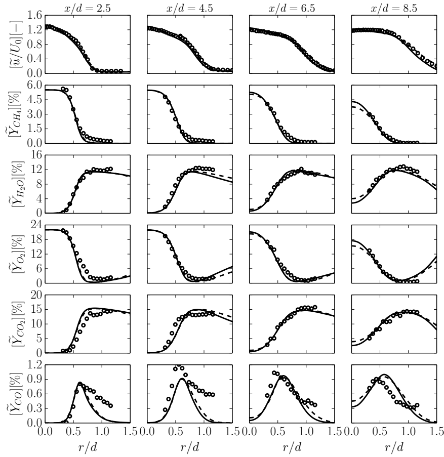
Figure 5.7: Transverse profiles of mean axial velocity and species mass fractions for four downstream locations obtained with the coarse and fine meshes. (o) Experiments (Chen et al. 1996); (—) L^{1.5}_{3.0\Delta} with coarse mesh; (---) L^{1.5}_{3.0\Delta} with fine mesh.
