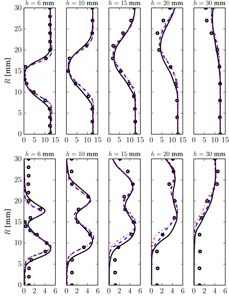
Figure 6.5: Favre mean (top) and resolved RMS (bottom) \text{CO}_2 [%] transverse mass fraction profiles at five downstream locations. ( \circ ): Favre measurements; ( \text{—} ) L_{0.83} ; ( \text{-- --} ) G_{0.83} ; ( \text{-} \cdot \text{-} ) C_{0.83} .
