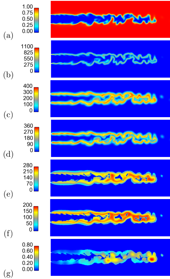
Figure 5.3: Instantaneous LES resolved fields and corresponding test-filtered quantities for the F3 flame. (a) \tilde{c} ; (b) |\nabla \tilde{c}| ; (c) |\widehat{\nabla \tilde{c}}| ; (d) |\nabla \tilde{c}| ; (e) \langle |\widehat{\nabla \tilde{c}}| \rangle ; (f) \langle |\nabla \tilde{c}| \rangle ; (g) \beta -field. Snapshots corresponds to simulation L_{3,0\Delta}^{1.5\Delta} .
