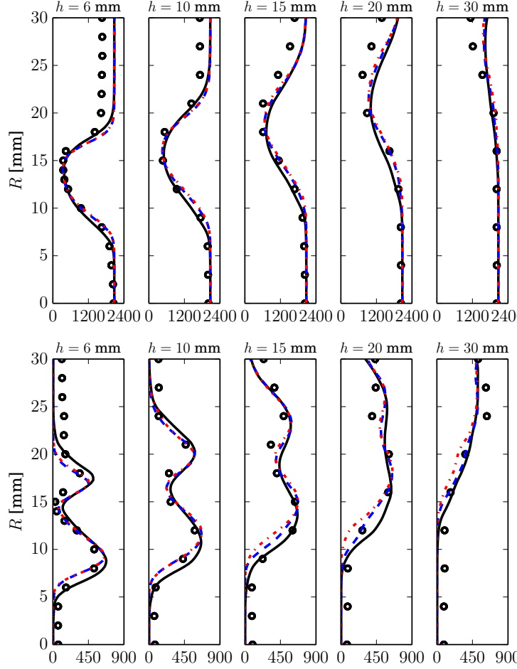
Figure 6.6: Favre mean (top) and resolved RMS (bottom) temperature T [K] transverse profiles at five downstream locations. ( \circ ): Favre measurements; (—) L_{0.83} ; (---) G_{0.83} ; (-.-) C_{0.83} .
