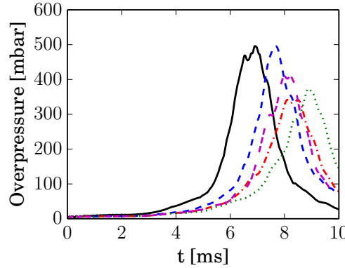
Figure 7.8: Comparison of overpressure signals for different simulations: (—) 2D-DNS1; (— — —) 2D-LES2 (TTGC, \delta_c = \delta_L^0 , adapted transport coefficients), (- · - ·) 2D-LES5 ( \delta_c = 2\delta_L^0 ); (····) 2D-LES6 (non-adapted transport coefficients), (- - - -) 2D-LES7 (LW).
