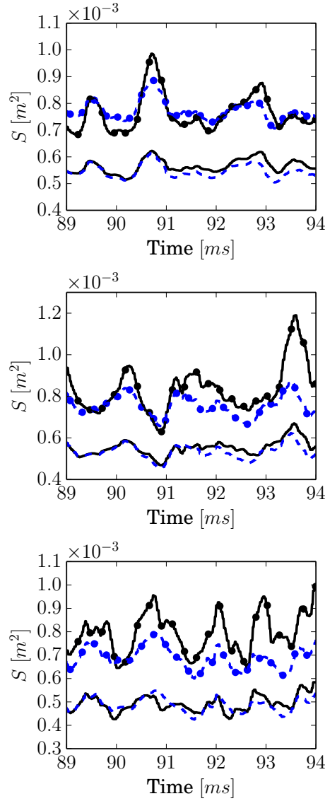
Figure 5.11: Temporal evolution of the resolved ( S_r(x_0, t) , no symbols) and total ( S_t(x_0, t) , symbols) flame surfaces at different locations: x_0 = 4.5d (top); x_0 = 6.5d (middle) and x_0 = 8.5d (bottom). The thickness of the volume slice is 12 mm. (—) L_{3.0\Delta}^{1.5\Delta} ; (—) G^{1.5\Delta} .
