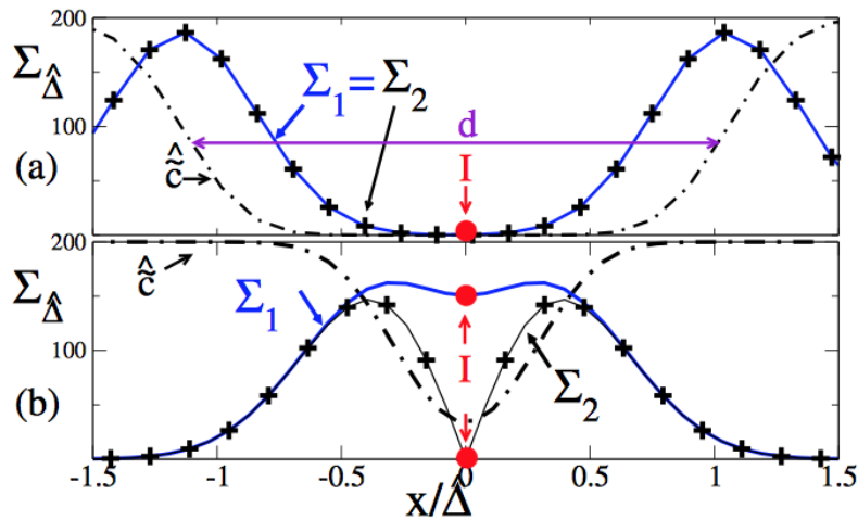
Figure 4.10: Two interacting one-dimensional planar flame fronts at a distance d . (a) d > \hat{\Delta} (b) d < \hat{\Delta} . \Sigma_1 = |\nabla \hat{c}| ; \Sigma_2 = |\nabla \hat{c}| (Mouriaux et al. 2016).
