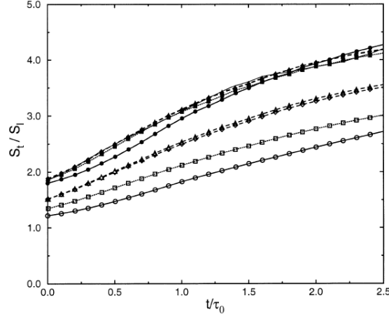
Figure 4.1: Time evolution of the turbulent flame speed. Time is made non-dimensional by the initial turbulent eddy turn-over-time \tau_0 . Thick solid line: DNS; \bullet, \circ \mathcal{F} = 6.6 ; \blacksquare, \square \mathcal{F} = 4.0 ; \blacklozenge, \diamond , \mathcal{F} = 2.8 - \gamma = 2 ; \blacktriangle, \triangle \mathcal{F} = 2.8 - \gamma = 3 . The empty symbols are for the resolved turbulent speed (computing the reaction rate without wrinkling factor), plain symbols are for the total turbulent speed (with wrinkling factor) (Charlette et al. 2002b).
