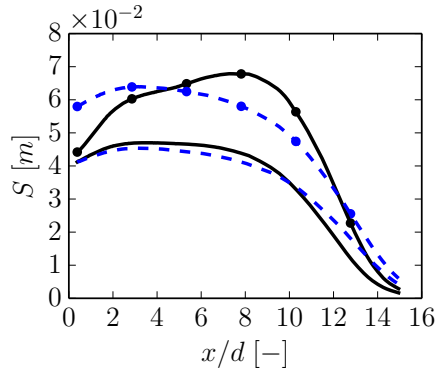
Figure 5.10: Spatial evolution of resolved ( S_r(x) , no symbols) and total ( S_t(x) , symbols) flame surfaces for local (—, case L_{3.0\Delta}^{1.5\Delta} ) and global (---, case G^{1.5\Delta} ) formalisms.
