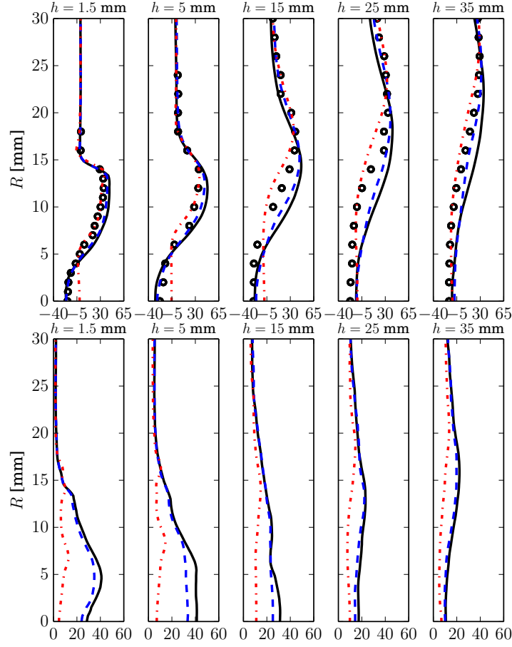
Figure 6.16: Favre mean (top) and resolved RMS (bottom) transverse axial velocity [m/s] profiles. (o): Favre measurements; (—) L_{0.70} ; (---) G_{0.70} ; (···) C_{0.70} .
