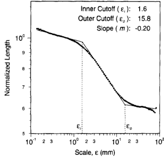
Figure 3.4: Normalized length as a function of scale for average of 366 images for the \text{CH}_4/\text{air} flame at \phi = 0.7 , mean bulk velocity \bar{u} = 5 \text{ m/s} and u'/S_L = 1.22 . Best-fit three linear segments are shown along with slope and inner and outer cut-offs (Smallwood et al. 1995).
