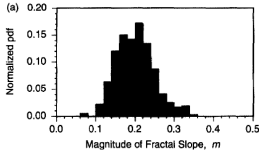
Figure 3.5: Histogram of the magnitude of fractal slope from 366 individual flame images for the \text{CH}_4/\text{air} flame at \phi = 0.7 , mean bulk velocity \bar{u} = 5 \text{ m/s} and u'/S_L = 1.22 (Smallwood et al. 1995).
