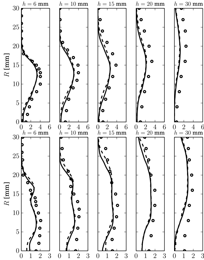
Figure 6.21: Favre mean (top) and resolved RMS (bottom) CH_4 [%] transverse mass fraction profiles at five downstream locations. ( \circ ): Favre measurements; (—) standard mesh; (---) fine mesh
