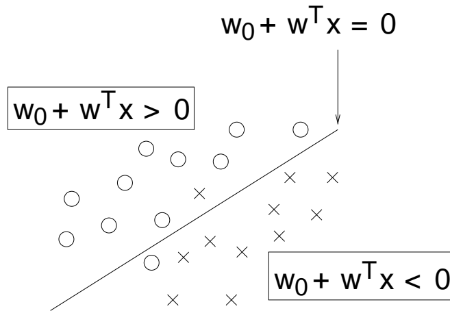
Figure 1.7: Hyper-plane separating two classes. The "crosses" and the "circles" [Lotte, 2008]
