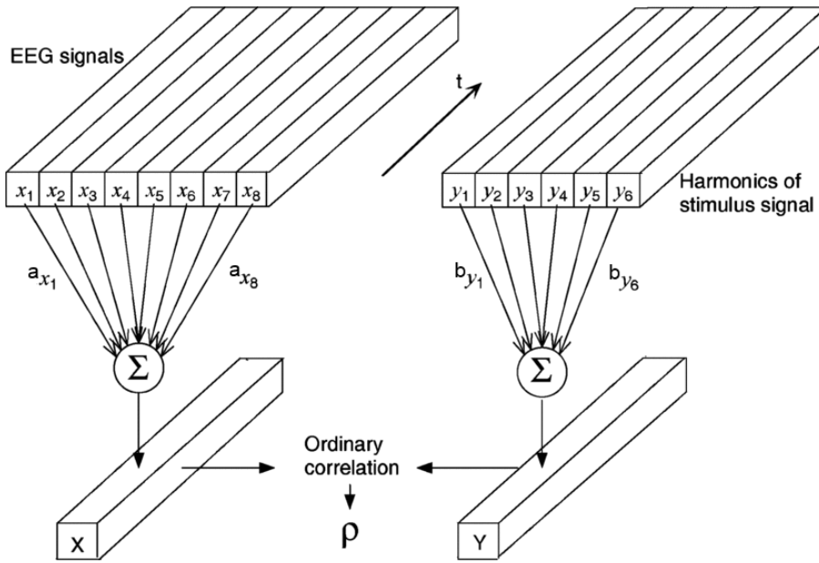
Figure A.1: CCA use for EEG signal analysis [Friman et al., 2001]. The signals x_1, x_2 , etc. are compared to the reference signals y_1, y_2 , etc. (typically the harmonics of the stimulus signal for SSVEP classification), producing a single correlation measure p .
