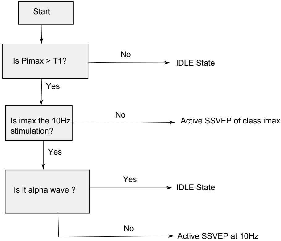
Figure A.5: Idle state detection Pipeline: For each frequency of stimulation i , CCA values P_i are computed. Let imax be the frequency maximizing P_i . When P_{imax} passes a pre-defined threshold T_1 , the corresponding SSVEP activation is detected. 10Hz detection is an exception, and an additional alpha wave detection is performed for reducing false positives.
