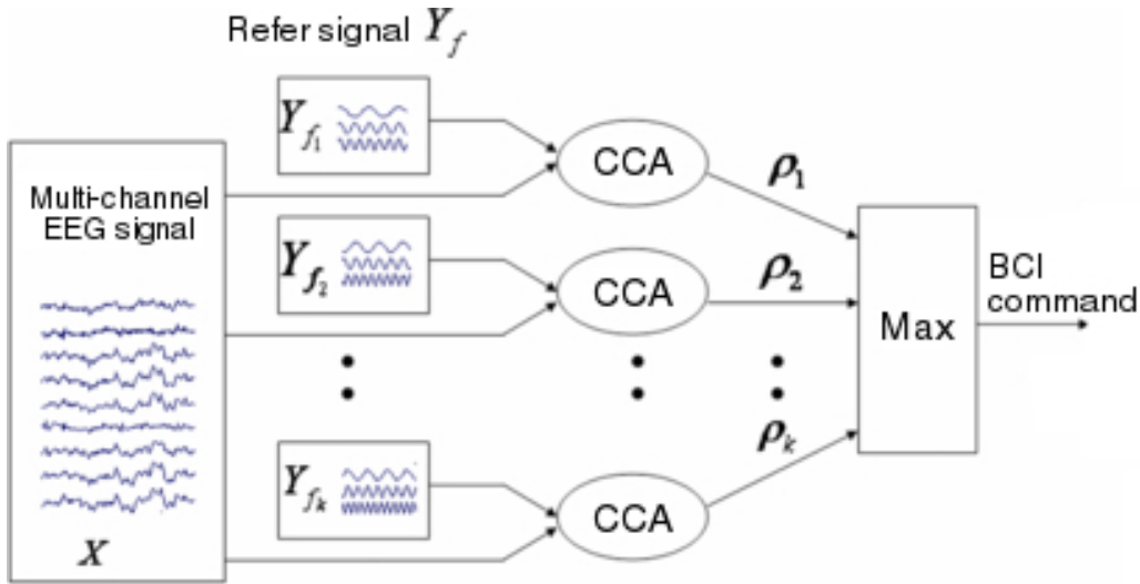
Figure A.2: Description of CCA-based pipeline for segmentation-paced classification, with with k targets, as described by [Bin et al., 2009]
