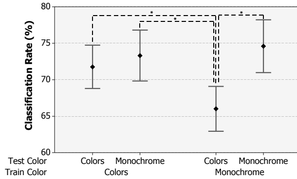
Figure 5.3: Classifier accuracy (CI 95%) depending on the training and testing color. Left: classifiers trained with colored targets tested on colored and monochrome targets. Right: classifiers trained with monochrome targets tested on colored and monochrome targets.
