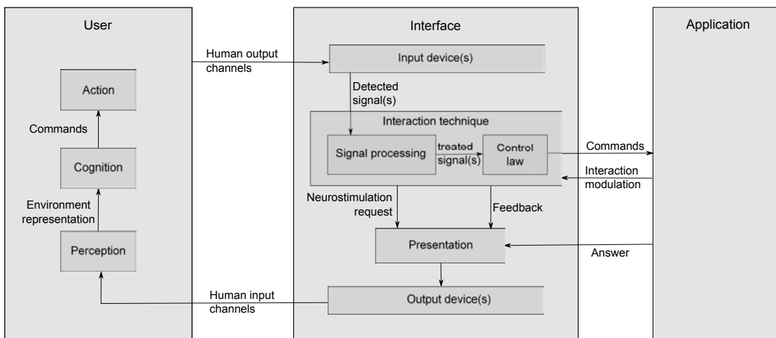
Figure 3: BCI-based interaction loop: A more detailed description of the Human-Computer Interaction loop, emphasizing the components of interest for BCI-based interaction. The user model can be decomposed into perception, cognition, and action processes. Input devices measure human activity, including cerebral activity. This measure is then processed and interpreted into a command. The application receives the generated command and produces an appropriate response. Output devices provide the required neurostimulation, the feedback from the interface, and the response from the application.
