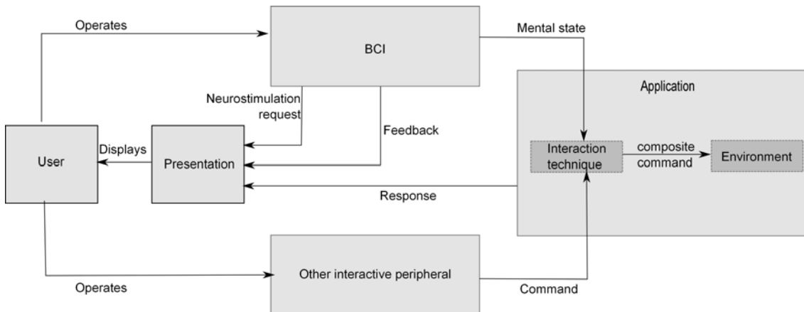
Figure 2.5: Hybrid interaction with a BCI: One or more other complementary interaction devices are used simultaneously to accomplish a more complex interactive task
