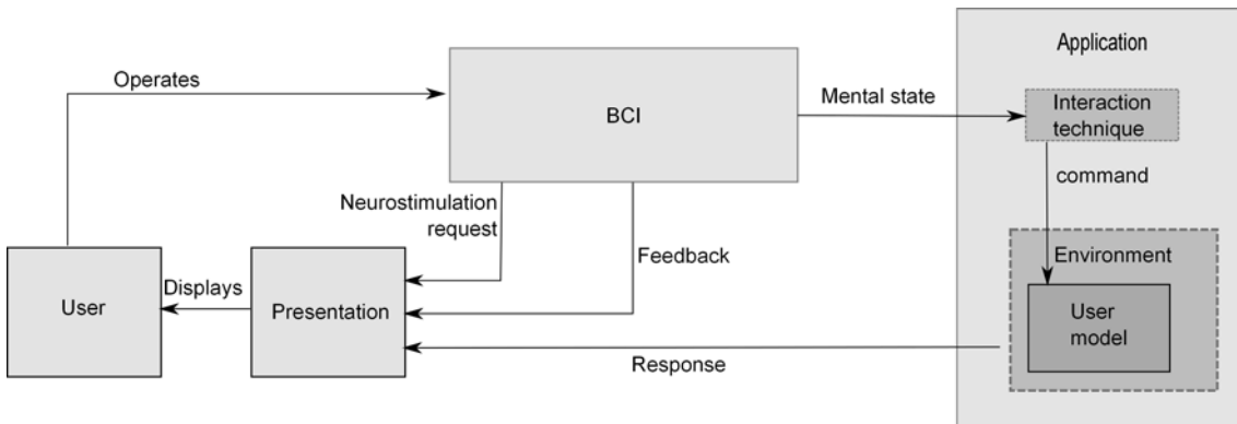
Figure 2.7: Passive BCI: The user does not send an explicit command, but the application can construct a model of the user based on his or her mental state
