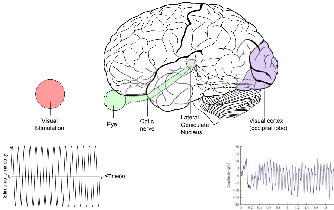
Figure 1.13: A visual stimulation is sent to the eye, with a periodic variation of luminosity, e.g. at 15 Hz (left plot). This signal is perceived and transmitted via the optic nerve, toward the visual cortex (located in the occipital lobe). The response in the resulting cerebral activity presents an enhanced 15 Hz component, called SSVEP (right plot). The cerebral response plot presented here is from [Zhu et al., 2010b]. The rest of this figure is original content.
