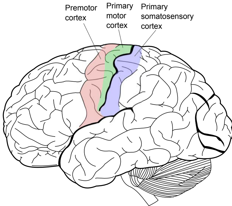
Figure 1.11: Motor and sensorimotor cortical areas
