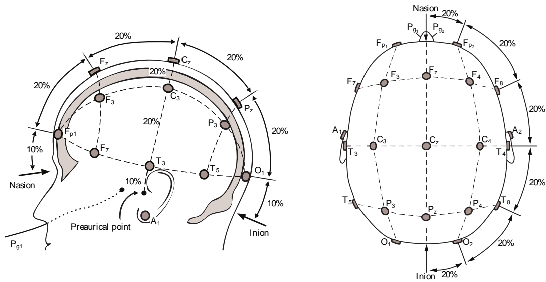
Figure 1.3: Electrodes placement according to the international 10-20 system [Tanner, 2011]. Left: Sagittal view. Right: Axial view
