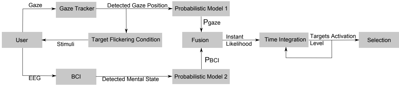
Figure 6.1: Schematic diagram of simultaneous processing for the proposed hybrid interaction technique based on the fusion of gaze and EEG inputs
