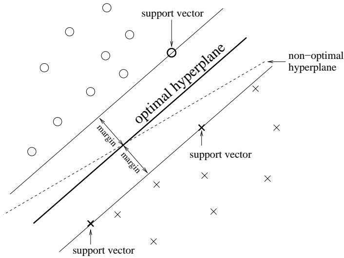
Figure 1.8: Hyper-plane computed from an LDA separating two classes. The "crosses" and the "circles", respecting SVM constraint [Lotte, 2008]
