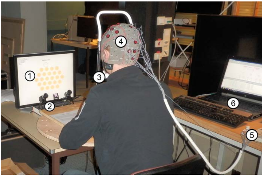
Figure 6.2: Experimental setup. 1: Visual display. 2: Gaze tracker. 3: Chin rest. 4: EEG headset. 5: EEG signal amplifier. 6: Laptop with OpenViBE software for EEG signal processing.
