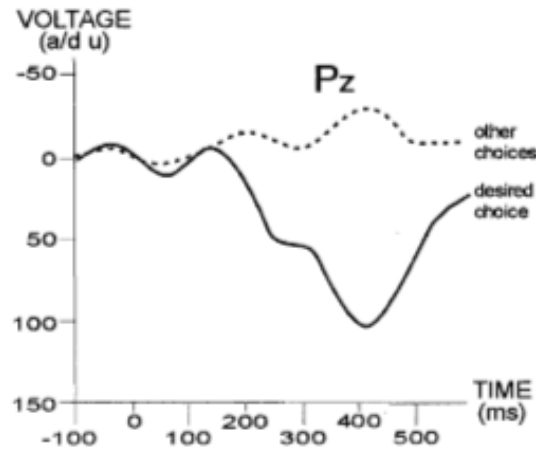
Figure 1.9: P300 potential, averaged over several presentations of the desired stimulus, and of other stimulus [Wolpaw et al., 2002]
