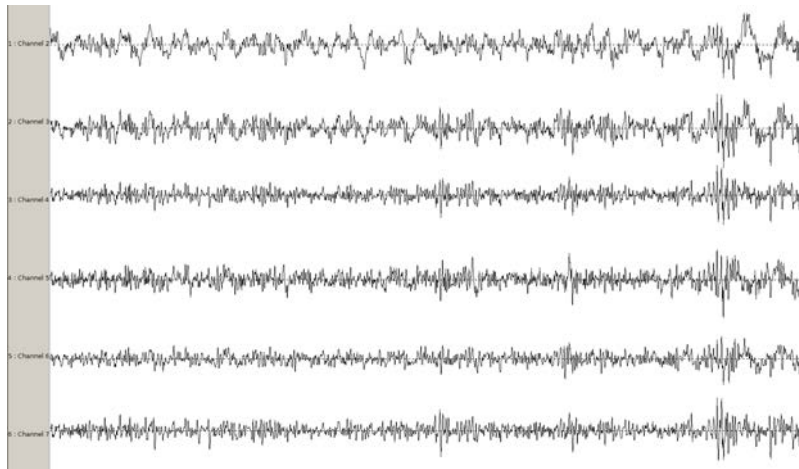
Figure 1.5: Temporal evolution of a typical EEG signal. Each line represents one channel.
