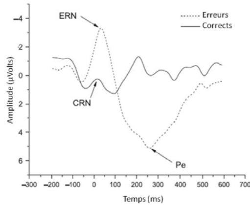
Figure 1.12: Average cerebral answer to trials for correct answers (full line) and incorrect (dotted lines) [Perrin, 2012]
