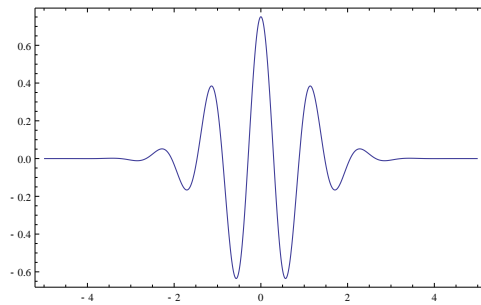
Figure 1.6: Shape of a typical wavelet signal: the Morlet Wavelet 6
