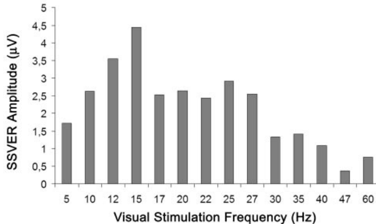
Figure 1.16: Amplitude of SSVEP response, as a function of the stimulation frequency [Pastor et al., 2003]
