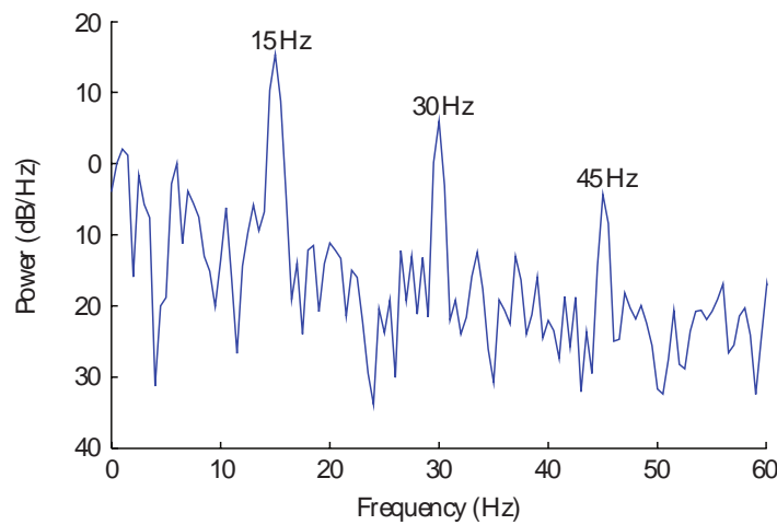
Figure 1.14: Frequency spectrum in visual areas during presentation of a 15Hz flickering stimulus [Zhu et al., 2010b]
