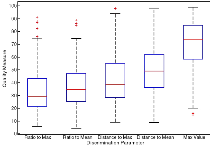
Figure A.3: Box plot of the quality measure for several discrimination features
