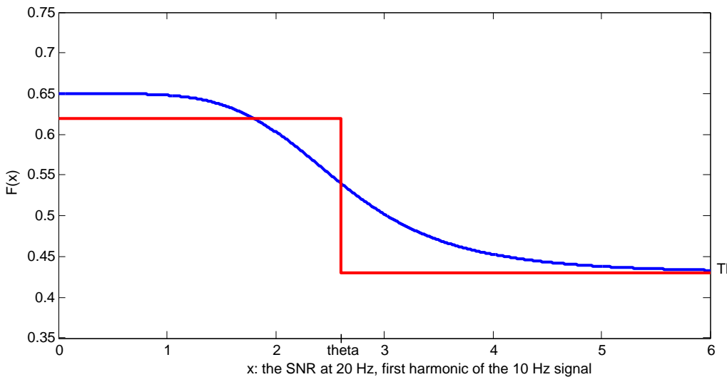
Figure A.6: Decision frontiers: the step function (red) and the sigmoid (blue)
