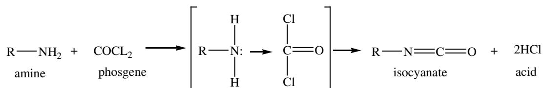
Scheme 2.6 The method of producing isocyanate [39].
