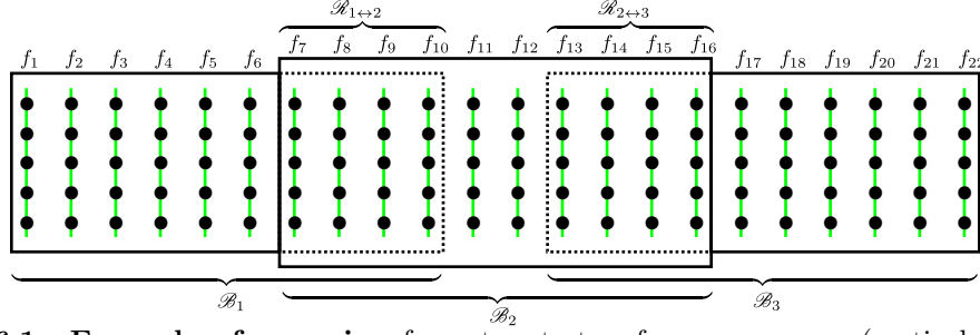
Figure 6.1: Example of grouping for a twenty-two frames sequence (vertical segments) containing five points each (black disks). Here frames are grouped into three chunks of ten frames each, with four frames overlap.
