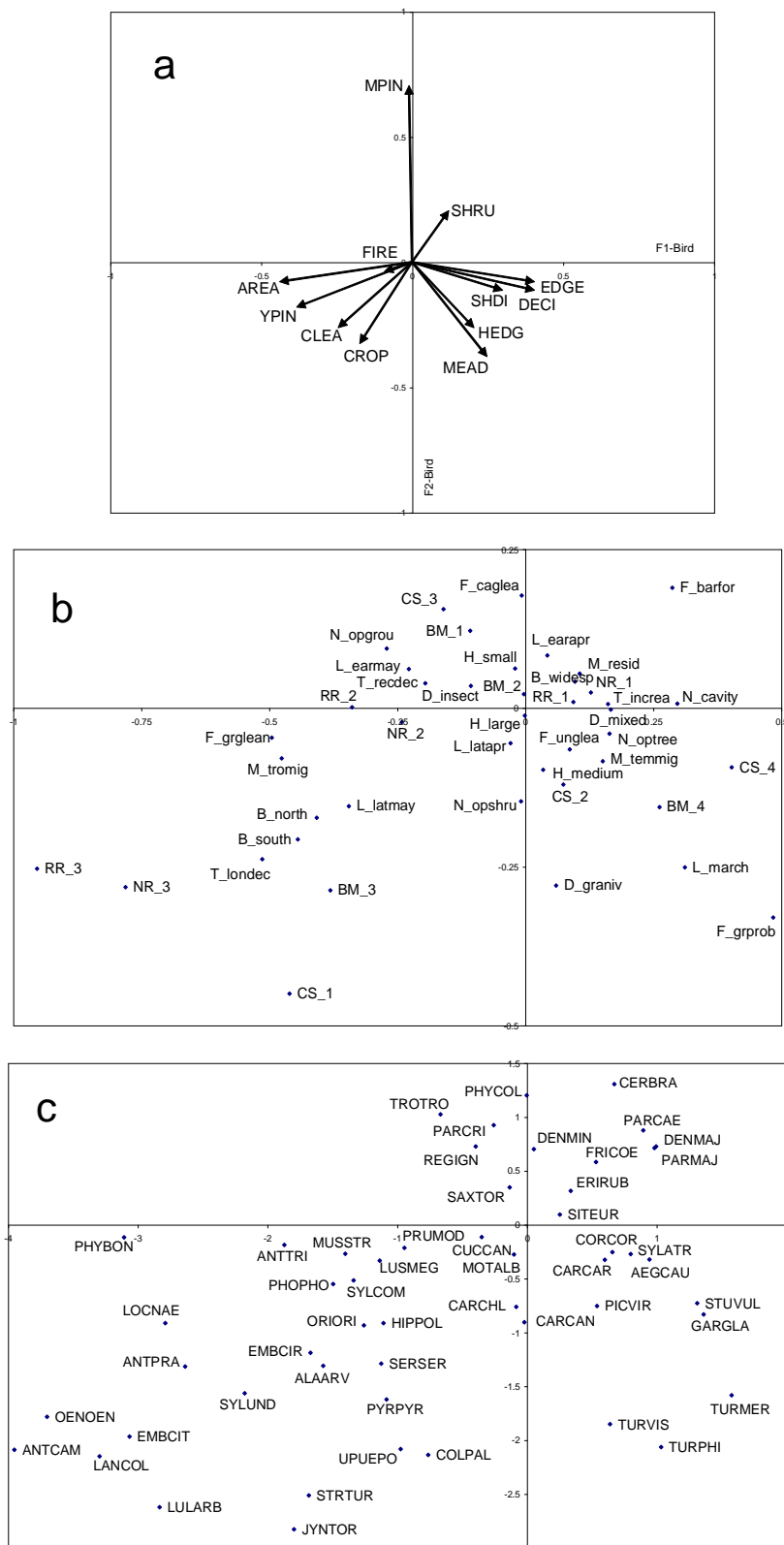
Fig. 2 Graphical display of RLQ scores of (a) landscape variables, (b) life traits categories and (c) bird species. See Annex A for the codes of life traits and Table 2 for landscape variables. Abbreviations of bird species names use the first three letters of genus and species scientific names, e.g. PHYBON = Phylloscopus bonelli .
