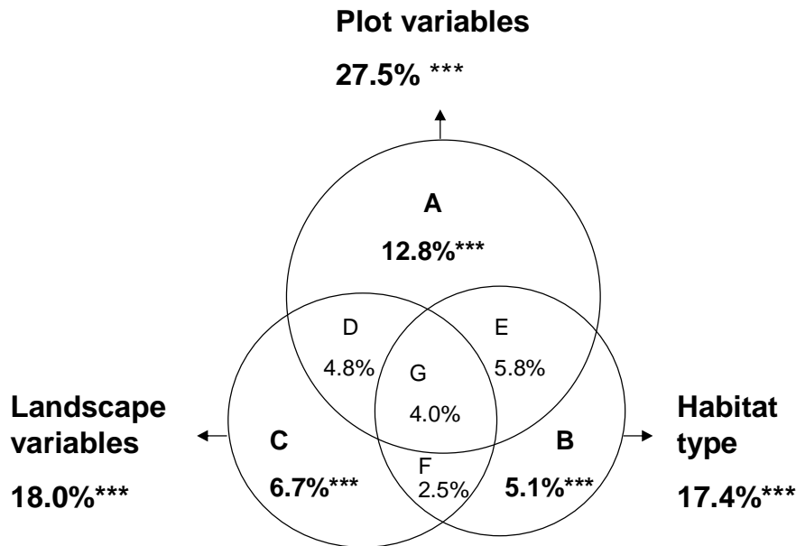
Figure 9. Decomposition of the variance in butterfly community structure explained by plot variables, habitat type and landscape variables in independent and confounded effects using several partial CCA's. Parts A, B and C represent the independent effects of plot, habitat and landscape variables, respectively; parts D, E, F and G indicate the joint effects. Significance levels are based on 999 Monte Carlo permutations: *** P=0.001 . The area of each circle is proportional to the variance explained by that group of variables. The total variance explained by the three sets of variables is 41.7 %.
