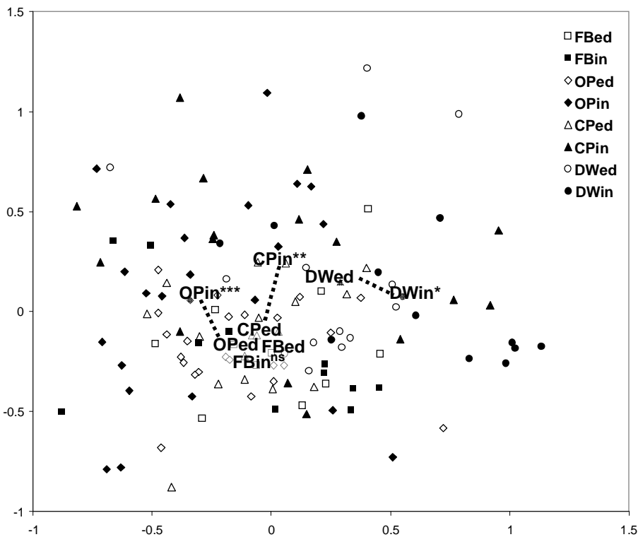
Figure 5. NMDS ordination plot based on Bray-Curtis distances. Each point represents an edge habitat (open symbols) or interior habitat (closed symbols). The position of the names of the habitat types indicates the centre of all plots of the corresponding type. Pairwise differences between edge and interior habitats per habitat type were tested with MRPP (* P<0.05 ; ** P<0.01 ; *** P<0.001 , ns not significant). FBed – firebreak edges, FBin – firebreak interiors, OPed - open pine stand edges, OPin – open pine stand interiors, CPed – closed pine stand edges, CPin – closed pine stand interiors, DWed - deciduous woodland edges, DWin – deciduous woodland interiors. Two-dimension stress = 0.27.
