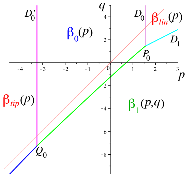
Figure 3.5: Respective domains of validity of integral means spectra \beta_{tip}(p) , \beta_0(p) , \beta_{lin}(p) , and \beta_1(p, q) . The thin straight line (coral) q = 2p corresponds to the version of whole-plane SLE studied in Ref. [2]. It does not intersect the lower domain where \beta_1 holds.
