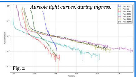
The aureole of Venus is the faint, thin light surrounding the planet disk, visible against the dark sky background. It is due to the refraction of sunlight in the mesosphere of the planet.
