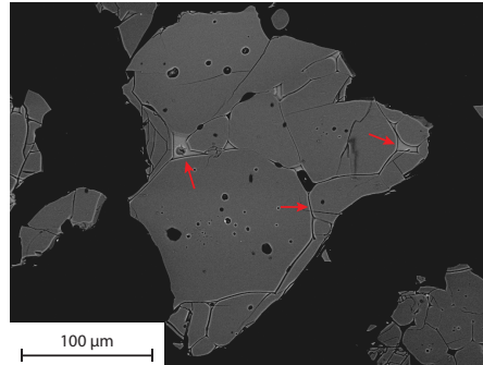
Figure 2.10 – SEM image of sample 0PR-PC6 showing melt present at grain boundaries and triple junctions (red arrows).
