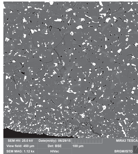
(b) Sample H_2O -sat.-PC19 run at 1250 °C, 1.5 GPa with hematite as pressure medium
