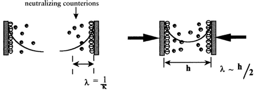
Figure 2.3: Schematic of counterion layer formation near charged surfaces, from [12]. The surfaces begin to interact electrostatically when their separation, h , becomes similar to twice the Debye length, \lambda .
