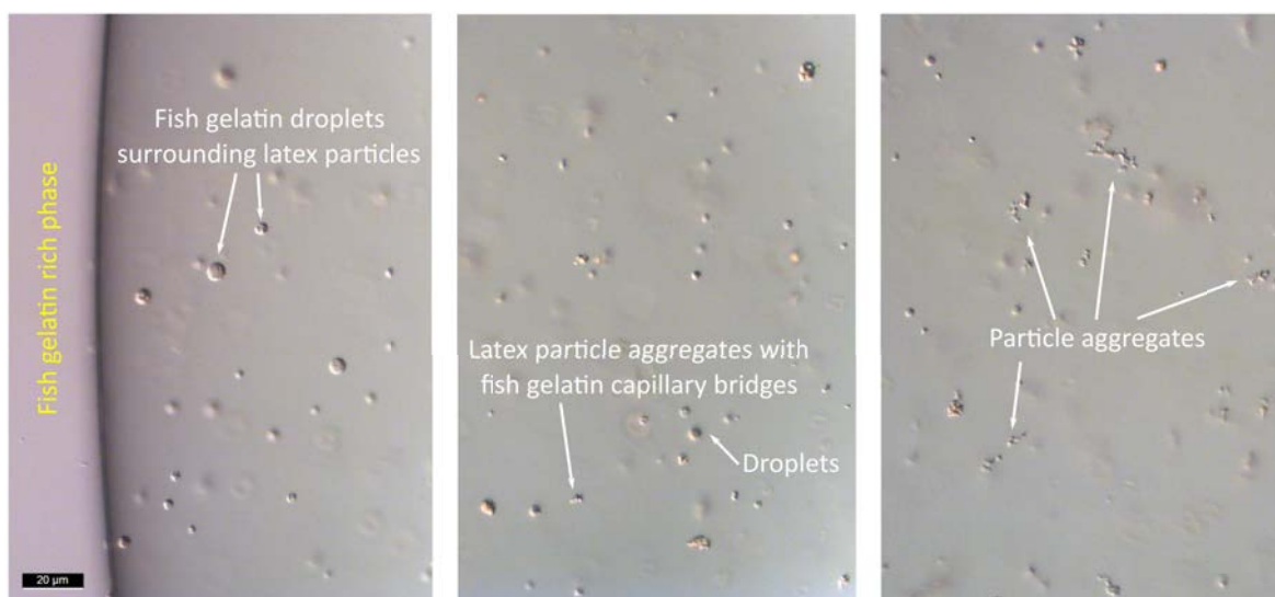
Figure 8.5: 200nm Carboxylate-functionalised latex particles dispersed in 20% dextran solution, close to the interface with a 20% fish gelatin solution, within a sample cell as described in Section 7.2.3. Sample aged for 24 hours. Left: At interface, diffusion of fish gelatin through sample causes nucleation of droplets of fish gelatin around particles. Centre: 1mm from interface, transition zone from nucleated droplets to capillary-bridged aggregates. Right: 2mm from interface, disparate aggregates connected with capillary bridges of diffused gelatin.
