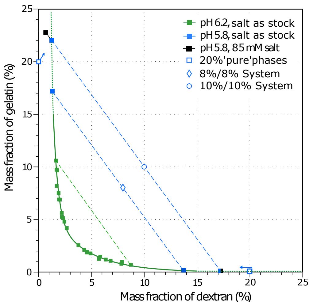
Figure 7.5: Extrapolation of published data by Vis et al. [109] to larger polymer concentration. Solid lines represent published phase diagram positions, dotted lines extrapolated positions. Tie-lines between phases in equilibrium are shown as dashed lines. The green pH6.2 system represents the published unadjusted stock salt concentration system. This is extrapolated to include the 8% / 8% fish gelatin / dextran , and 10% / 10% fish gelatin / dextran systems studied, with the points shown in blue, with the starting points of the systems shown as an open blue diamond and circle respectively. The addition of salt to the 10% / 10% fish gelatin / dextran system, shown as the black squares, results in an increase of the tie line length along the same tie line. The position along the tie line of the high-salt points are measured through IR Spectroscopy. When creating a 10%/10% system by mixing equal volumes of 20% polymer, the initial phase diagram position is indicated by the unfilled blue squares. The system will equilibrate through water and polymer diffusion till the filled blue squares are reached.
