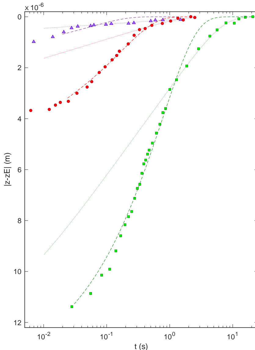
Figure 10.12: Fitting of Equations 10.4 (dotted lines) and 10.1 (dashed lines) for 1\ \mu\text{m} , 4\ \mu\text{m} and 12\ \mu\text{m} Sulphate Latex particles adsorbing to the dextran / fish gelatin interface, shown by purple triangles, Red circles and green squares respectively.
