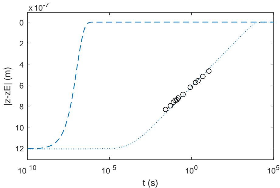
Figure 10.11: Fitting of Equation 10.4 (dotted line) to the data of Kaz et al. tracking the adsorption of a 1.8\ \mu\text{m} diameter Sulphate latex particle (black circles, from Figure 3a of Reference [62]), using parameters specified in [21]. The exponential regime, given by Equation 10.1 is shown as the dashed line, however only logarithmic behaviour is observed in this trajectory.
