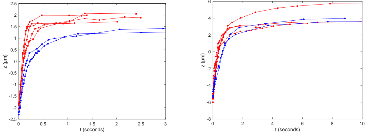
(a) 4 \mu\text{m} Sulphate latex particles adsorbing to a dextran-gelatin interface. Red squares: 10% / 10% fish gelatin / dextran . Blue circles: 8%/8% fish gelatin / dextran.
