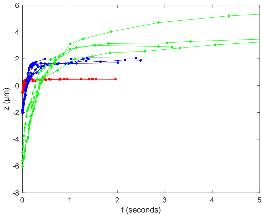
(a) Sulphate latex particles of size 1\ \mu\text{m} (red squares), 4\ \mu\text{m} (blue circles), and 10\ \mu\text{m} (green diamonds) adsorbing to the interface of a 10% / 10% dextran / fish gelatin system.
