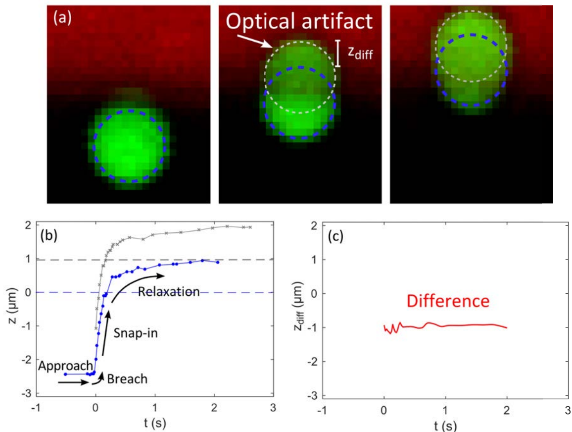
Figure 10.1: Example of confocal microscopy tracking of an adsorption of a 4.5 \mu\text{m} Sulphate latex particle to an 8%/8% dextran / fish gelatin interface. (a) 8 \mu\text{m} \times 10 \mu\text{m} Frames from confocal microscope. Fluorescein-labelled particle shown in green, and the fish-gelatin-rich phase is labelled red with Rhodamine B. Time of images from moment of breach: 0 s, 0.61 s and 1.03 s. In frames 2 and 3, two particle images can be seen, due to a lensing effect elsewhere in the sample. Either image can be tracked. (b): results of particle tracking, z representing the distance of the blue particle centre from the interface. Uncertainty in measurement approximately 0.15 \mu\text{m} . Blue trajectory tracked from lower particle image outlined in blue, grey trajectory upper image outlined in grey. Upper and lower dashed lines correspond to interface positions for upper and lower particles, respectively. (c) Difference, z_{\text{diff}} between upper and lower particle positions from tracking. No trends is observed and noise is the same size as measurement uncertainty. Either image can therefore be tracked.
