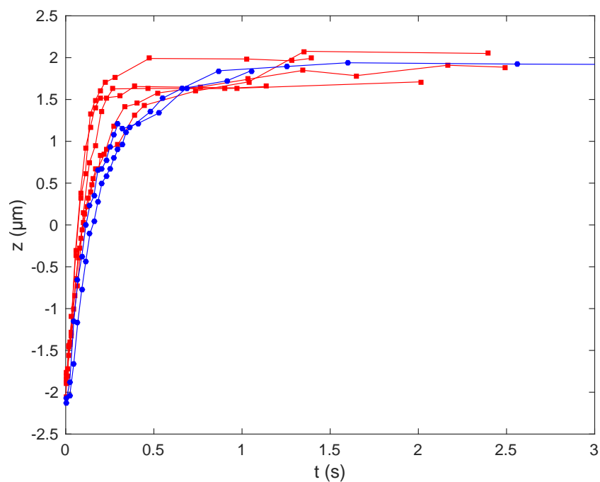
Figure 10.6: Influence of initial phase purity upon adsorption of 4 \mu\text{m} Sulphate latex particles to the dextran-gelatin interface in a 10% / 10% dextran / fish gelatin system. Red squares: pure phases. Blue circles: thermodynamically equilibrated phases. No influence of initial phase purity is seen within experimental errors.
