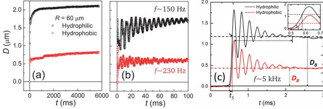
Figure 3.10: Snap-in of a 120 \mu\text{m} diameter particle. Oscillations in (b) caused by activation of capillary waves, whereas those in (c) are due to resonance of the cantilever. Inset shows initial \sim 0.2 ms of the motion, defining the 'snap-in time' t_s . D_B is the cantilever deflection at which the capillary force balances the cantilever spring force.
