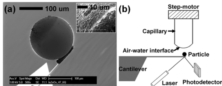
Figure 3.9: From [17]. a) SEM images of a silica glass bead with diameter 172\ \mu\text{m} glued onto a cantilever. Inset is a zoom of the surface. b) Schematic of the AFM particle interaction apparatus. The stepper motor brings the particle into contact with the water droplet, and the deflection of the laser point caused by the bending of the cantilever is measured by the photodetector.
