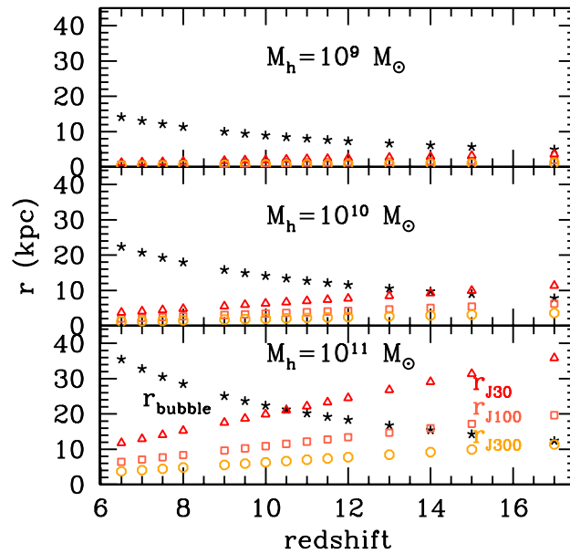
Fig. 5.9 – Metal polluted bubble radius (black stars), and radius of the regions where J_{21,LW} = 30 (red triangle), J_{21,LW} = 100 (orange squares) or J_{21,LW} = 300 (yellow circles) vs redshift for different halo masses ( 10^9, 10^{10}, 10^{11} M_\odot ). All quantities are computed one free-fall time after the star-formation burst. Only regions which are at a distance above the distance given by r_{bubble} , and below the r_{rad} are illuminated by the given radiation intensity and are not polluted by galactic winds. For instance, halos with mass 10^{11} M_\odot at z = 15 can irradiate a nearby halo at a distance of \sim 17 kpc with an intensity J_{21,LW} = 100 without polluting it (the metal bubble has reached only a distance of \sim 14 kpc).
