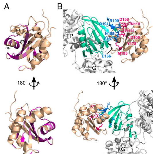
Fig. 3. LpoB interacts with the UB2H domain of PBP1B. (A) Residues showing a significant perturbation upon His-UB2H addition are mapped on the cartoon representation of the LpoB(sol) structure. Residues showing chemical shift perturbations higher than 0.05 ppm are shown in pink, and residues for which the [^1\text{H}, ^{15}\text{N}] correlation showed intensity changes upon interaction are in dark purple ( SI Appendix, Fig. S4C ). (B) Final HADDOCK model of the LpoB–PBP1B complex after addition of ambiguous restraints from NMR perturbations, and biochemical/functional data (Fig. 4). Residues changed to Ala, or reverse-charge amino acids in the activity assays, are represented as sticks in blue (UB2H domain) or magenta (LpoB). Cartoon representation of LpoB and UB2H domain are shown in wheat and green, respectively. Additional domains in PBP1B are shown in gray.
