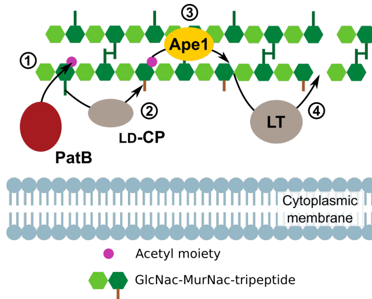
Figure I.3.8: O-deacetylation by Ape proteins is required for peptidoglycan cleavage by lytic transglycosylases. If muero-tetrapeptide are acetylated by PatB (1), a L,D-carboxypeptidase (LD-CP) is required to generate muero-tripeptides (2). The latter mueropeptides are the substrates for the O-acetyl-peptidoglycan esterase Ape1, which can remove their O-acetyl moiety at the position 6 of MurNac (3). This step is essential to enable cleavage of the glycan strand by lytic transglycosylases (4). Adapted from Moynihan & Clarke, 2014b.
