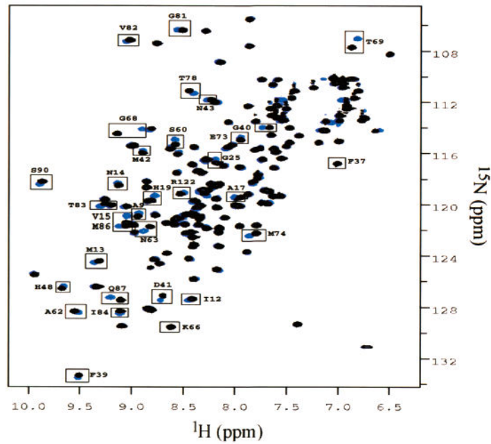
Figure 1.5.13: ^1\text{H} - ^{15}\text{N} HSQC spectra superimposition of ^1\text{H} , ^{15}\text{N} , ^{13}\text{C} ZipA 185-328 (black) and ^1\text{H} , ^{15}\text{N} , ^{13}\text{C} ZipA 185-328 interacting with FtsZ C-terminal peptide (blue). The resonances shifting upon interaction are boxed. Taken from Moy et al., 2000.
