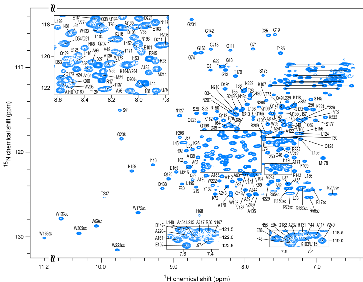
Fig. 1 Fully assigned 2D [ ^1\text{H} , ^{15}\text{N} ]-HSQC spectrum of 2.5 mM LpoA N in 100 mM sodium acetate buffer, pH 4.5, at 323 K. Each backbone amide resonance is labeled with the amino acid type ( one-letter code ) and position in the sequence. Amine groups from
