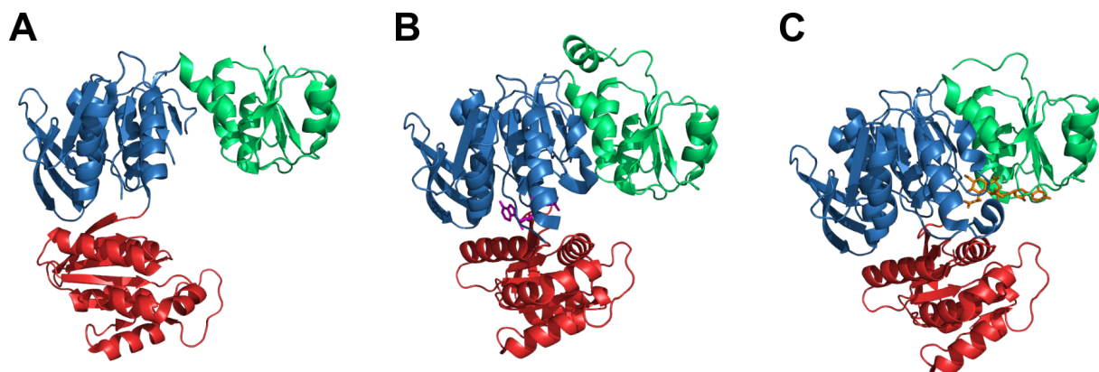
Figure I.2.8: Mur ligases conformations. Mur ligases (here Haemophilus influenzae MurC) can adopt an open conformation (A; PDB code 1GQQ) in the apo-enzyme and a closed conformation induced by ATP (B; PDB code 1GQY) and/or UDP-MurNAc (C; PDB code 1P31) binding. Domains 1, 2 and 3 are colored in green, blue and red respectively. The ATP and UDP-MurNAc substrate mimetics are shown as magenta and orange sticks, respectively.
