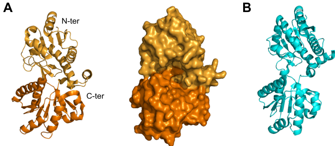
Figure II.2.2: LpoA C-terminal domain is a structural homologue of leucine/valine/isoleucine binding proteins (LVIBP). (A) Cartoon (left) and surface (right) representation of the crystal structure of Haemophilus influenzae C-terminal domain of LpoA (residues 257 – 575, corresponding to residues 257 – 678 in E. coli ; PDB code 3CKM). The two sub-domains are represented in two shades of orange. (B) Structure of LVIBP in an open conformation (PDB code 1Z15).
