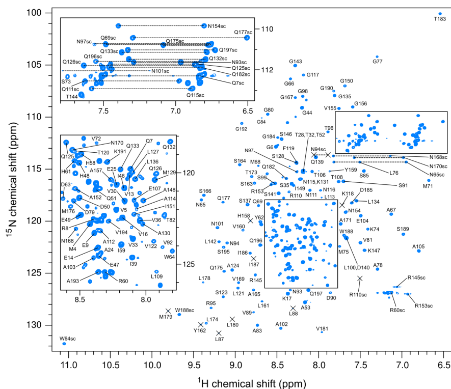
Fig. 1 Fully assigned 2D [ ^1\text{H} , ^{15}\text{N} ]-HSQC spectrum of a 0.8 mM sample of ^{13}\text{C} , ^{15}\text{N} -labeled LpoB in 100 mM sodium acetate buffer, pH 4.5, containing 10 % \text{D}_2\text{O} at 308 K. Each backbone amide resonance is labeled with the amino acid type (one-letter code) and position in the sequence. Amino groups from tryptophan (H \epsilon 1-N \epsilon 1) and arginine (H \epsilon -N \epsilon ) side chains are labeled with "sc". Assigned amide groups from glutamine and asparagine side chains are outlined
