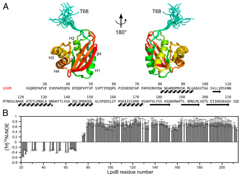
Fig. 2. LpoB structure shows a globular domain with a flexible N-terminal region. (A) Ensemble of the 20 lowest-energy structures of LpoB(sol) (from Thr68 for clarity) determined by NMR spectroscopy (colors from cyan to red are from N to C terminus). The position of \alpha -helices (H1–H4) and \beta -strands ( \beta 1– \beta 4) are indicated on the structure and on the sequence below (helices and arrows). (B) Heteronuclear \{^1\text{H}\} - ^{15}\text{N} -NOE values calculated from the intensity ratio between the saturated and the reference experiments. Errors on the intensity ratio were calculated from the signal-to-noise ratio of the NMR signal in each spectrum. The numbering begins at Val21. High, low, and negative values indicate low, medium, and high flexibility, respectively.
