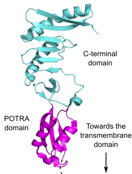
Figure I.4.14: Structure of the periplasmic region of E. coli FtsQ (PDB code 2VH1). The POTRA domain (in magenta), the closest to the cytoplasmic membrane, is required for the FtsQ localization to mid-cell. The C-terminal domain (in light blue) recruits the FtsBL sub-complex.
