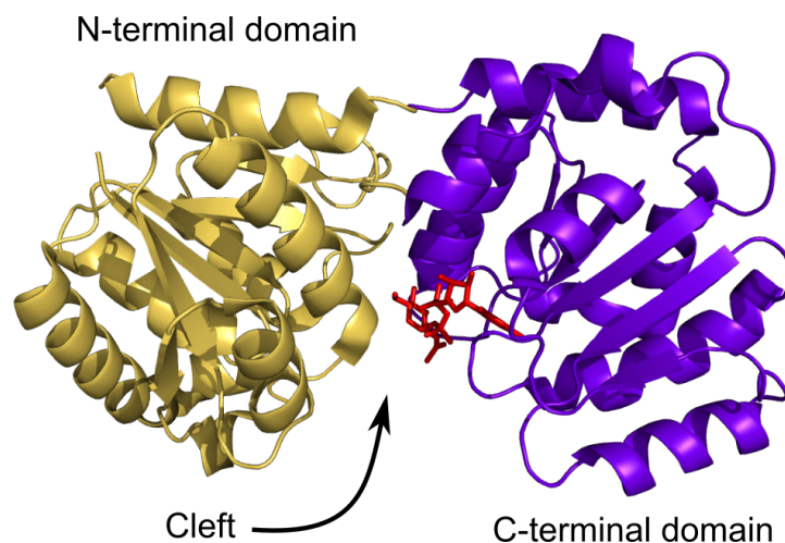
Figure I.2.14: Structure of E. coli MurG (PDB code 1NLM). The UDP-GlcNAc substrate is represented in red sticks. Binding site of the lipid I is located on the other face of the cleft, on the N-terminal domain.
