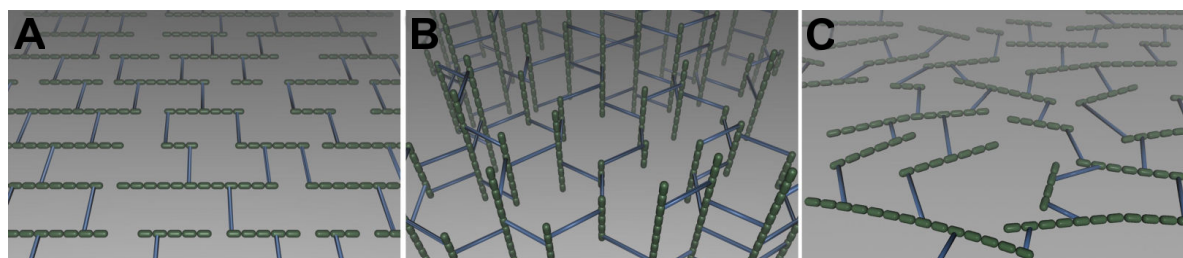
Figure I.1.6: Main models for peptidoglycan organization. (A) The layered-model, (B) the scaffold model. (C) represents a third model derived from the first one, which allows more disorder in the glycan chains positions and is consistent with recent AFM data on E. coli , S. aureus , and S. pneumoniae . Taken from Gan et al., 2008.
