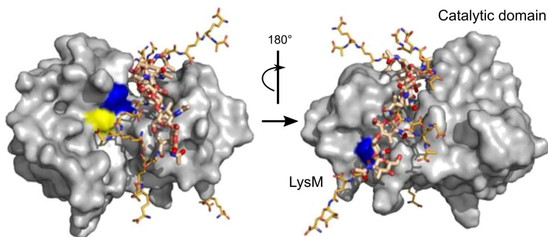
Figure I.5.18: Lowest-energy model generated by HADDOCK for the Ldt Bs -peptidoglycan (hexasaccharide-tetrapeptide) complex. The residues later mutated to prove their implication in the interaction (Val 47 and His 122) are colored in blue while the catalytic cysteine is in yellow. Taken from Schanda et al., 2014.
