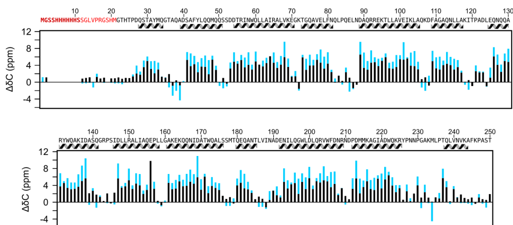
Fig. 2 Amino acid sequence and secondary structure of LpoA N . Residues in red in the sequence correspond to the N-terminal oligo-histidine tag and are irrelevant to wild-type LpoA. The first eleven residues in bold and darker characters in this tag remain mainly unassigned. The secondary structure elements, 13 \alpha -helices represented below the sequence, were predicted using TALOS+ according
