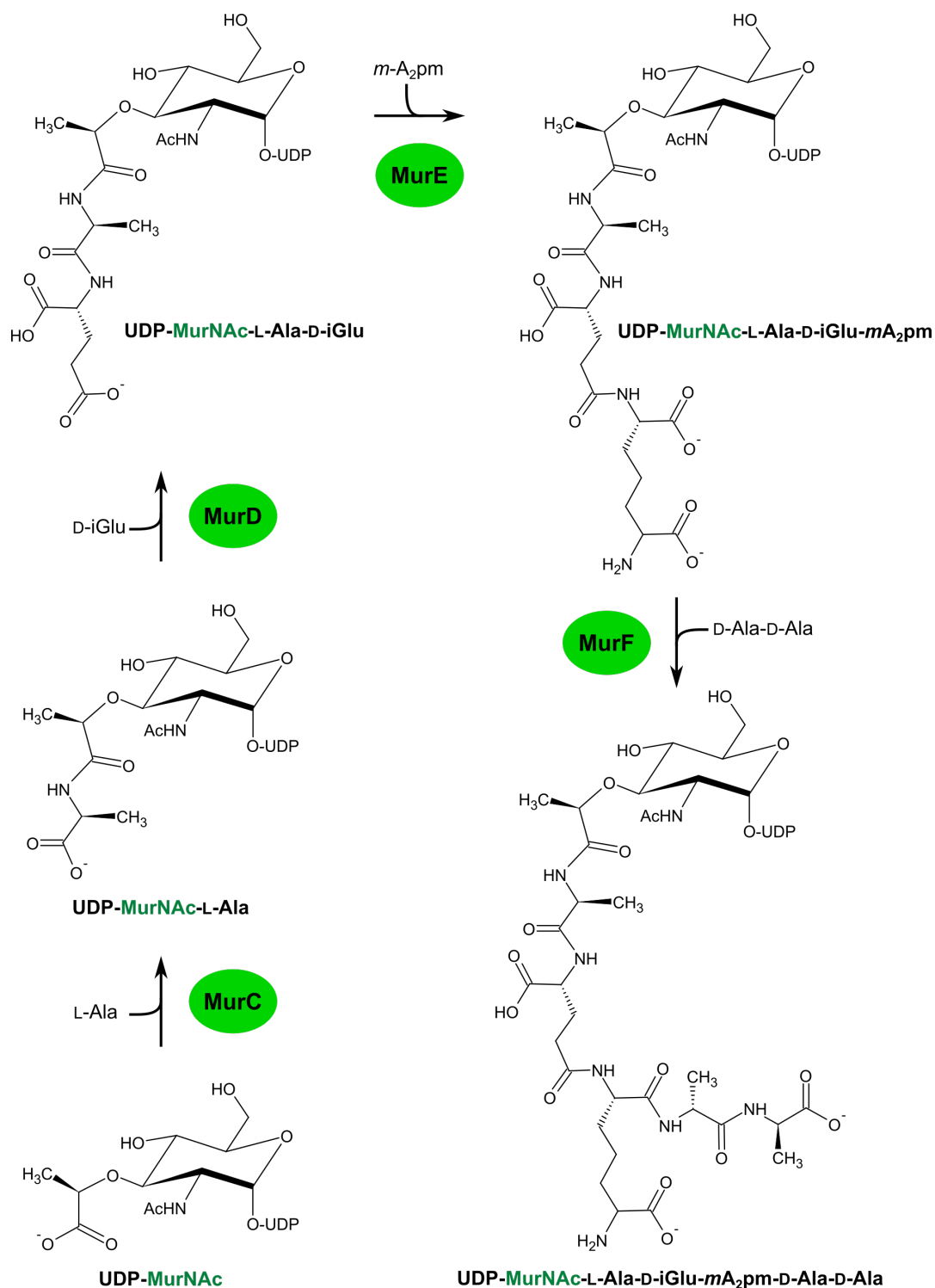
Figure I.2.6: Biosynthesis of UDP-MurNAc-L-Ala-D-iGlu- m A 2 pm-D-Ala-D-Ala from UDP-MurNAc by Mur ligases. The UDP-MurNAc-pentapeptide is synthesized in 4 steps, consisting in the sequential addition of L-Ala, D-Glu, m -A 2 pm (or L-Lys) and D-Ala-D-Ala by MurC, MurD, MurE and MurF, respectively. Adapted from Kouidmi et al., 2014.
