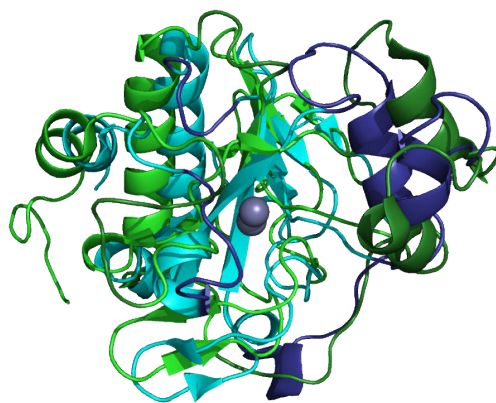
Figure I.5.7: Comparison of Citrobacter freundii AmpD structures solved by NMR (green, PDB code 1J3G) and X-ray crystallography (blue, PDB code 2Y2D). Significant structural modifications are highlighted in dark green and dark blue on their respective structures (mainly in the right region).
