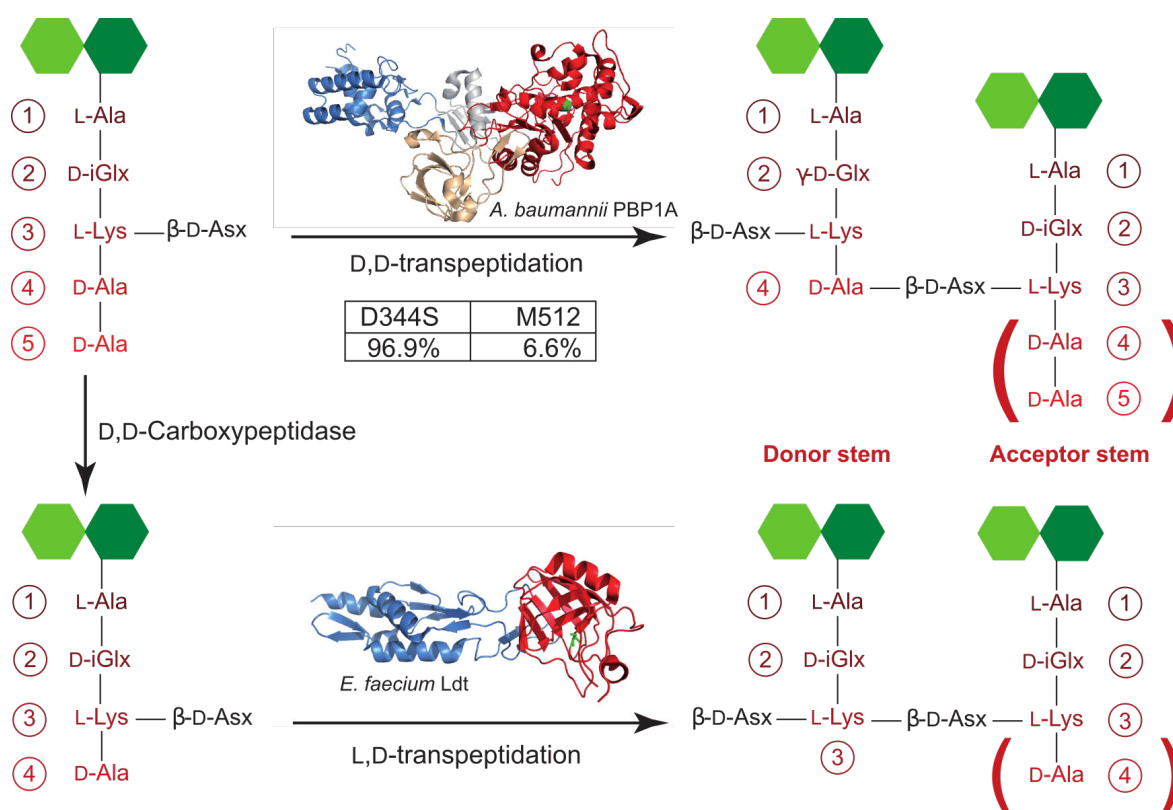
Figure I.1.9: Schematic representation of the 4 → 3 and 3 → 3 cross-links in Enterococcus faecium . The formation of these cross-links is catalyzed by D,D- and L,D-transpeptidase enzymes, respectively. The light and dark green colors represent the GlcNAc and MurNAc saccharides, respectively. Amino acids are indicated in red with their stereochemistry. Cross-links consist in a peptide bond between the amino group of the amino acid in position 3 of the acceptor peptide stem and the carbonyl group of the amino acid in position 3 or 4 of the donor strand. 96.9% of the cross-links are the usual 4 → 3 cross-links in the ampicillin-sensitive E. faecium strain, D344S, while 6.6% only of these cross-links are present in the M512 ampicillin-resistant strain, yielding to a majority of 3 → 3 cross-links in this strain (Mainardi et al., 2002).
