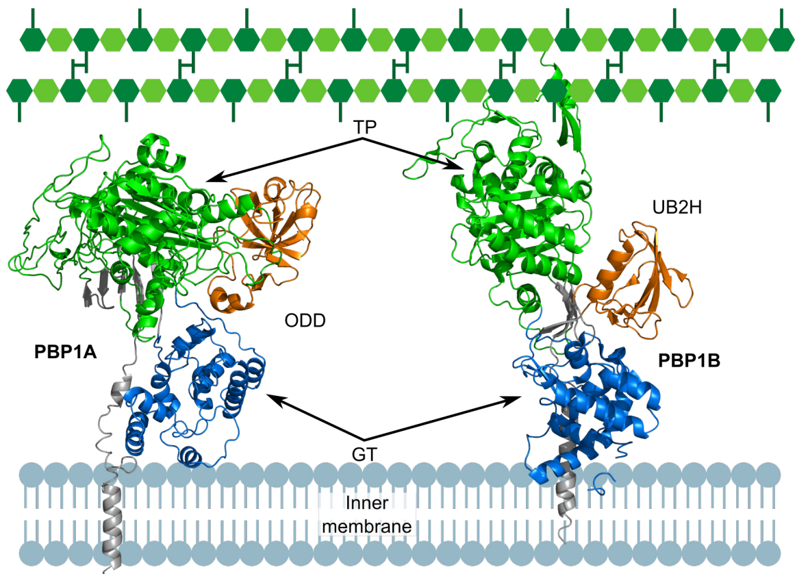
Figure I.2.16: Structural organization of the two E. coli main bifunctional PBP1s: PBP1A (model generated by Phyre2), and PBP1B (PDB code 3VMA). The transpeptidase (TP), glycosyltransferase (GT) and non-catalytic domains (ODD and UB2H for PBP1A and PBP1B, respectively) are colored in green, blue, and orange respectively. The transmembrane \alpha -helix and the \beta -sheet linking these domains are in gray. Note that the relative position of the TP compared to the GT domain in the modeled PBP1A may be different in the real structure.
