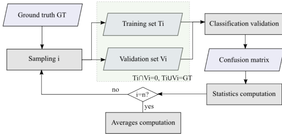
Figure 4.6: Illustration of the validation procedure
