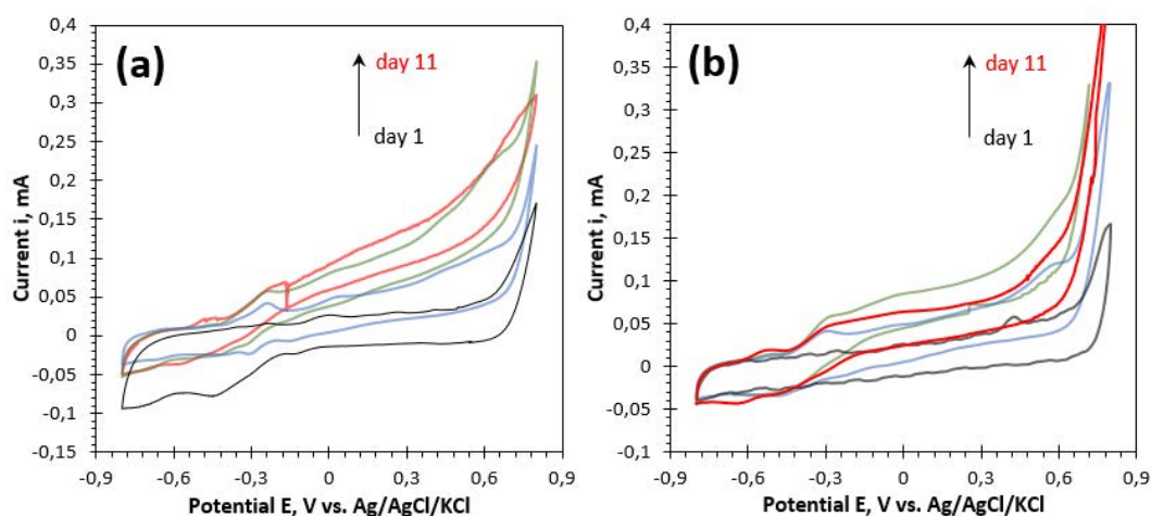
Figure 2.26 – Effect of the presence or absence of oxygen in solution during the incubation of a 1 cm 3 carbon felt under polarization ( E_{working} = +0.3 V ) in a sealed or open to air single-compartment. Bacteria are sample at an OD_{600} = 2.1 , transferred in MR1 medium supplemented with lactate at 30 mM and diluted or centered to an OD_{600} = 0.6-0.7 . The Mediated Electron Transfer occurs between -0.4 and 0 V vs. Ag/AgCl/KCl and the Direct Electron Transfer occurs between 0 and 0.8 V vs. Ag/AgCl/KCl.
