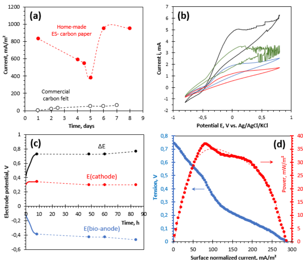
Figure 3.21 – Electrochemical characterization of a dual-compartment reactor based on the use of: a ES-carbonpaper (electrospinning of a 10 w.% PAN solution stabilized at 220°C and carbonized at 940°C, \sigma_T = 5 \text{ mS} \cdot \text{m}^{-1} and \sigma_p = 3.4 \text{ mS} \cdot \text{m}^{-1} ) as anode and a 2 \text{ cm}^3 carbon felt as cathode. The anolyte consists in a solution of S. oneidensis sampled in log-phase ( \text{OD}_{600} = 1.7 ) diluted in an MR1-L medium at \text{OD}_{600} = 0.7 . The catholyte is a 150 mM NaCl supplemented in 10 mM \text{K}_3\text{Fe}(\text{CN})_6 . A Nafion® membrane is used as a separator. Both anodic and cathodic sides are aerated with vent-cap. The system is not polarized. (a) Comparison between the anodic current provided by an ES-carbon paper at 0.3 V vs. Ag/AgCl/KCl in comparison with a standard 1 \text{ cm}^3 carbon felt in the same condition of measurement and incubation (Current normalized by the geometric surface area). (b) Cyclic voltammometry monitoring of the system at: — day 1, — day 4, — day 5, — day 7. (c) OCP monitoring of: • the anode, • the cathode and • the MFC OCV as function of the time (continuous line = continuous measurement). (d) Characterization of the whole MFC at day 3: • Polarization curve, • Power curve (current and power normalized by the geometric surface area).
