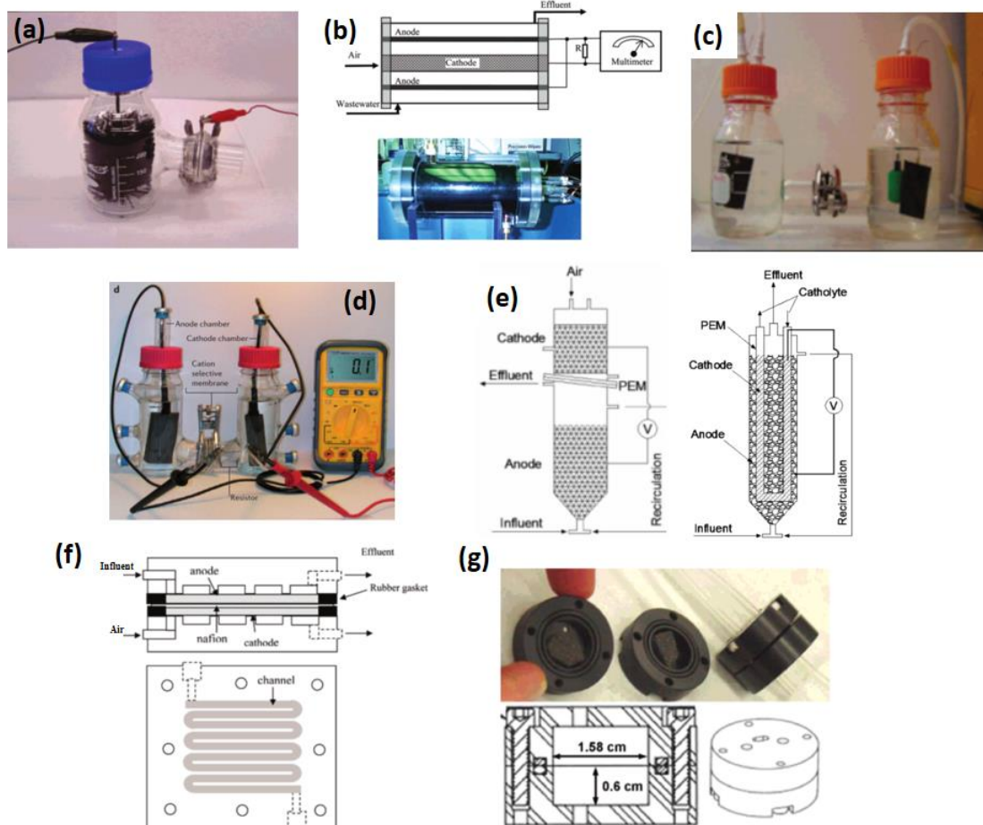
Figure 1.25 – MFC architectures: (a) Single-chamber air-cathode bottle [131], (b) horizontal tubular single-chamber air-cathode [50], H-type architectures (c) gas sparging (Figure 1.22.c) [191], (d) anaerobic condition [192], (e) Cylindrical/tubular [194,195], (f) Planar architecture [193], (g) Micro fuel cell [196]
